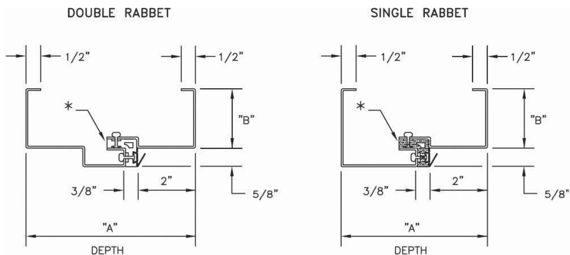
FIGURE 8.32 Thermal Break Hollow Metal Frame (Source: Courtesy of Ceco Door)
