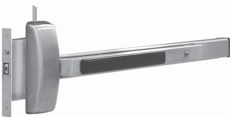
FIGURE 2.96 Concealed Two-Point Lockset (Source: Courtesy of SARGENT® Manufacturing Company)
