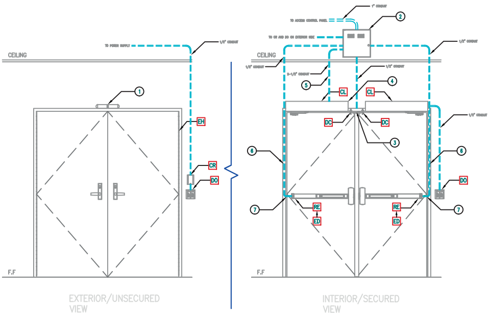
FIGURE 10.2 Elevation Drawing (Source: Courtesy of copyright © 2002–2013, Securitron Magnalock Corporation, an ASSA ABLOY Group Company)
