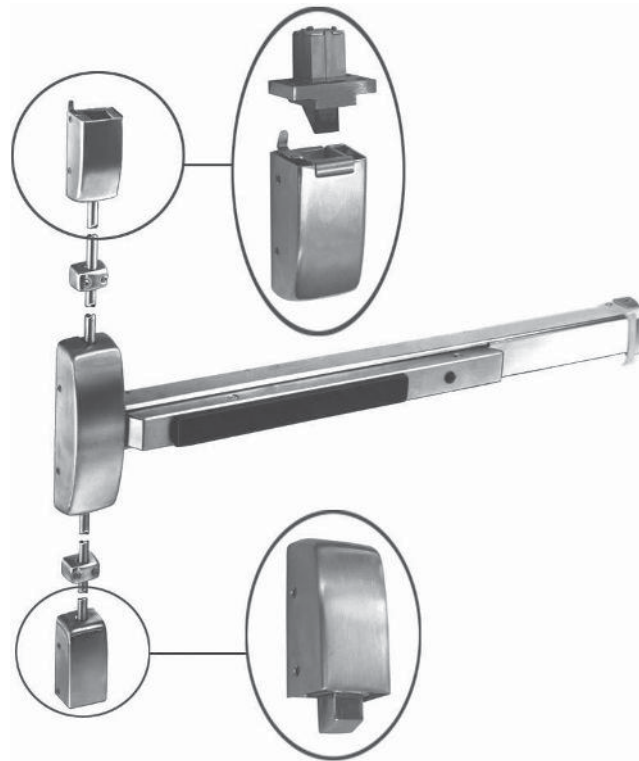
FIGURE 2.90 Windstorm Rated Surface Vertical Rod Exit Device and Latches (Source: Courtesy of SARGENT® Manufacturing Company)
