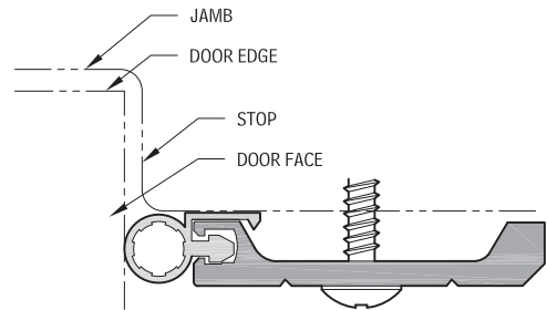
FIGURE 8.16 Heavy-Duty Surface-Mounted Perimeter Seal Housing
