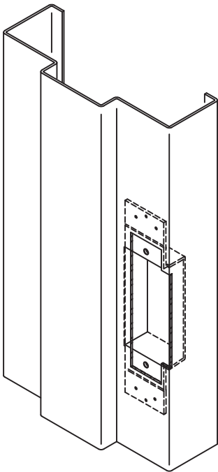
FIGURE 2.181 Mortise Strike Preparations on Door Frame (Source: Courtesy of Ceco Door)
