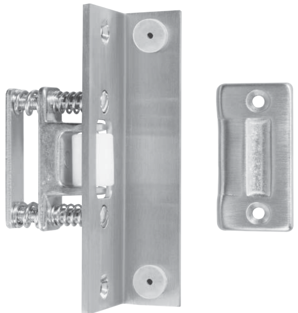
FIGURE 9.34 Roller Latch with Angle Stop (Source: Courtesy of Rockwood® Manufacturing Company)
