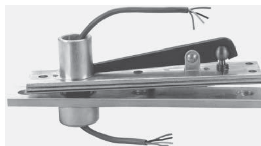
FIGURE 1.103 Electric Transfer Center Top Pivot (Source: Courtesy of Rixson®)
