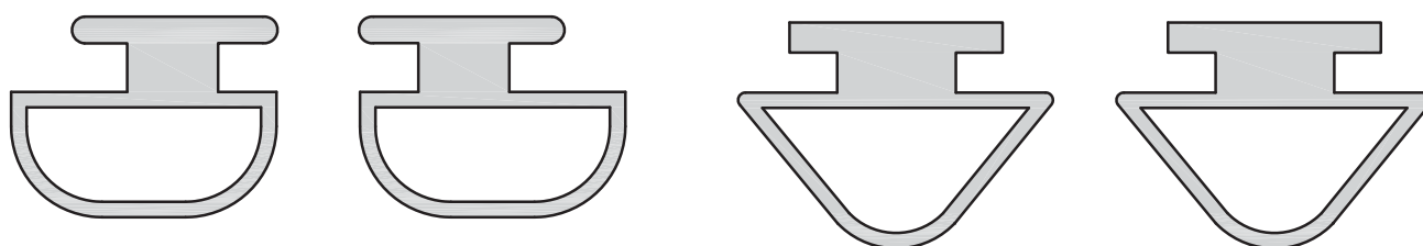
FIGURE 8.30 Alternate Insert Materials and Shapes (Source: Courtesy of Pemko Manufacturing Company)
