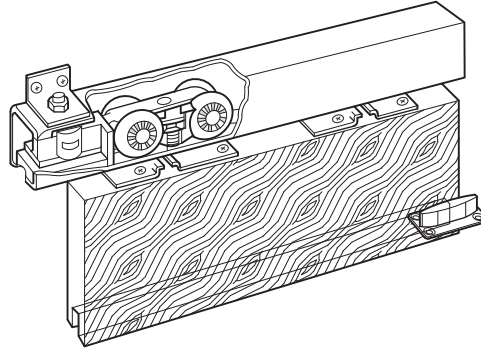
FIGURE 1.109 Sliding Door Hardware
