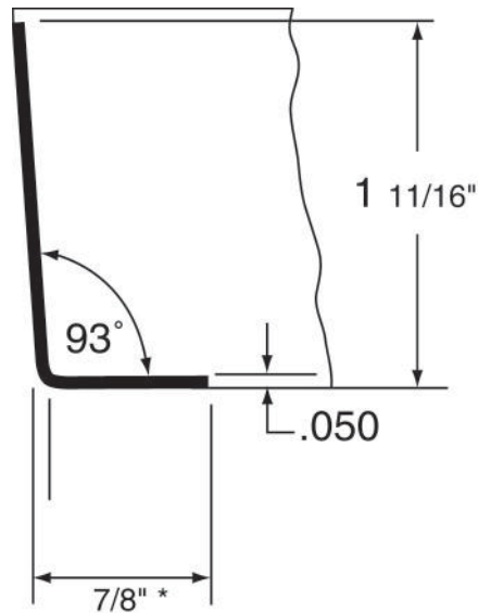
FIGURE 6.4 Door Edge Guard Beveled Angle (Source: Courtesy of Rockwood® Manufacturing Company)
