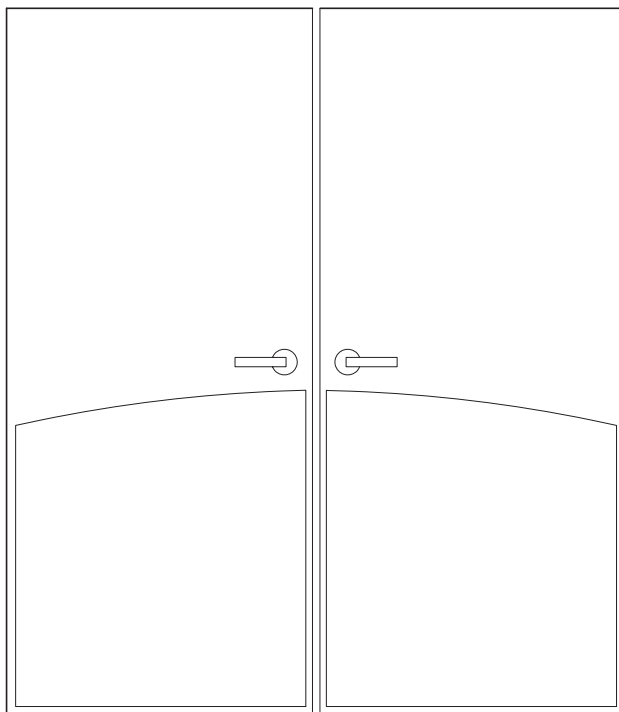
FIGURE 6.17 Decorative Protection Plate (Source: Courtesy of Rockwood® Manufacturing Company)
