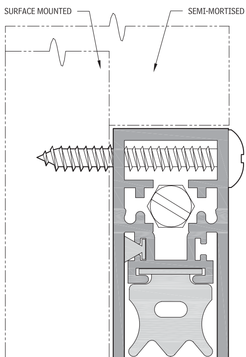
FIGURE 8.26 Surface-Mounted Automatic Door Bottom
