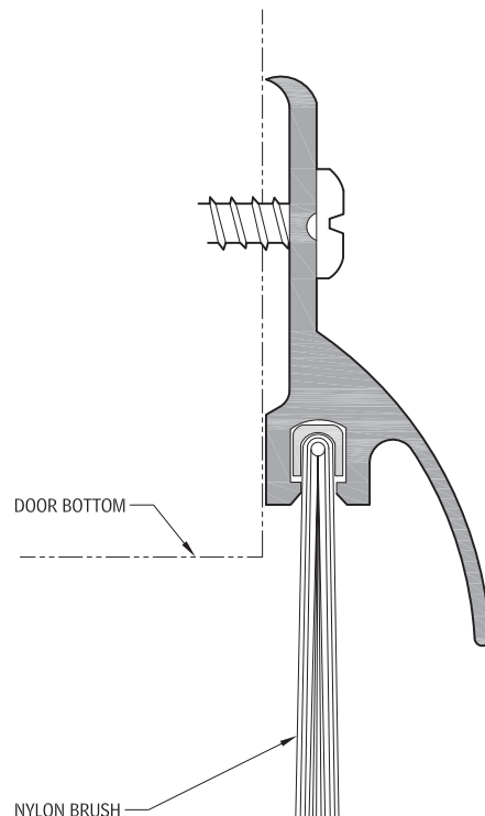
FIGURE 8.22 Surface-Mounted Door Sweep Brush in Housing (Source: Courtesy of Pemko Manufacturing Company)
