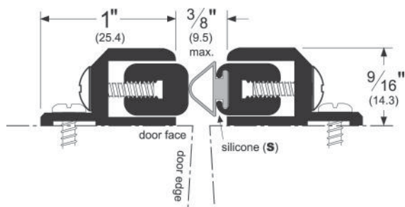
FIGURE 8.1 Adjustable Split Astragal (Source: Courtesy of Pemko Manufacturing Company)
