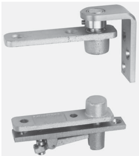
FIGURE 1.81 Standard Duty Center Pivot Set
