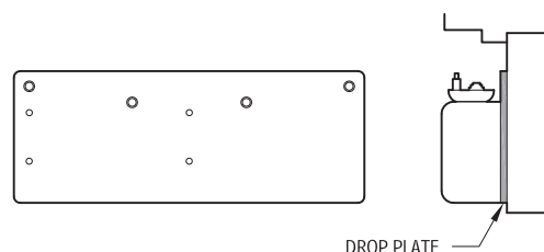
FIGURE 5.8 Narrow Top Rail Surface Door Closer Mounting Bracket
