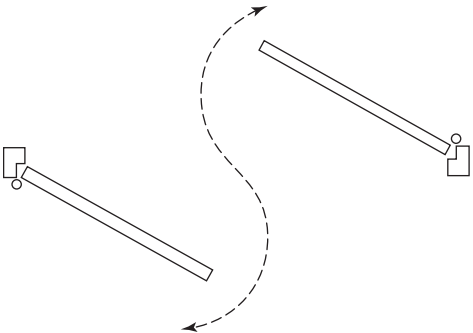
FIGURE 2.62 Surface Vertical Rod Exit Device Strike (Source: Courtesy of SARGENT® Manufacturing Company)
