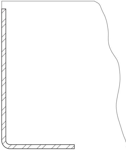
FIGURE 6.3 Door Edge Guard Square Angle (Source: Courtesy of Rockwood® Manufacturing Company)
