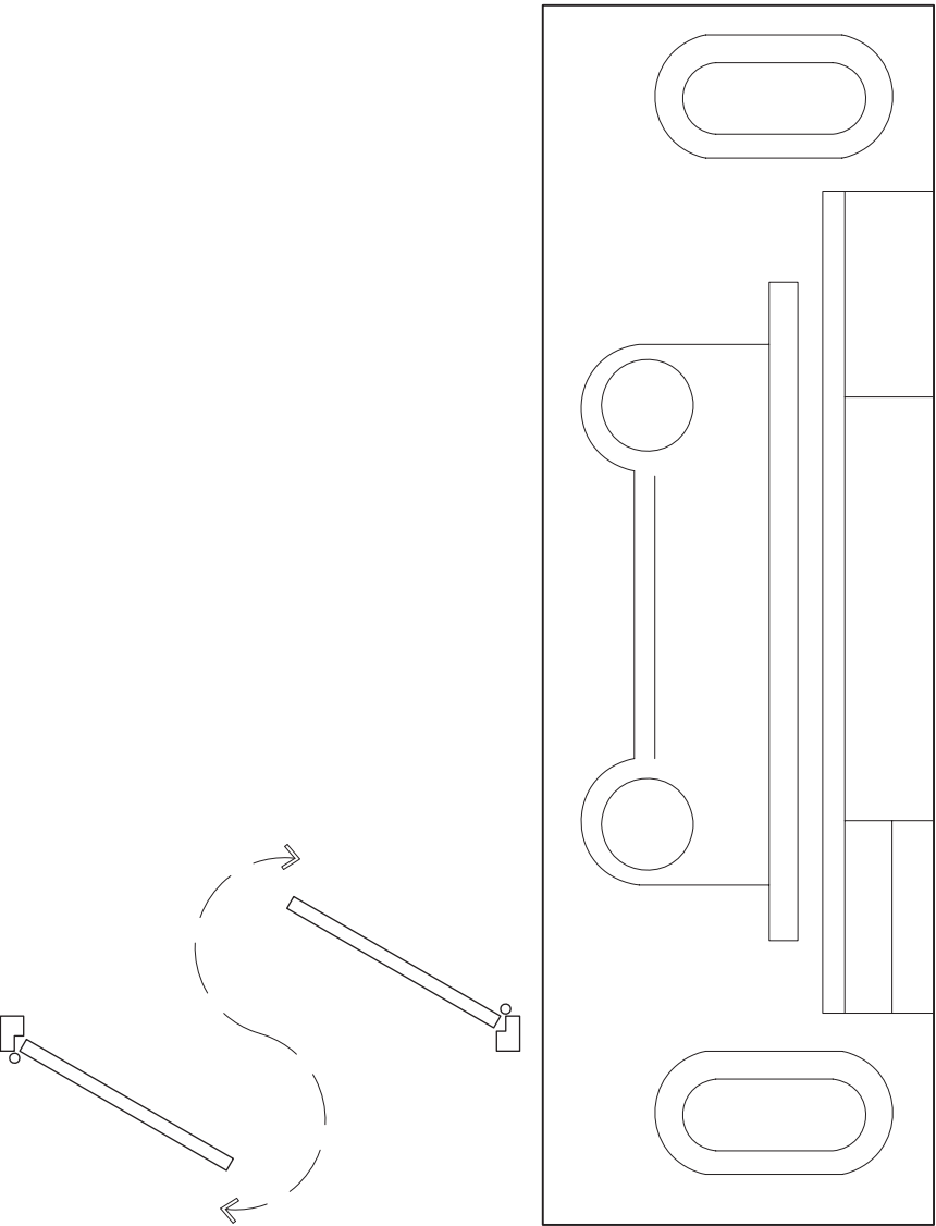
FIGURE 2.60 Rim Exit Device Strike (Source: Courtesy of SARGENT® Manufacturing Company)
