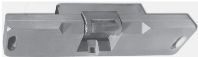
FIGURE 2.45 Electric Strike for Vertical Rod Exit Device (Source: Courtesy of copyright © 2002–2013, Securitron Magnalock Corporation, an ASSA ABLOY Group Company)
