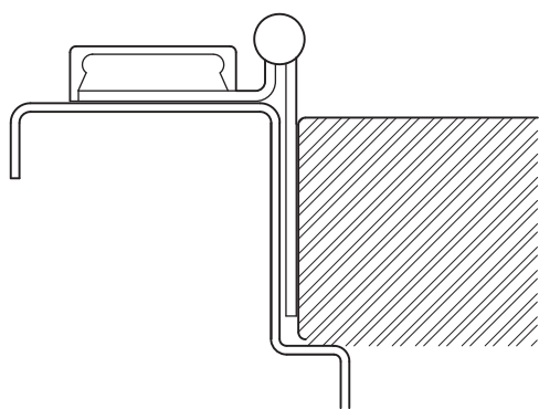
FIGURE 1.79 Half Mortise Continuous Hinge (Source: Courtesy of Markar Architectural Products)
