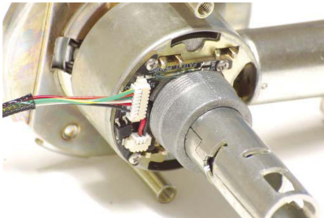
FIGURE 2.171 Electrified Bored Lockset Chassis (Source: Courtesy of SARGENT® Manufacturing Company)
