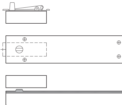
FIGURE 1.108 Patch Fitting Floor Closer
