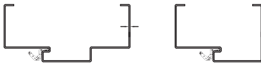
FIGURE 8.31a Kerf Hollow Metal Door Frame (Source: Courtesy of Ceco Door)
