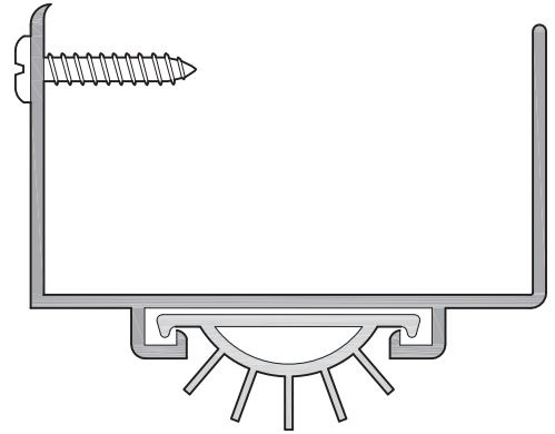
FIGURE 8.24 Surface-Mounted Full Door Shoe (Source: Courtesy of Pemko Manufacturing Company)
