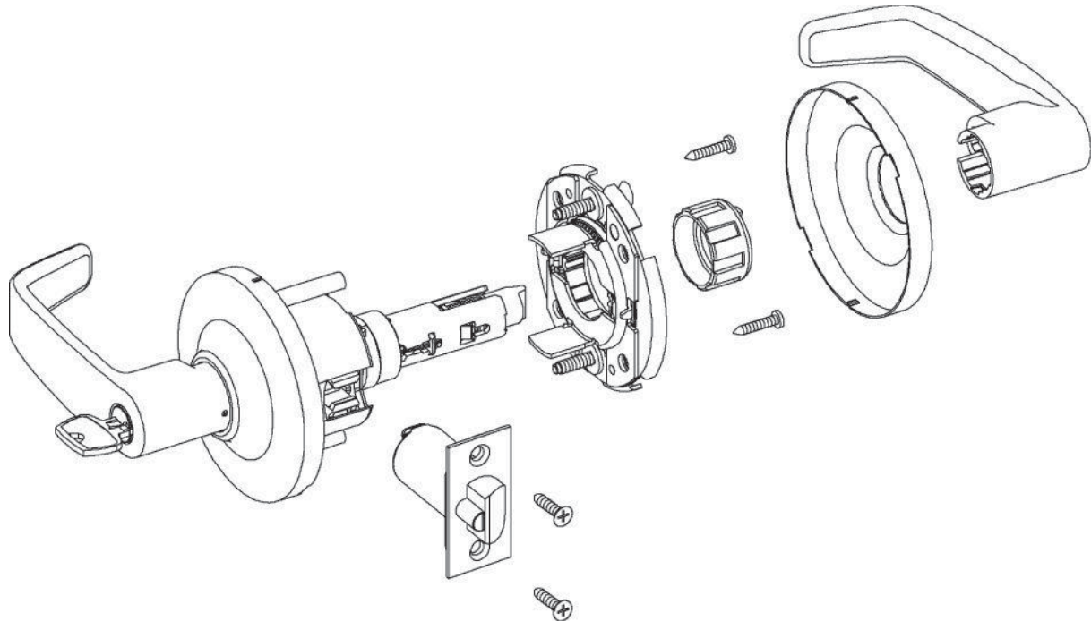
FIGURE 2.130 Bored Lockset Diagram (Source: Courtesy of SARGENT® Manufacturing Company)
