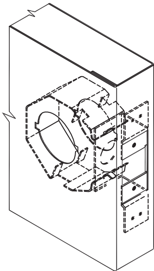
FIGURE 2.182 Bored Lockset Preparations on Door (Source: Courtesy of Ceco Door)
