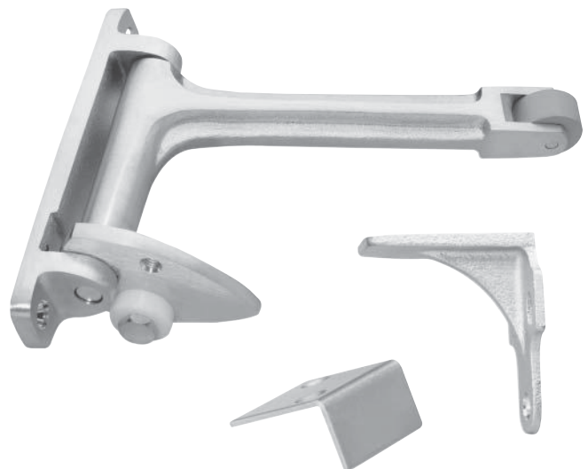
FIGURE 4.2 Gravity Door Coordinator (Source: Courtesy of Rockwood® Manufacturing Company)
