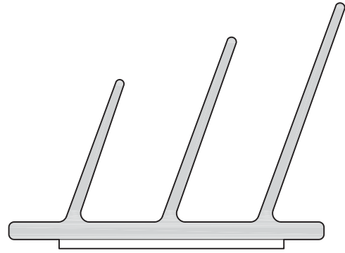
FIGURE 8.20 Surface-Mounted Triple Fin Adhesive Perimeter Seal (Source: Courtesy of Pemko Manufacturing Company)
