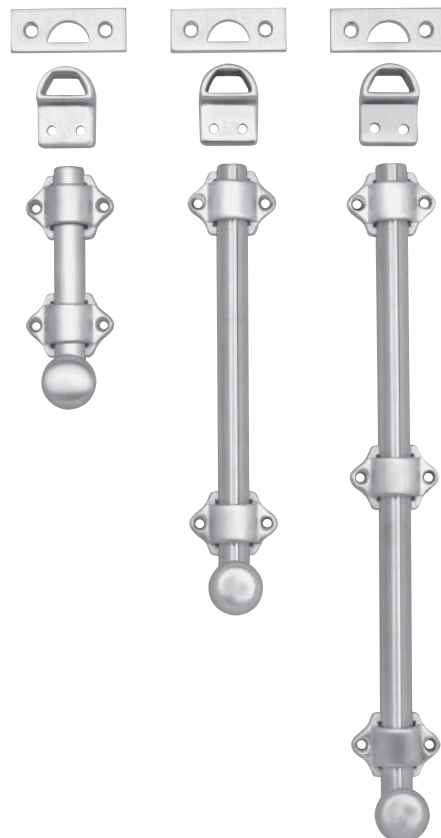
FIGURE 2.3 Dutch Door Bolts (Source: Courtesy of Rockwood® Manufacturing Company)
