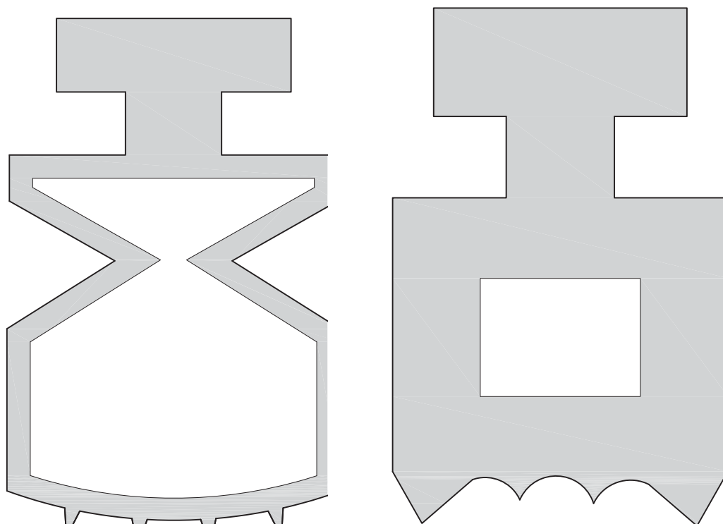
FIGURE 8.29 Alternate Insert Materials and Shapes (Source: Courtesy of Pemko Manufacturing Company)
