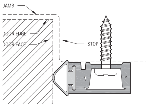
FIGURE 8.17 Surface-Mounted Perimeter Seal in Housing with Cover
