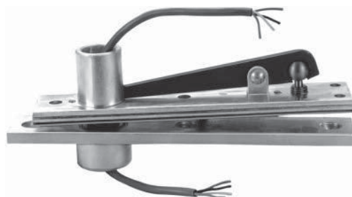
FIGURE 1.88 Electric Transfer Center Top Pivot (Source: Courtesy of Rixson®)
