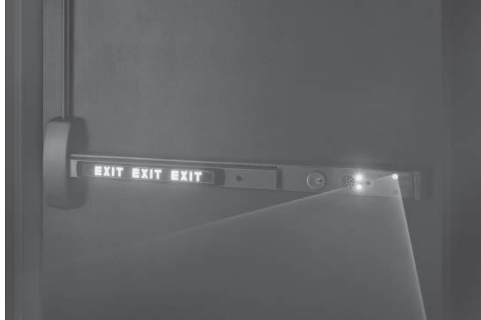
FIGURE 2.75 Wayfinding Device (Source: Courtesy of SARGENT Manufacturing Company)
