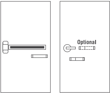
FIGURE 9.22 Door Guard Installed Closed (Source: Courtesy of Rockwood® Manufacturing Company)
