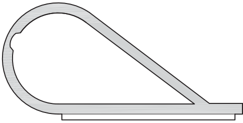
FIGURE 8.19 Surface-Mounted Bulb Adhesive Perimeter Seal (Source: Courtesy of Pemko Manufacturing Company)
