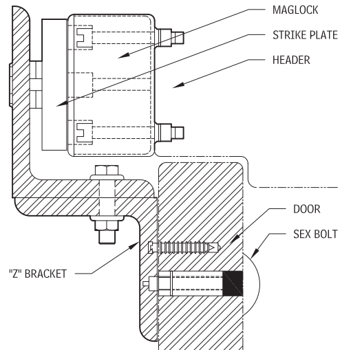
FIGURE 2.110 Z-Bracket Diagram
