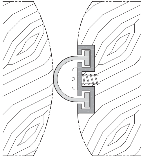
FIGURE 8.5 Recessed Meeting Stile Astragal (Source: Courtesy of Pemko Manufacturing Company)
