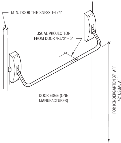
FIGURE 2.48 Crossbar Exit Device (Source: The Graphic Standards Guide to Architectural Finishes , John Wiley & Sons, Inc.)
