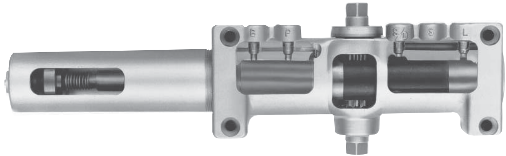
FIGURE 5.1 Surface-Mounted Door Closer Body (Source: Courtesy of Norton® Door Controls)
