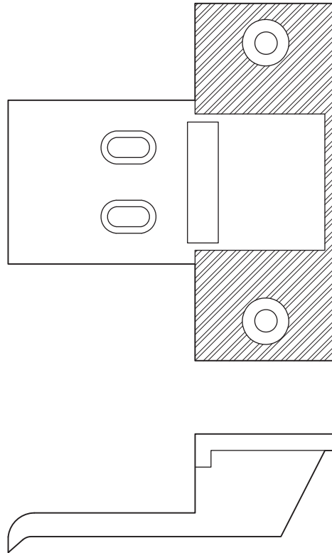
FIGURE 2.58 Rim Exit Device Strike (Source: Courtesy of SARGENT® Manufacturing Company)
