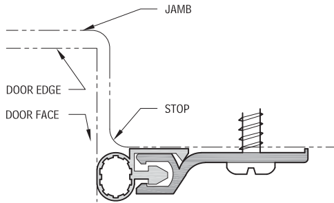
FIGURE 8.15 Surface-Mounted Perimeter Seal in Housing
