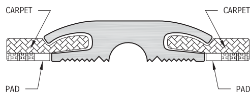
FIGURE 8.14 Residential Vinyl Threshold
