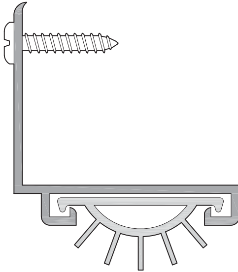
FIGURE 8.23 Surface-Mounted Half-Door Shoe (Source: Courtesy of Pemko Manufacturing Company)
