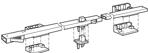
FIGURE 4.1 Bar Door Coordinator (Source: Courtesy of Rockwood® Manufacturing Company)
