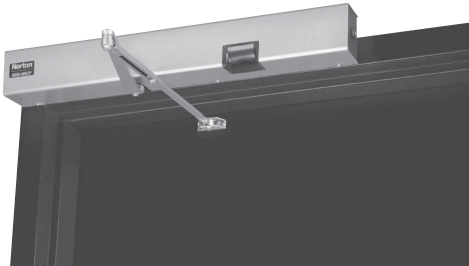
FIGURE 5.12 Electronic Motion Sensor Hold Open Door Closer (Source: Courtesy of Norton® Door Controls)
