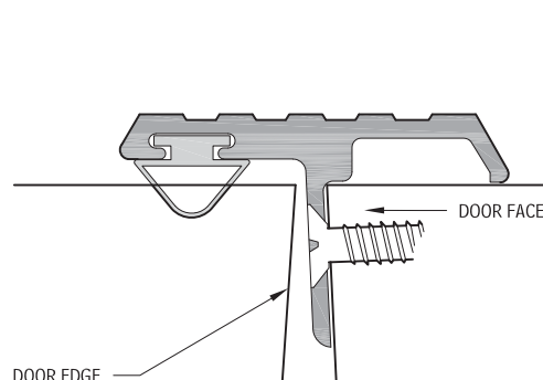
FIGURE 8.3 Overlapping Tee Astragal (Source: Courtesy of Pemko Manufacturing Company)
