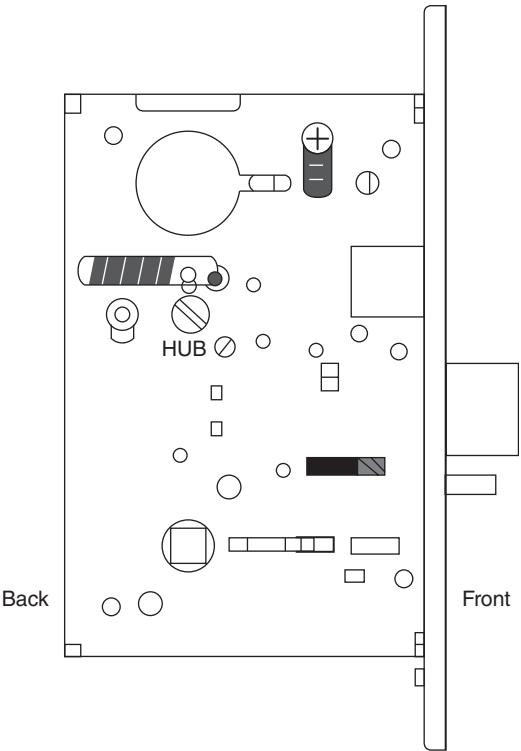
FIGURE 2.136 Mortise Lockset Diagram (Source: Courtesy of SARGENT® Manufacturing Company)
