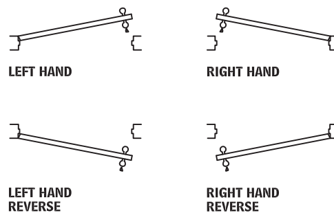
FIGURE 2.78 Door-Handing Chart
