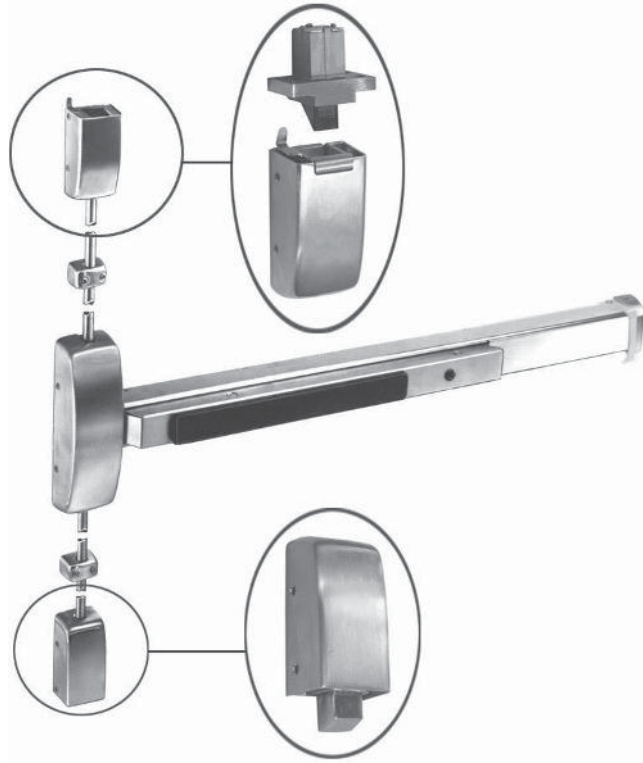
FIGURE 2.99 Hurricane Rated Exit Device and Latches. (Source: Courtesy of SARGENT® Manufacturing Company)
