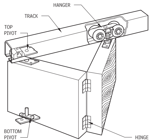
FIGURE 1.119 Bi-Folding Door Hardware
