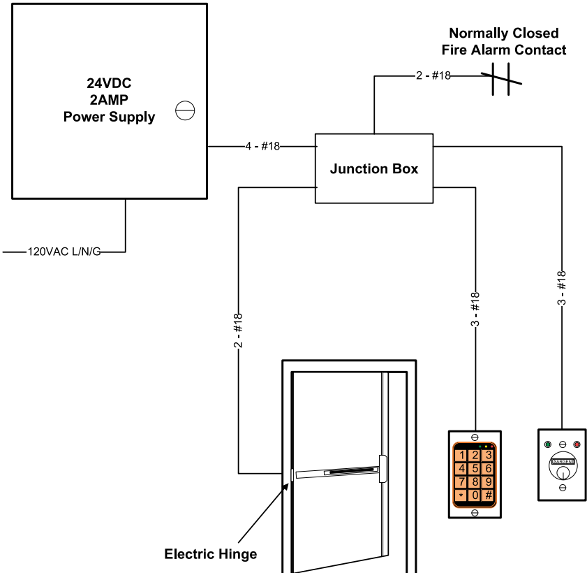
FIGURE 10.1 Elevation Drawing (continues) (Source: Courtesy of copyright © 2002–2013, Securitron Magnalock Corporation, an ASSA ABLOY Group Company)
