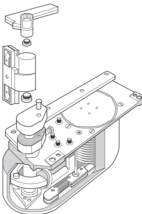
FIGURE 5.7 Floor-Mounted Door Closer (Source: Courtesy of Rixson®)
