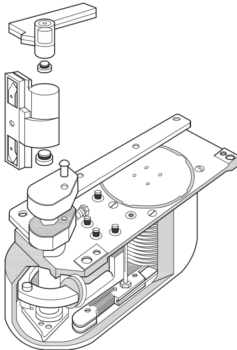
FIGURE 1.99 Heavy Duty Floor Closer
