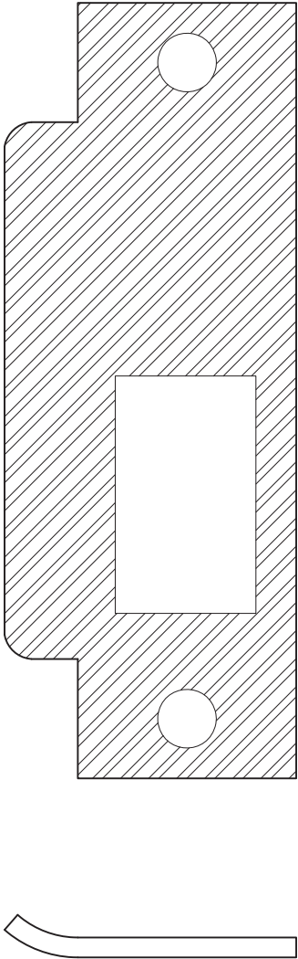
FIGURE 2.61 Mortise Exit Device Strike (Source: Courtesy of SARGENT® Manufacturing Company)
