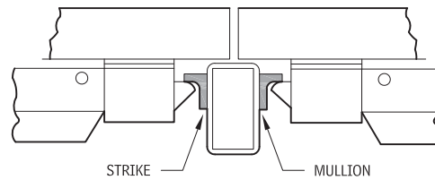
FIGURE 2.91 Rectangular Removable Mullion
