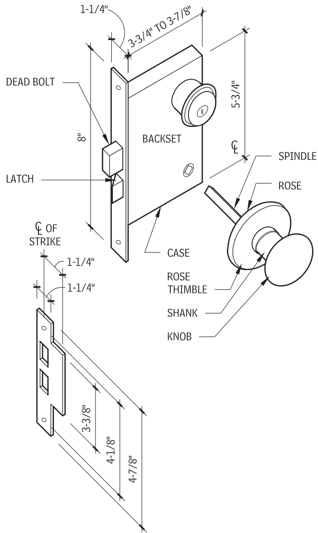
FIGURE 2.177 Mortise Lock
