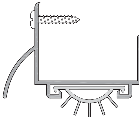
FIGURE 8.25 Door Shoe with Drip Cap (Source: Courtesy of Pemko Manufacturing Company)
