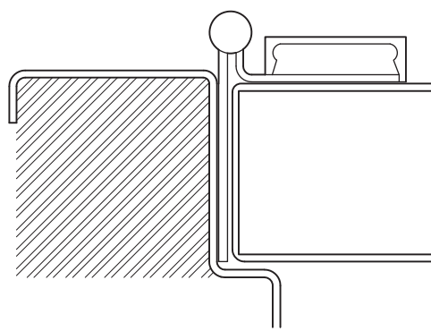
FIGURE 1.80 Half Surface Continuous Hinge (Source: Courtesy of Markar Architectural Products)
