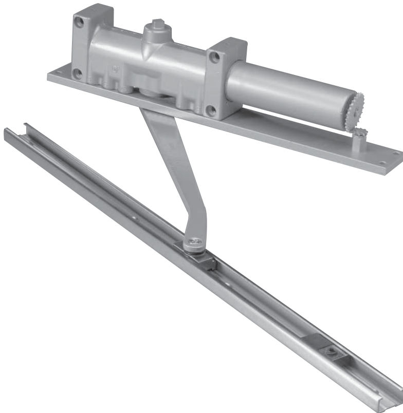
FIGURE 5.6 Concealed in the Frame Door Closer (Source: Courtesy of Norton® Door Controls)
