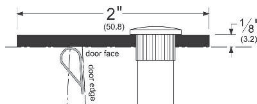
FIGURE 8.2 Overlapping Astragal (Source: Courtesy of Pemko Manufacturing Company)
