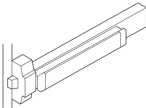
FIGURE 2.50 Crossbar Exit Device (Source: The Graphic Standards Guide to Architectural Finishes , John Wiley & Sons, Inc.)
