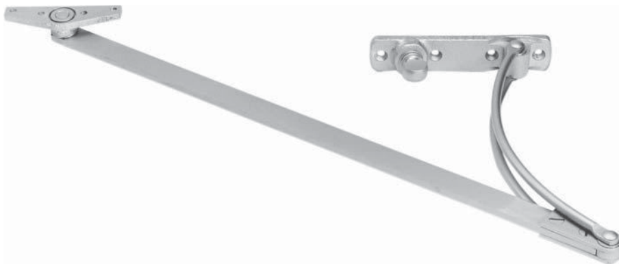
FIGURE 5.21 Cantilever Arm Overhead Stop
