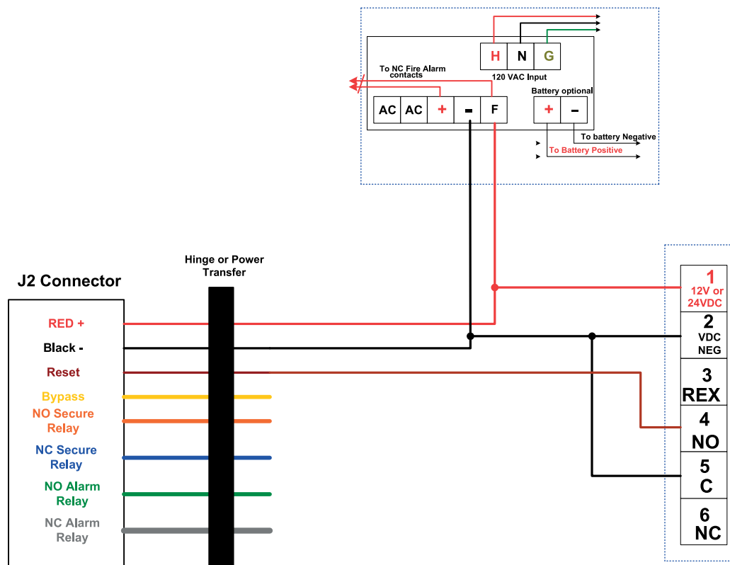
FIGURE 10.3 Point-to-Point Diagram
