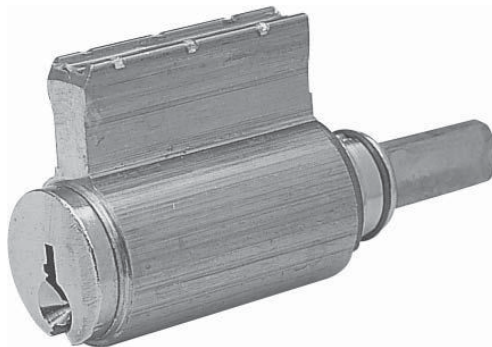
FIGURE 2.33 Key in Lever Cylinder (Source: Courtesy of SARGENT® Manufacturing Company)
