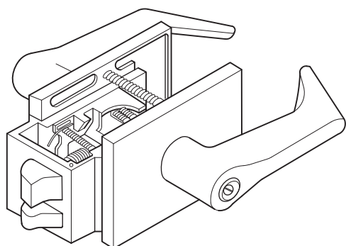
FIGURE 2.142 Preassembled Lockset Diagram (Source: Corbin Russwin®, Inc.)
