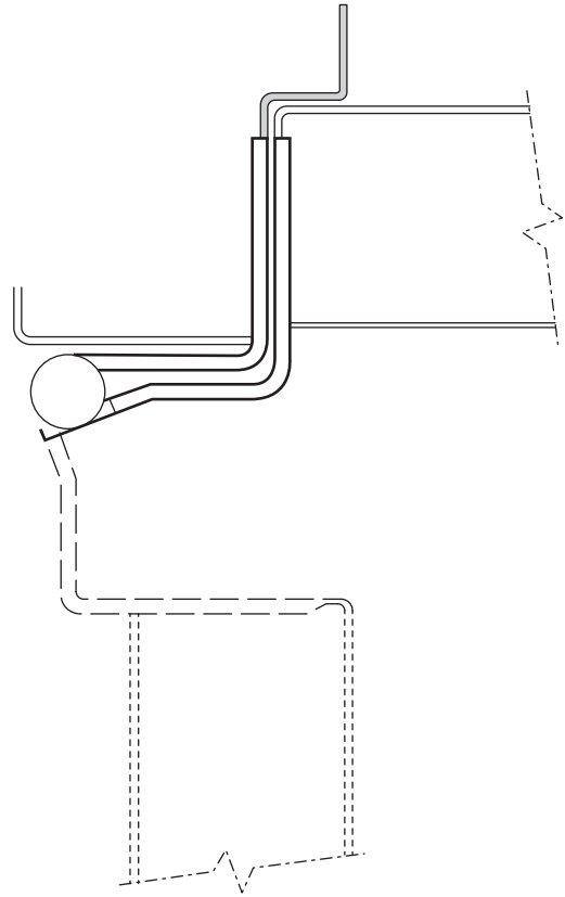
FIGURE 1.70 Swing-Clear Continuous Hinge (Source: Copyright © ASSA ABLOY, Inc. All rights reserved.)
