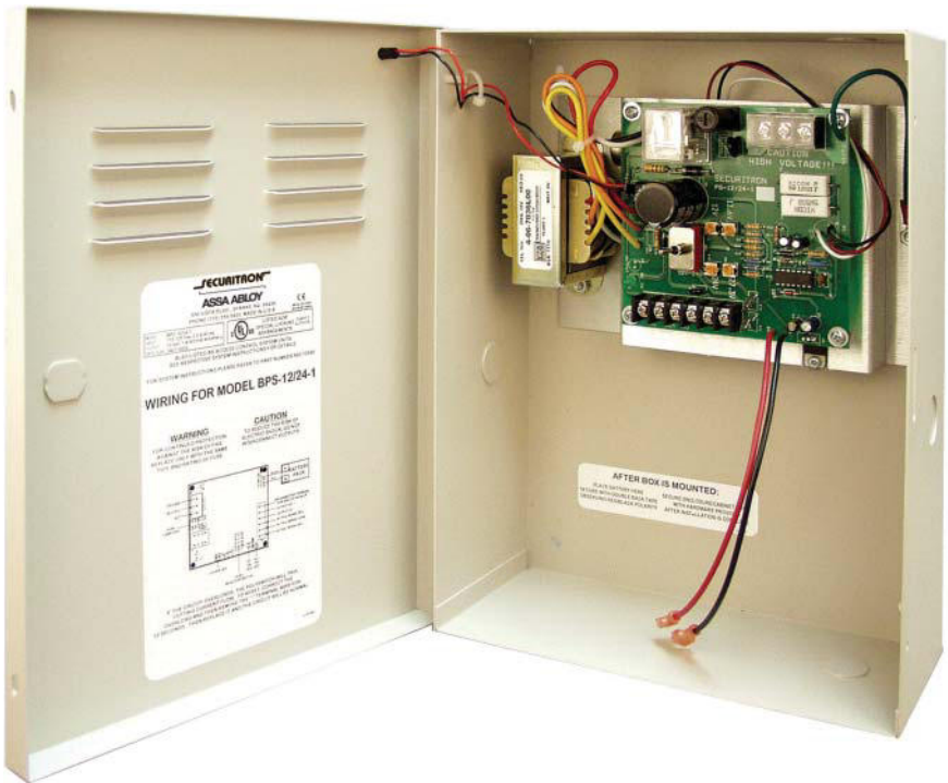
FIGURE 10.8 Power Supply (Source: Courtesy of copyright © 2002–2013, Securitron Magnalock Corporation, an ASSA ABLOY Group Company)
