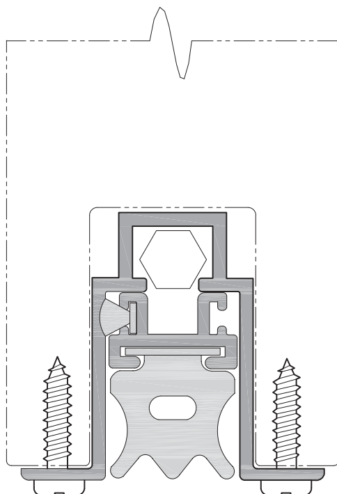
FIGURE 8.27 Concealed or Mortised Automatic Door Bottom
