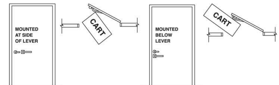
FIGURE 9.21 Door Guard Installed Open (Source: Courtesy of Rockwood® Manufacturing Company)
