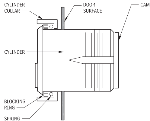
FIGURE 2.25 Cylinder Illustration
