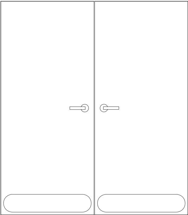
FIGURE 6.13 Decorative Protection Plate (Source: Courtesy of Rockwood® Manufacturing Company)
