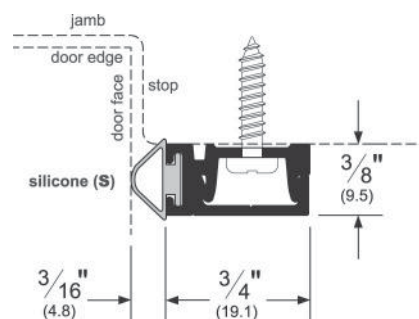
FIGURE 8.4 Snap Cover Astragal (Source: Courtesy of Pemko Manufacturing Company)
