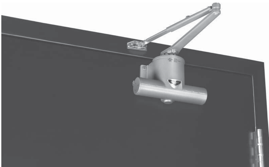
FIGURE 5.3 Pot Belly Surface-Mounted Door Closer (Source: Courtesy of Norton® Door Controls)
