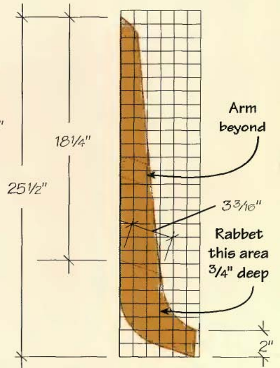
BACK SUPPORT
