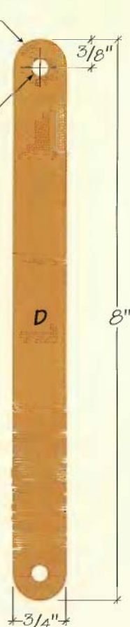
FRONT VIEW BASE STRIPS
