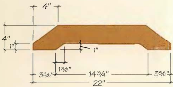
FOOT LAYOUT
