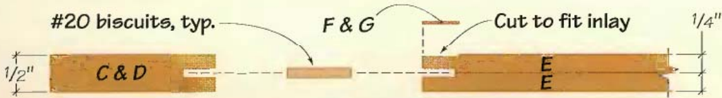
DETAIL: BOTTOMS, FRAMES & INLAYS
