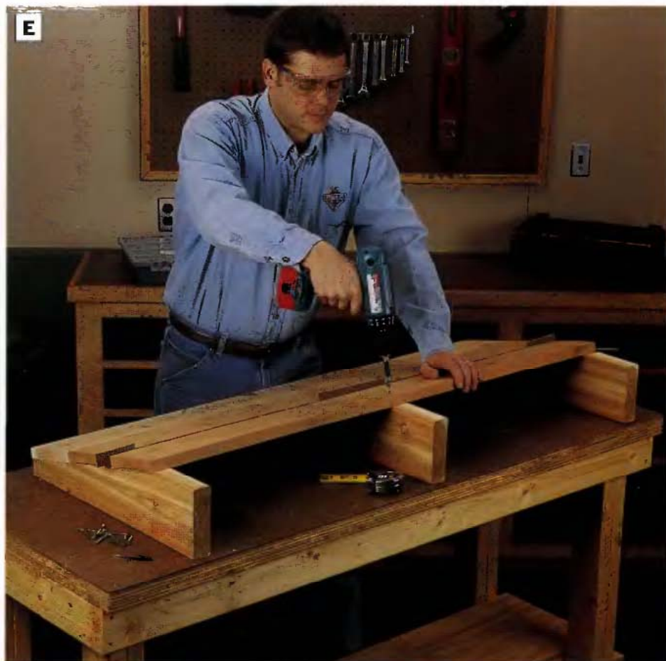
PHOTO E: Attach the back slats along the angled edges of the back supports with screws. Use \frac{1}{4} -in. spacers between the back slats to hold the slats apart.
