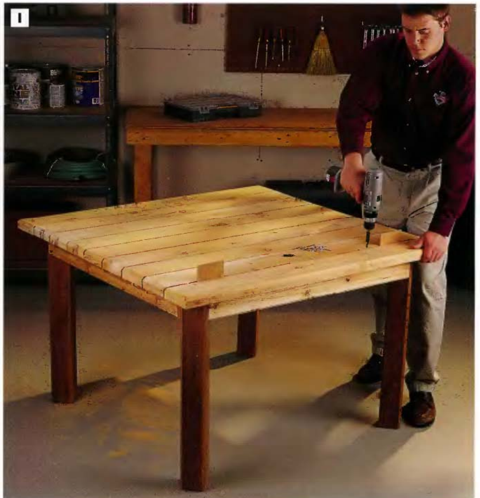
PHOTO I: Attach the top slats to the aprons with 2 \frac{1}{2} -in. deck screws. Fasten the center slat first, then work outward. This way, the overhang will be consistent on both ends of the table, and the slats will be evenly positioned. Use a pair of \frac{3}{16} -in. spacers to create uniform gaps between the slats.
