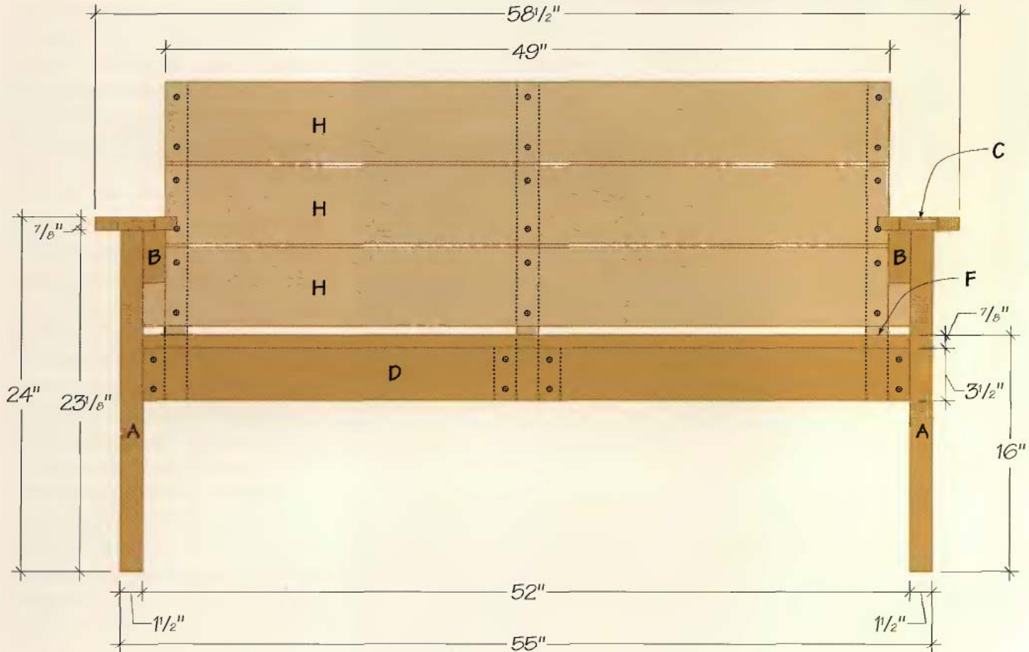
FRONT ELEVATION
