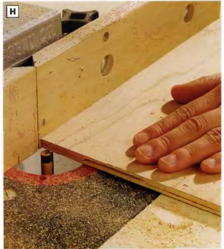
PHOTO H: Rout a shallow rabbet around the top face of the bottom panel for the veneer inlay strips. Install a \frac{1}{2} -in. straight bit in your router table to cut this \frac{1}{32} -in.-deep rabbet. Practice on scraps first and test the fit of the strips in the rabbet.
