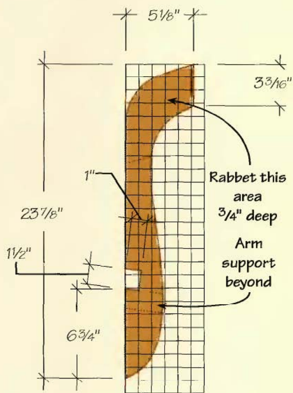
BACK SUPPORT
