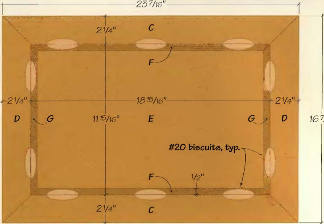
TOP VIEW ASSEMBLED BOTTOM
