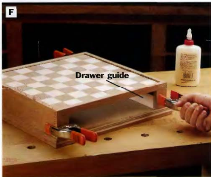
PHOTO F: Cut and glue a drawer guide into the recesses on either side of the drawer openings. Clamp the guides from both sides of the chessboard while the glue dries.
