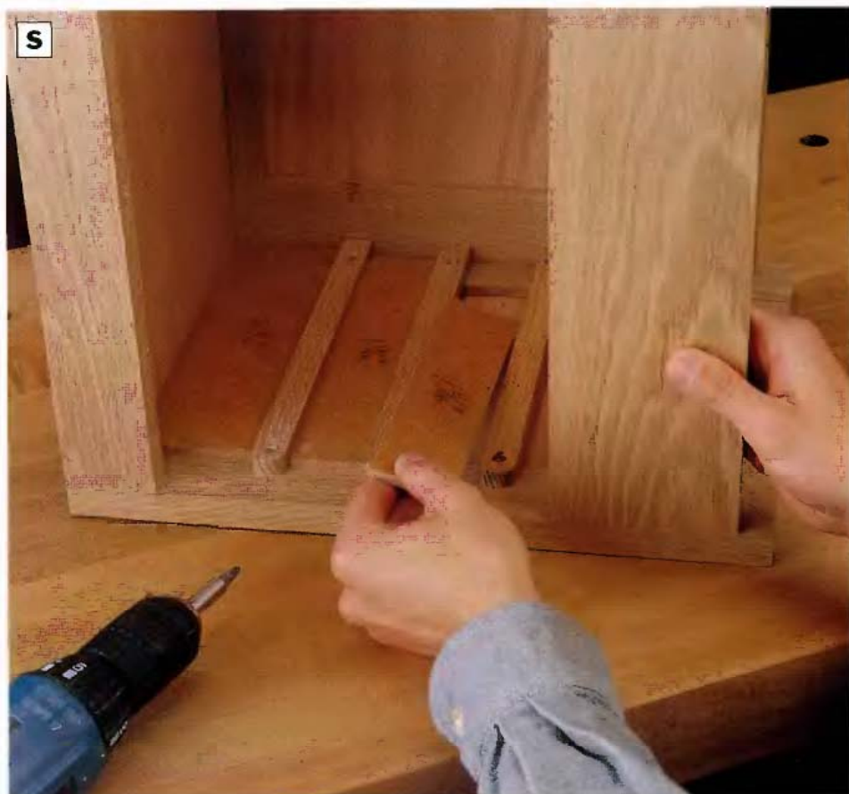
PHOTO S: Mount the drawer slides using spacers to maintain even placement. After the slides are in place, remove the spacers.
