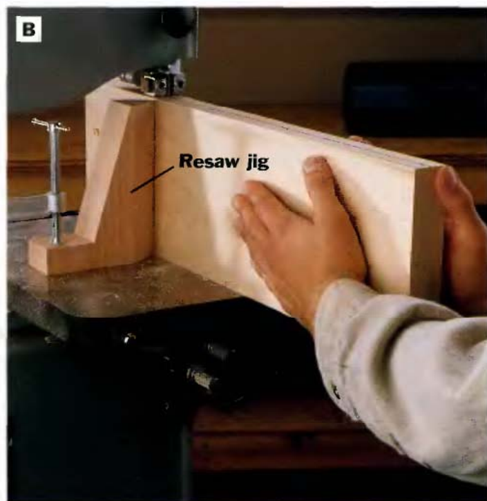
PHOTO B: Resaw the maple stock in half for the sides and ends of the box, using a marked centerline as a guide for the blade. A shop-made resaw jig clamped to the saw table will help square the board to the table and keep the blade tracking along the cutting line.
