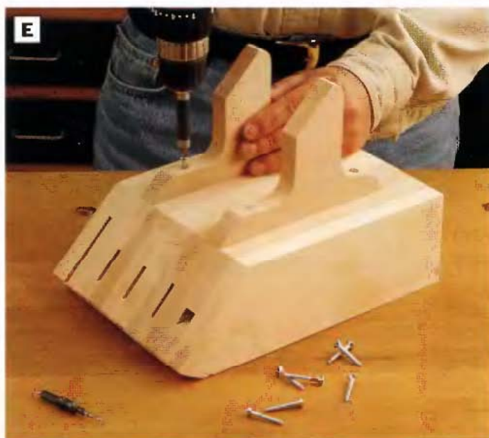
PHOTO E: Drive flathead wood screws through the feet and into the bottom of the knife block. Drill countersunk pilot holes for the screws first, to make screw installation easier and to recess the screw heads.
