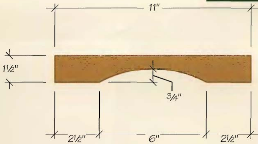
HANDLE
