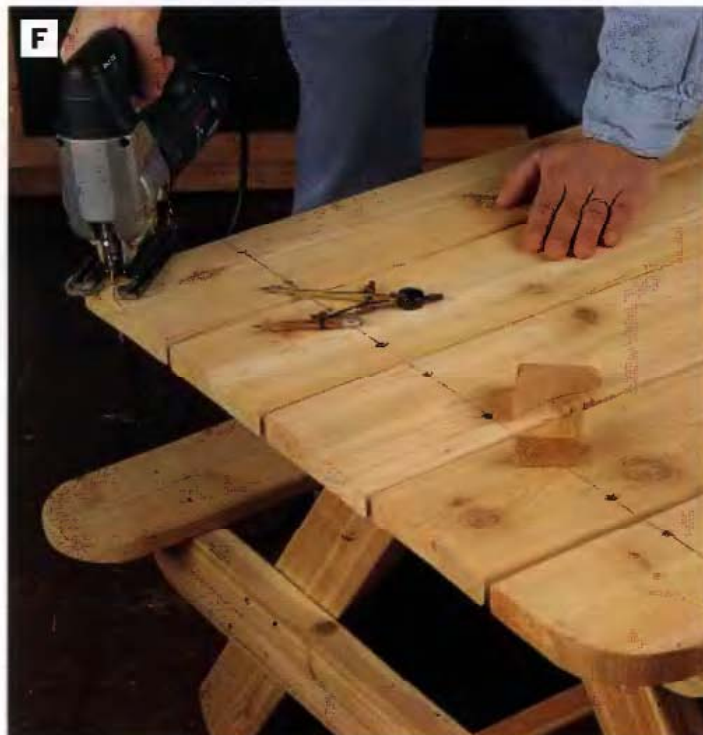
PHOTO F: Mark a 2\frac{3}{4} -in. radius on each of the four corners of the tabletop, and trim the corners with a jlg saw.
