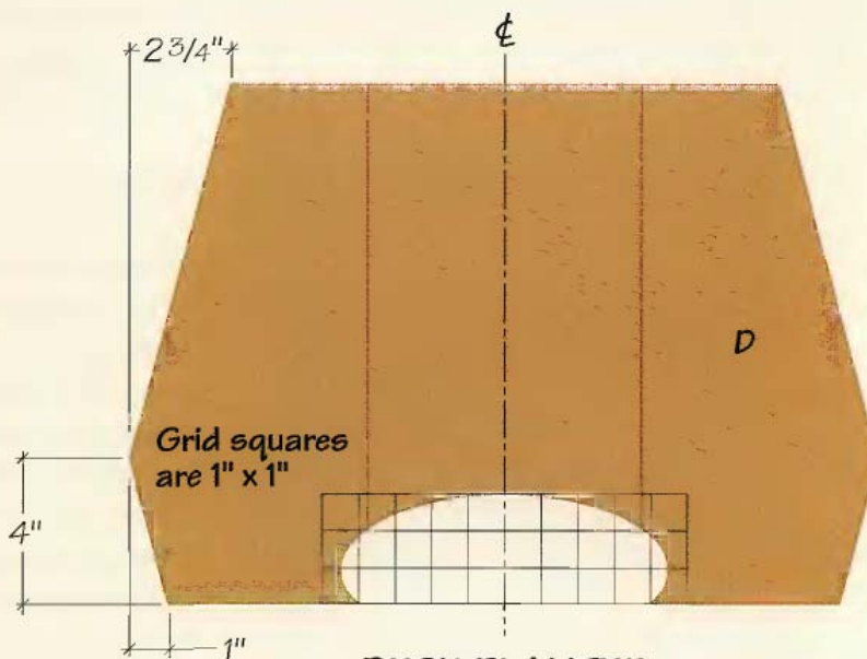
DECK PLANTER
