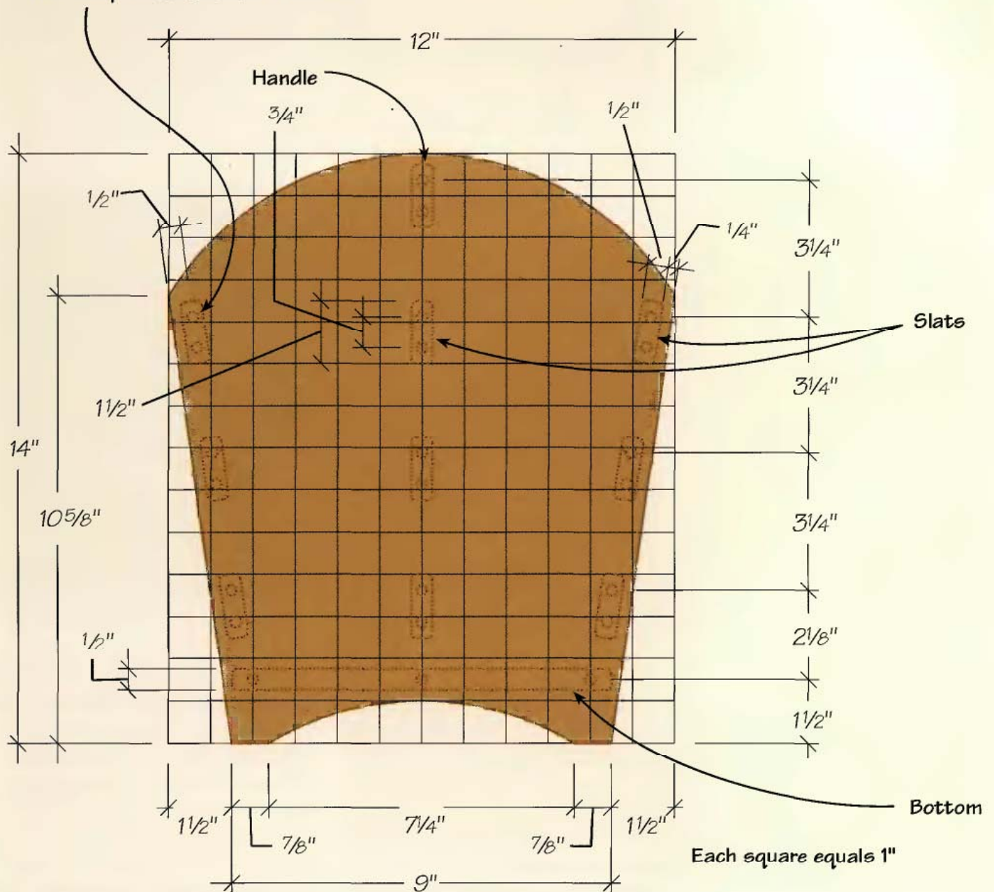
END VIEW
