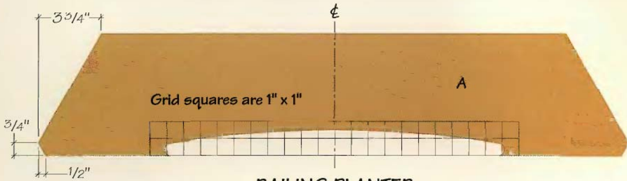
RAILING PLANTER
