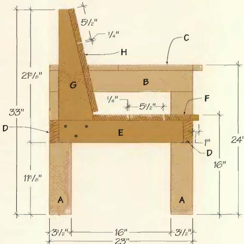
SIDE SECTION
