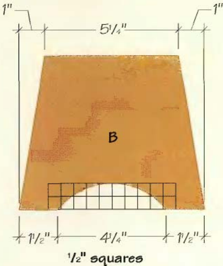
STRETCHER LAYOUT
