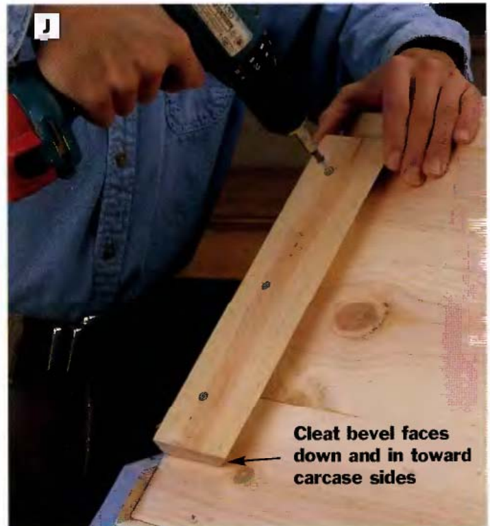
PHOTO J: Attach French cleats to the sides of the cabinet, flush with the top of the carcass. The cleat bevels face down and into the sides.
