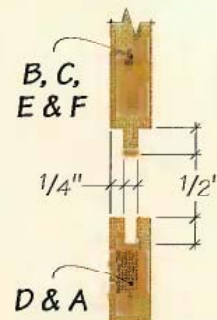
TOP VIEWS
