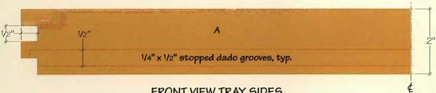
FRONT VIEW TRAY SIDES
