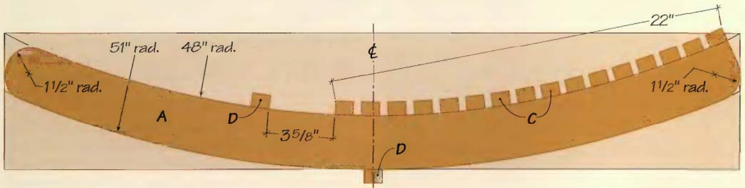
BACK SUPPORTS
