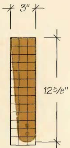
ARM SUPPORT
