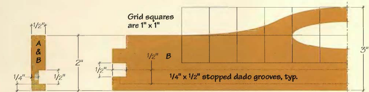
DETAIL: DADOES
