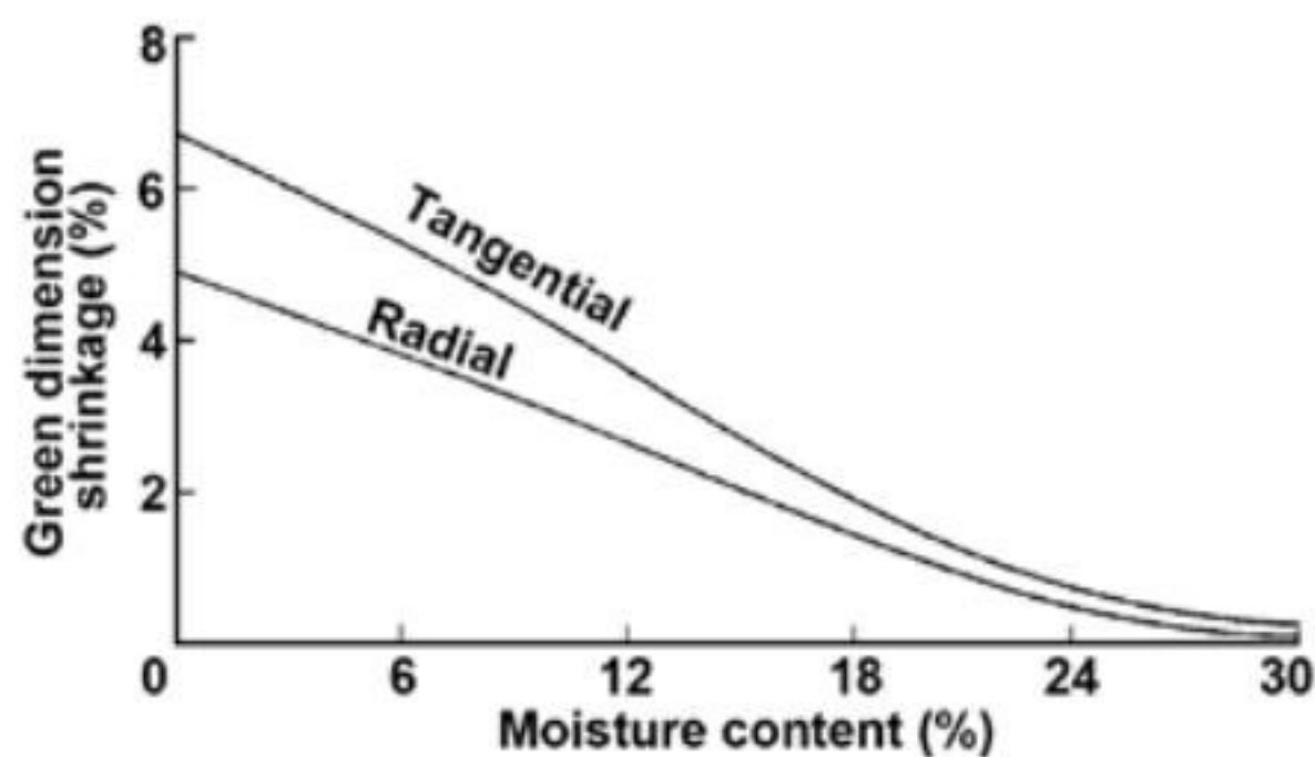
Figure 4-4. Typical moisture content–shrinkage curves.
