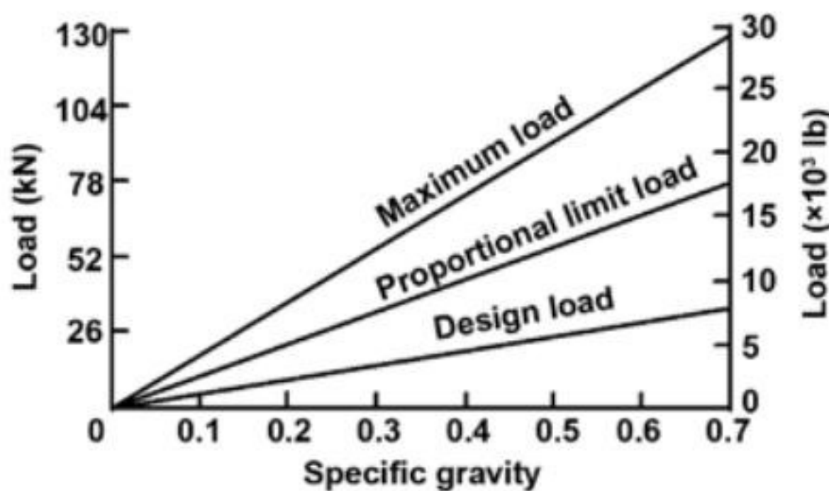
Figure 8-18. Relation between load bearing parallel to grain and specific gravity (ovendry weight, volume at test) for two 63.5-mm (2-1/2-in.) split rings with a single 12.7-mm (1/2-in.) bolt in air-dry material. Center member was thickness 101.6 mm (4 in.) and side member thickness was 50.8 mm (2 in.).
