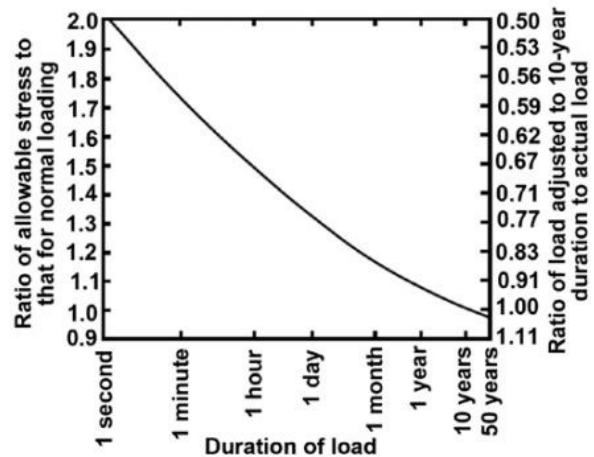
Figure 7–9. Relation of strength to duration of load.
