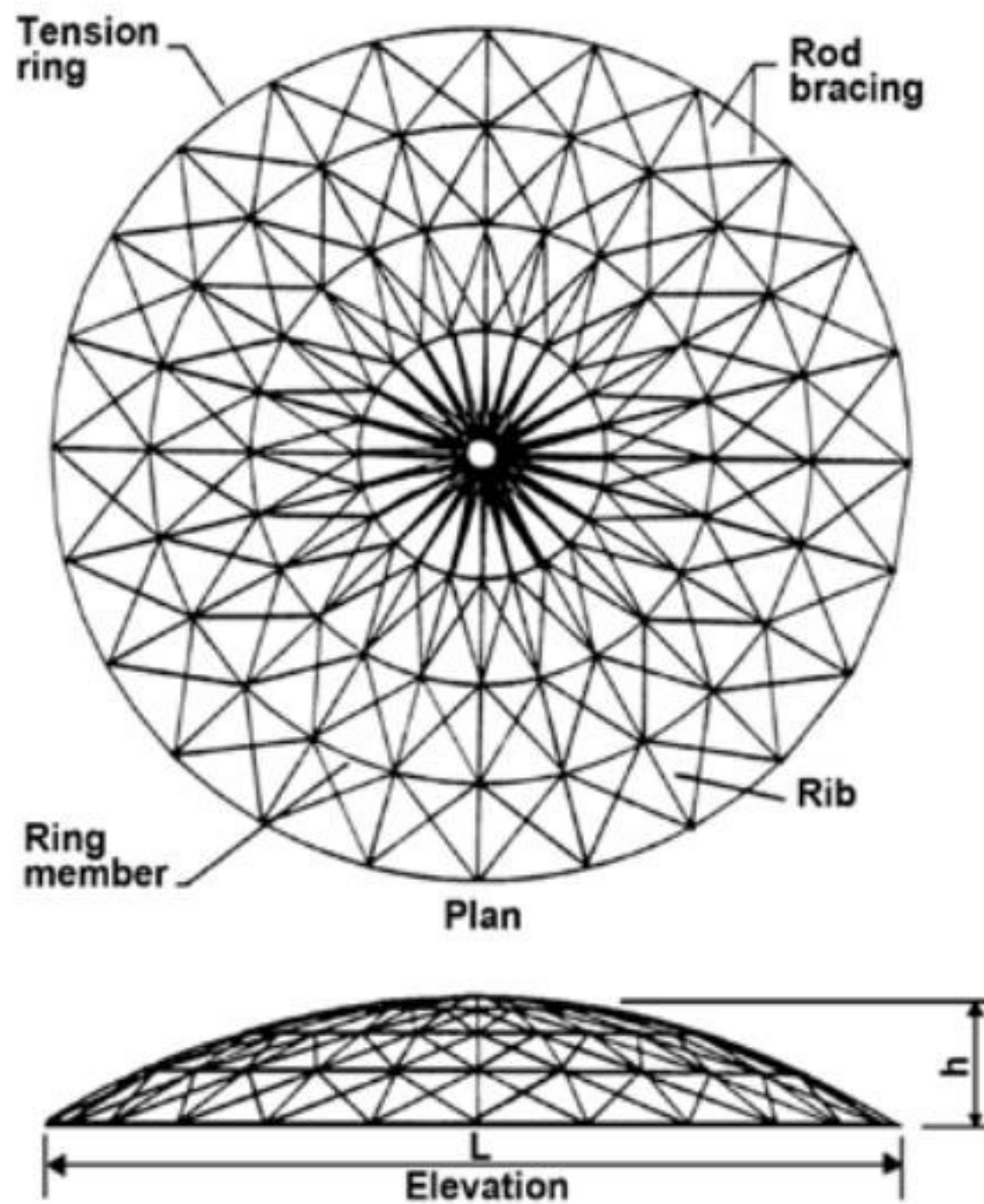
Figure 17-7. Member layout for a radial-rib dome.
