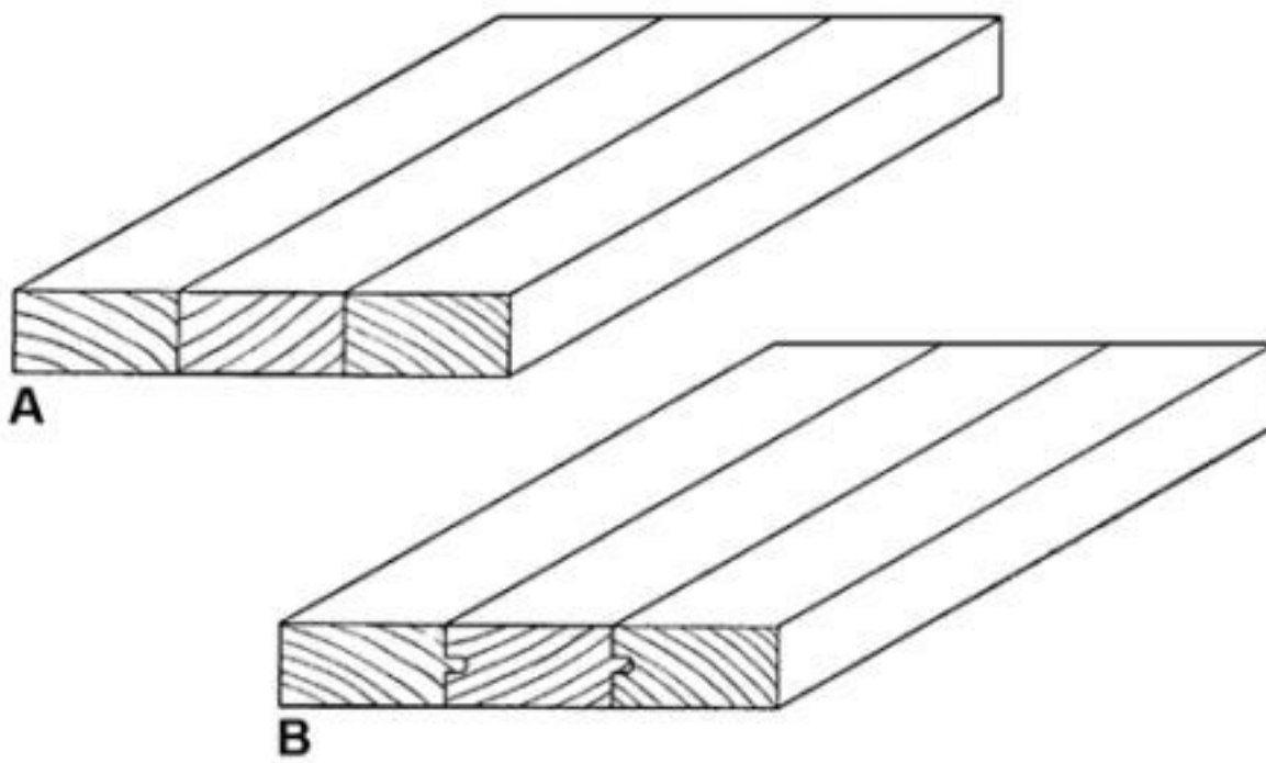
Figure 10-9. Edge-grain joints: A, plain; B, tongue-and-groove.
