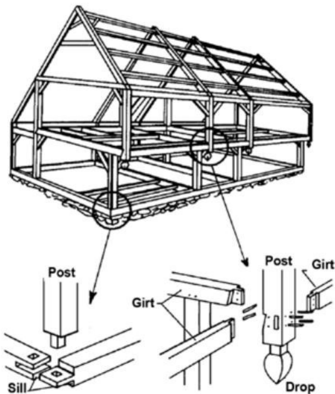
Figure 17–6. Timber frame structure with typical joint details.
