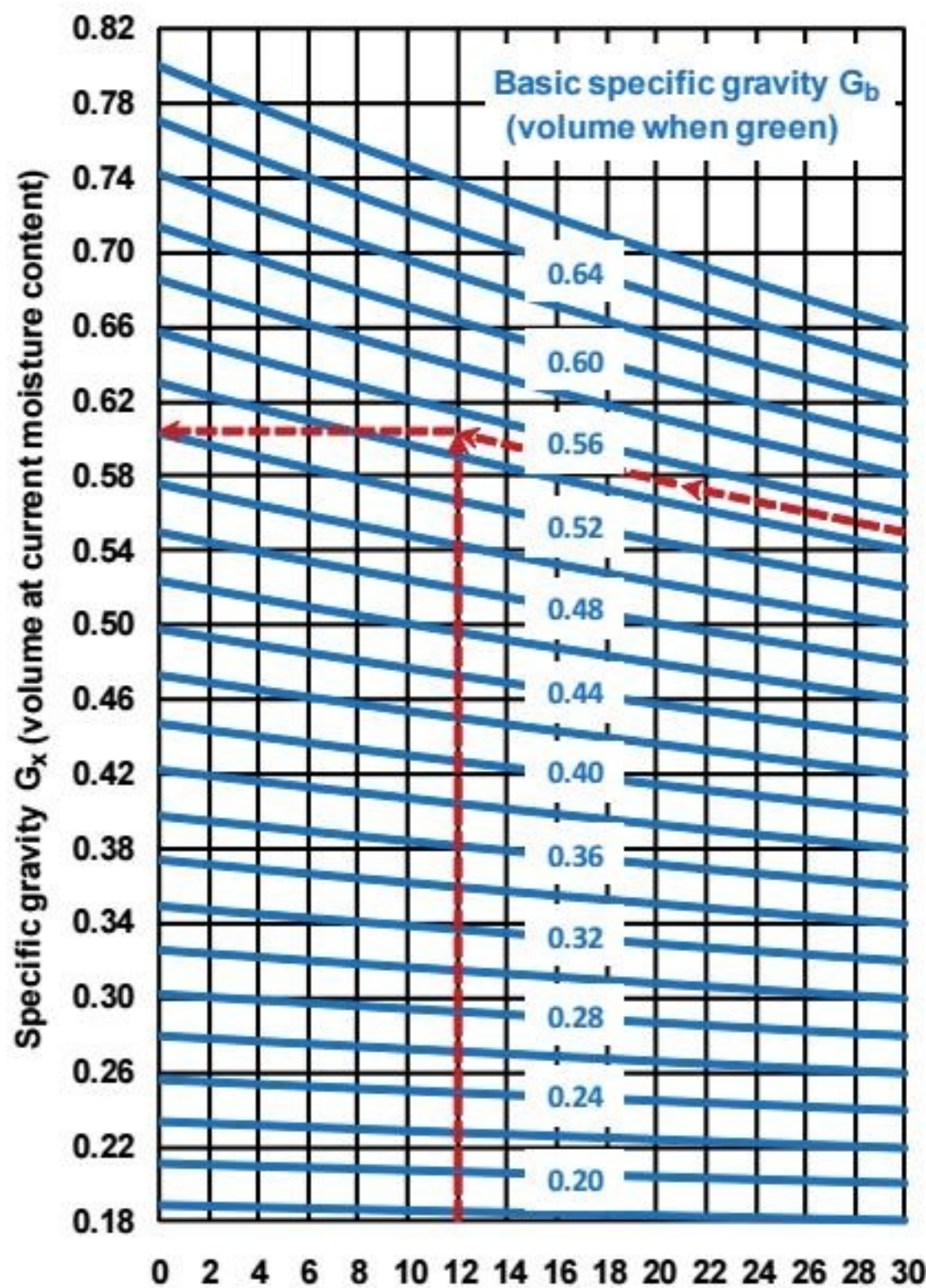
Figure 4-6. Relationship of specific gravity and moisture content.
