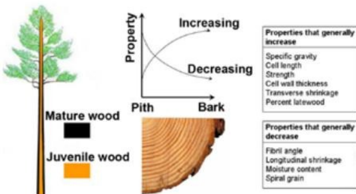
Figure 5–9. Properties of juvenile wood.
