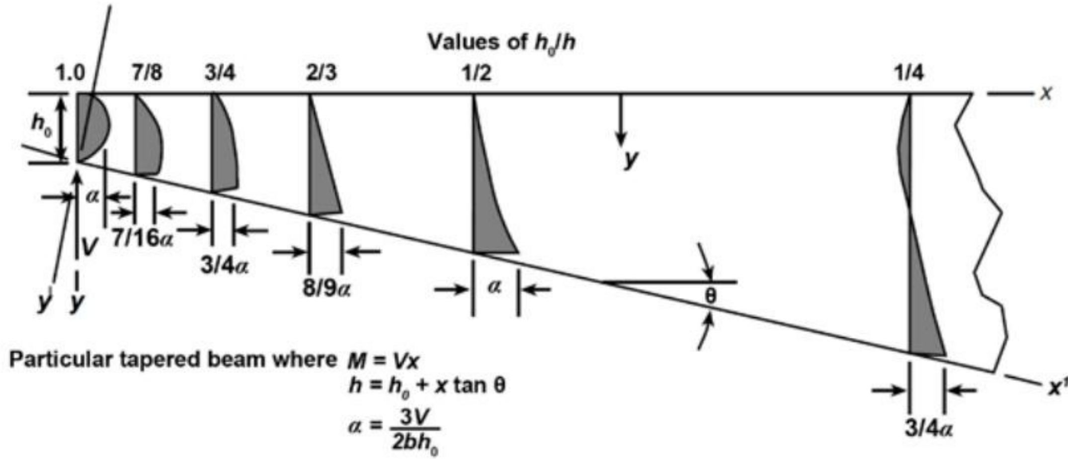
Figure 9-4. Shear stress distribution for a tapered beam.
