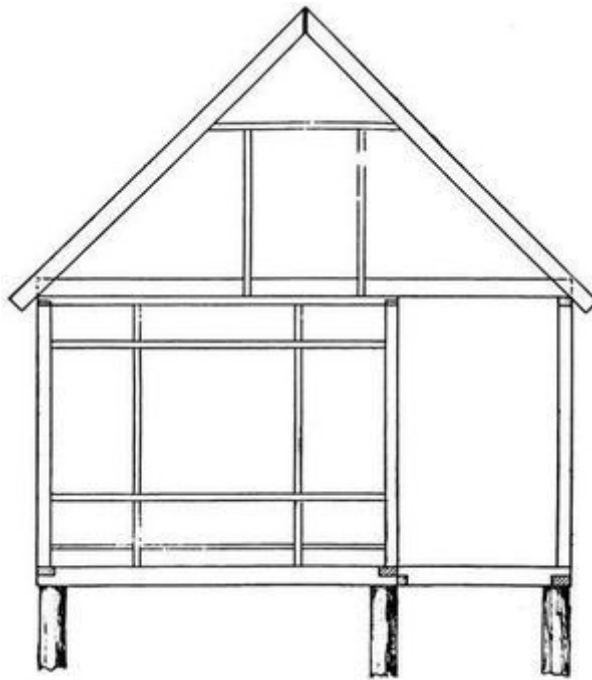
Fig. 396. END ELEVATION.
