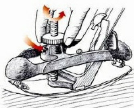
ABOVE: Adjusting the sole. When completed, tighten the locking screw.
