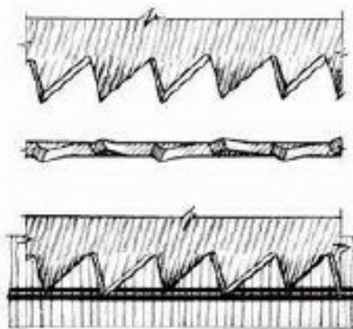
ABOVE: The shape and profile of the crosscut saw results in a scoring-and-slicing cut.
