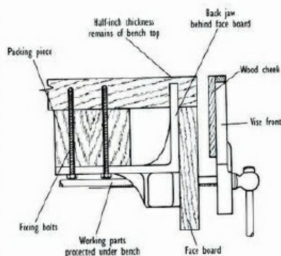
ABOVE: Large vise fixed by coach screws.
