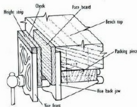
ABOVE: Small vise fixed with screws.
