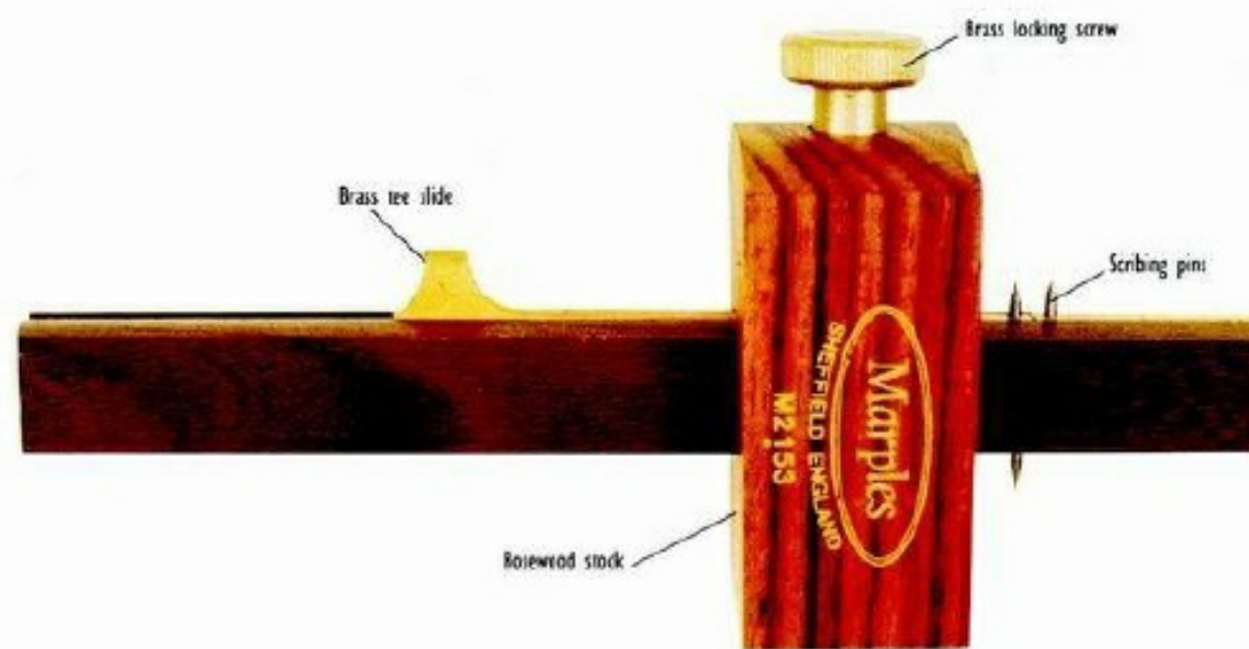
RIGHT: Combination mortise and marking gauge.
