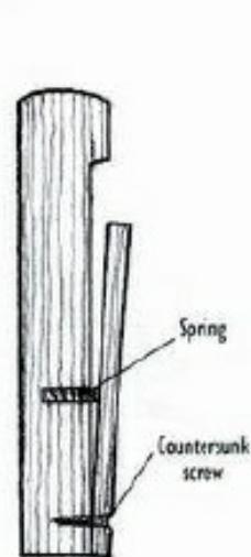
ABOVE: Quick-release bench stop made of wood.
