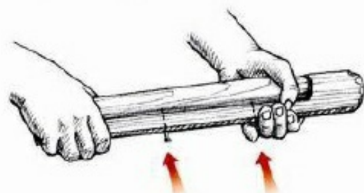
ABOVE: Chair leg jig. Set the leg in the jig, press them together so that the nail points mark the position of the stretcher holes.
