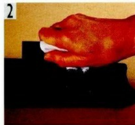
ABOVE: Hold the scraper with a piece of cloth so that you don't cut your hands. Hone the filed edge on a medium stone. Aim for a square-cut polished edge.
