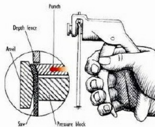
ABOVE: The saw set in action.
