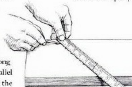
LEFT: Make sure that the 0 and 7 inch marks are perfectly aligned with the edges of the board.
