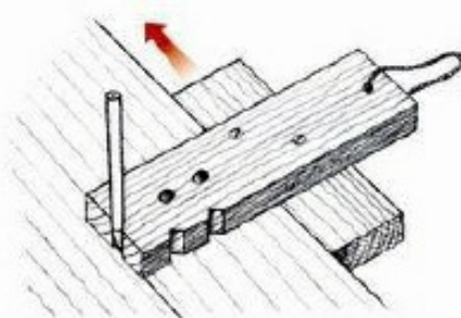
ABOVE: Cross jig. Slide the jig hard up against the workpiece so that the pencil marks a line that is parallel to the edge.
