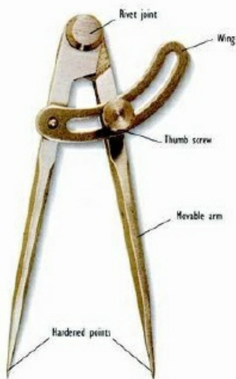
ABOVE: Wing dividers.
