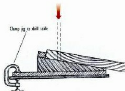
ABOVE: Angle-drilling jig – the jig allows you to drill repeat holes at the same angle.
