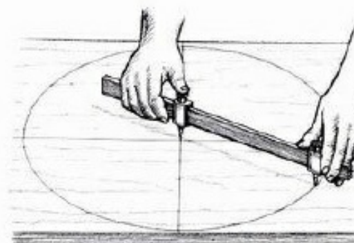
ABOVE: Spike one trammel point down on the center and swing the other point to scribe the circle.
