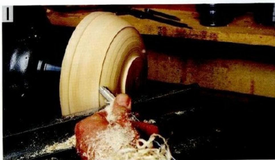
ABOVE: A well-formed, turned bowl.
