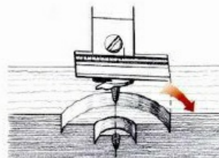
ABOVE: Cross-section showing the expansion bit in action.
