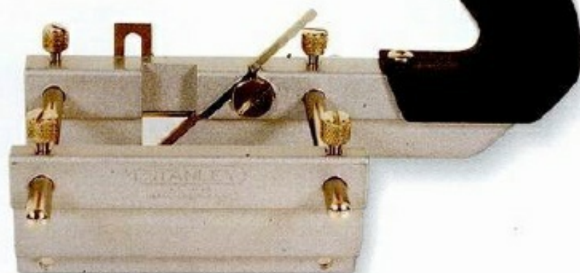
LEFT: The plough plane is designed specifically to cut grooves and channels.
