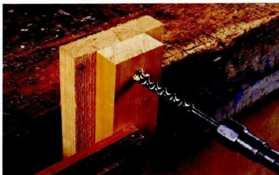
ABOVE: For maximum efficiency, the waste piece needs to run down to the floor.
