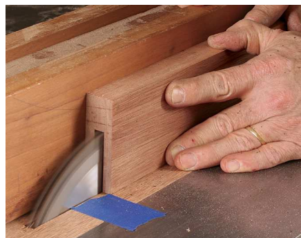
Clear a path for a new one. Use a dado set to plow a groove where the tenon should have been.
