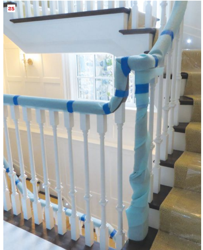
Hardwood stairs can be protected using hardboard or plywood tread covers (24), secured to skirtboards using cleats. For stair railings, the author recommends wrapping the railing in sill sealer and tape (25). Foam board works well for protecting walls (26).
