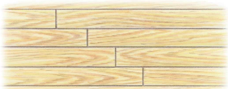
Staircasing
