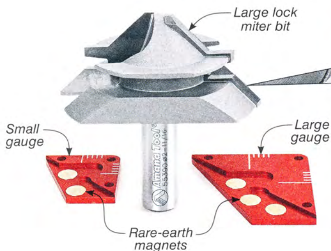
▲ Registration. The raised edge of the gauge should be tight against the cutting edge.
