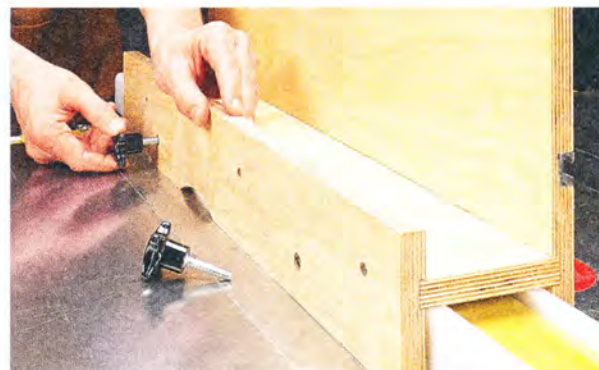
▲ Threaded Inserts & Knobs. For a fence that will see lots of action, it's worth going to the trouble of installing threaded inserts and knobs.
