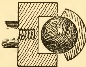
FIG. 133.—SECTION OF HOME-MADE CHUCK.
