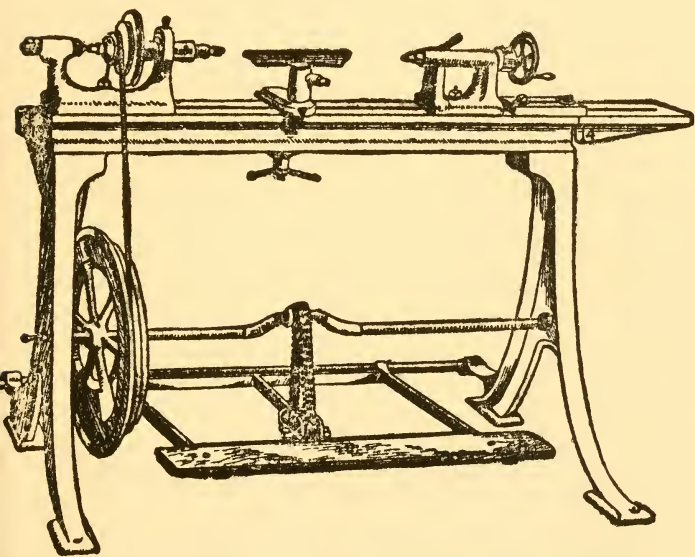
FIG. 1.—SKETCH OF STANDARD TREADLE LATHE, WITH EXTENSION PIECE.
