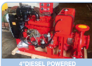
4" DIESEL POWERED WATERPUMPS 4 CYLINDER DIESEL 80M3 / HR 20-30M HEAD
