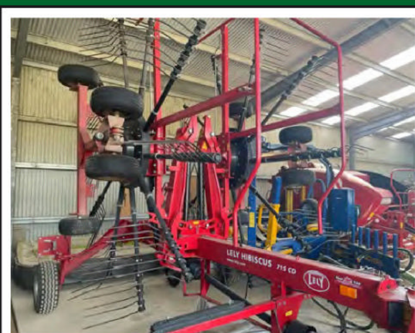
2014 Lely Hibiscus 715 CD 715, twin rotor rakes, well maintained machine OBOC. Located on farm Leongatha.
