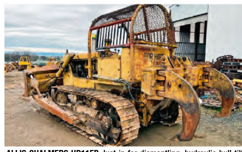
ALLIS CHALMERS HD11EP Just in for dismantling, hydraulic bull tilt blade, swivel tyne rear rippers, turbo 11,000 series running engine, Powershift transmission and converter, good undercarriage all round, all parts available, phone Brendan on 02 6762 4466. S172. TA1144219. POA
