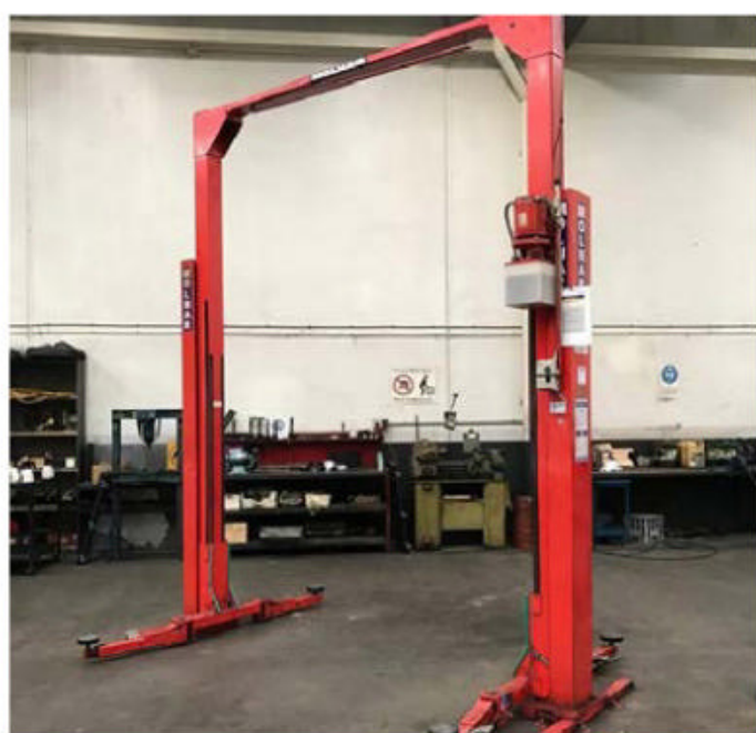
Molnar MF1705-93-OH-3T Clear floor car hoist, type MF1705-93-OH-3T, 3 ton capacity, 2 post.
