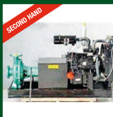
SOUTHERN CROSS 80X50-315 Isuzu 3AE1, 30 hp diesel, 15 litres per second at 80 metre head. AW54939-FM077-112-02. DPLIn27518. $7,850 + GST
