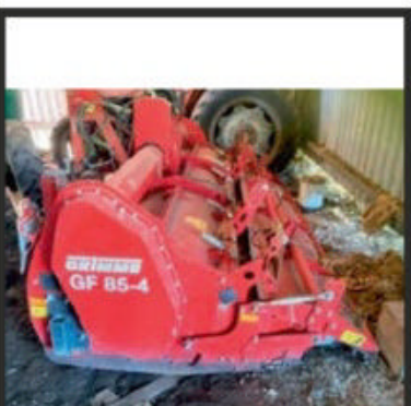
GRIMME GF85-4 4 ROW POTATO HILLER near new tines with a spare set of new tines. Hardly used, TBA. QLD. DIY1132032. 0409 641 130. $45,000
