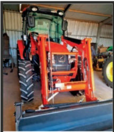
KIOTI RX8030 2019, cab tractor 80hp, power shuttle, FWA, loader with 4in1 bucket, S59SHN. SA. DIY1132228. 0419 819 649. $62,500
