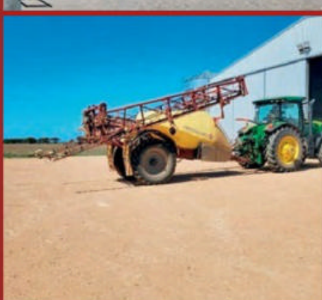
HARDI 5030 COMMANDER Eagle SPC Boom 364 Pump 4 Section EFC Fluid System Venturi Fill ISO/JD Controller 35 Litre Chemical Hopper 18.4-38 Tyres Coming July 2022. 102780. TA1125710. $38,500
