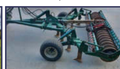
COUSINS V-Form 4.25m 7 leg trailed subsoiler c/w Razor Ring packer
