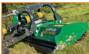
SPEARHEAD SNIPER 280 SHD £6,950 NEW 2.8m heavy duty front or rear mounted flail, 400mm hyd offset, Adjustable rear roller, Front flaps and chains, Hammer flails, 2.5m working width, 5 belts, all welded construction.
