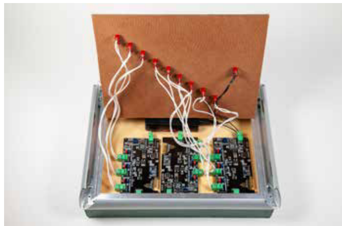
6 Tipping up the control panel diagram provides access to the battery and transmitters for wiring. The removable screw terminals allow for quickly removing the track diagram.
