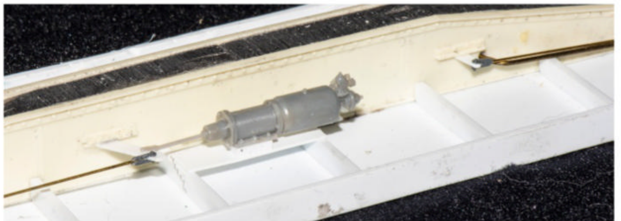
6 Worth the effort. The straight side sills on the flatcar make the brake details easy to see. Charles used commercial parts from San Juan Model Co. as well as scratchbuilt brass parts to re-create the K brake system.
