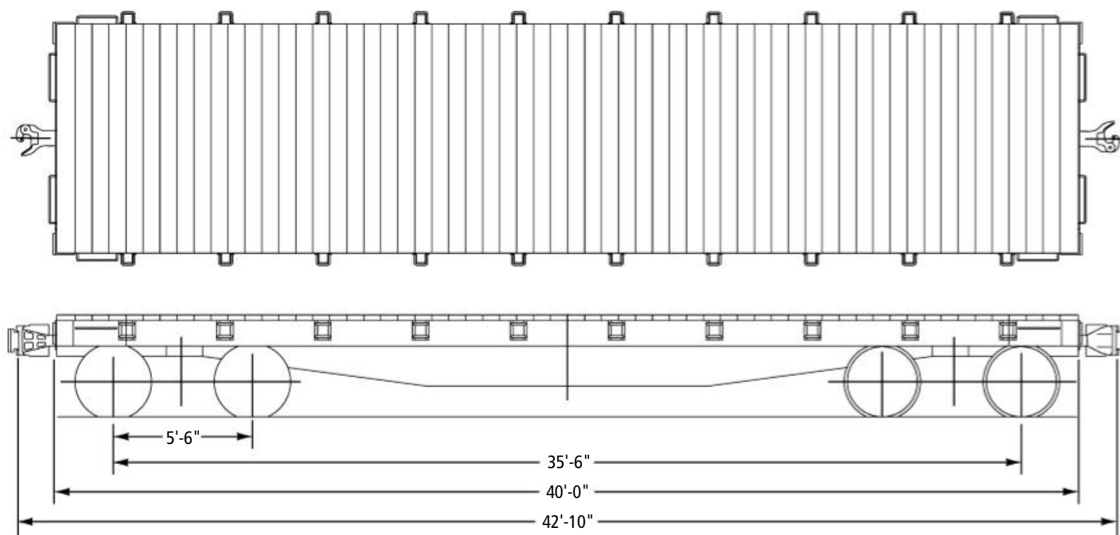
DENVER & RIO GRANDE WESTERN 21000-21249 SERIES FLATCAR
