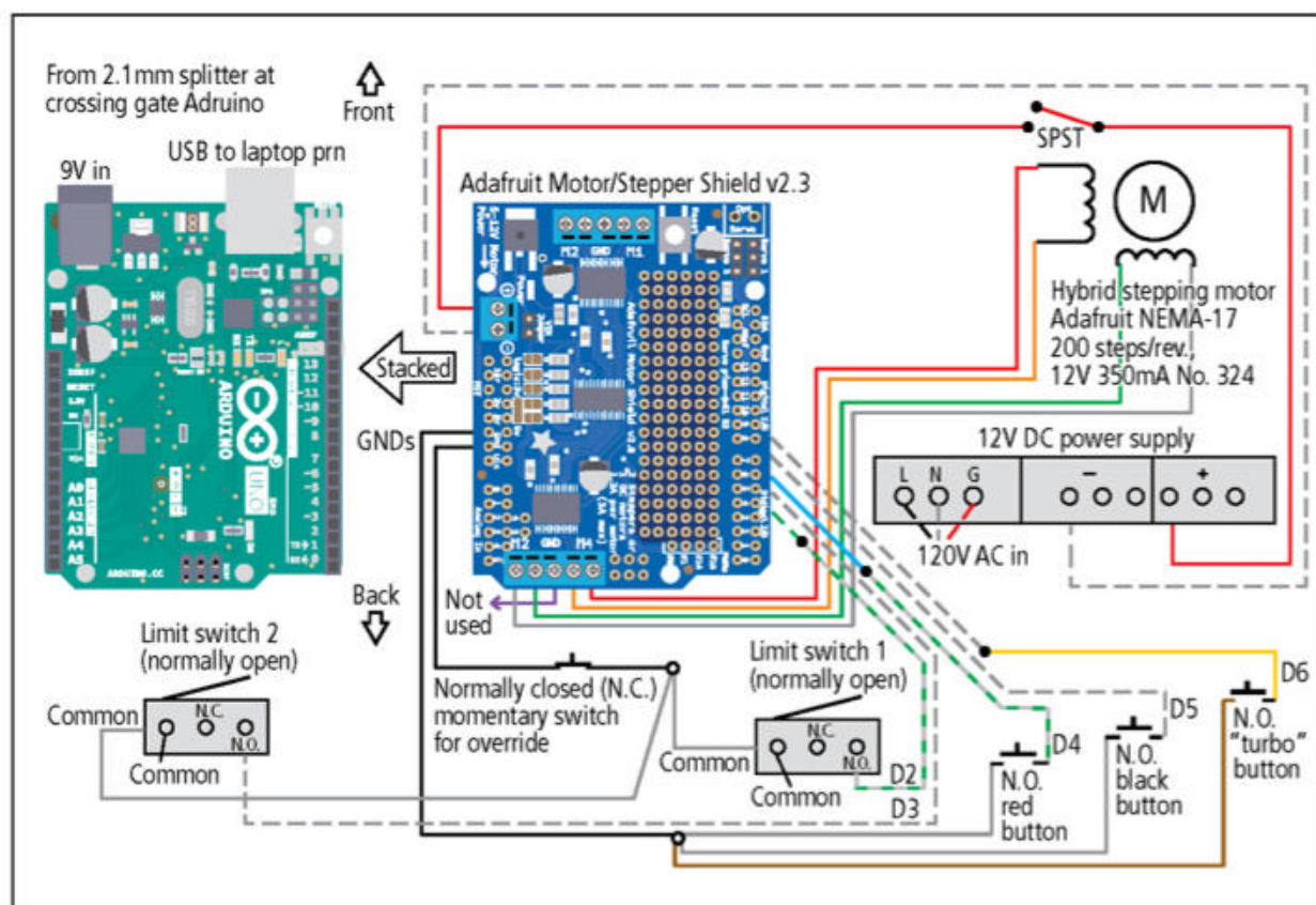
5 This illustration shows how the Arduino Uno, Adafruit MotorShield, and stepper motor are connected to each other and the position of switches in the circuit.
