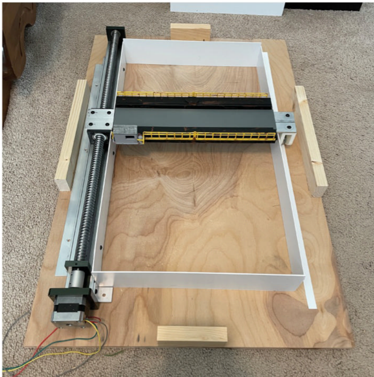
2 The stepper motor and slide rail mechanism that moves the transfer table is shown mounted to 1/2"-thick furniture-grade plywood.
