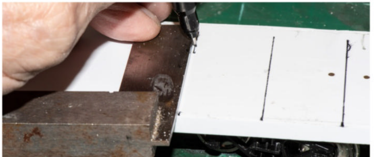
7 Mapping things out. Charles used a divider to mark the locations of the stake pockets on one side of the car. He used a square and fine-point marker to transfer those locations across the deck and to the car sides.
