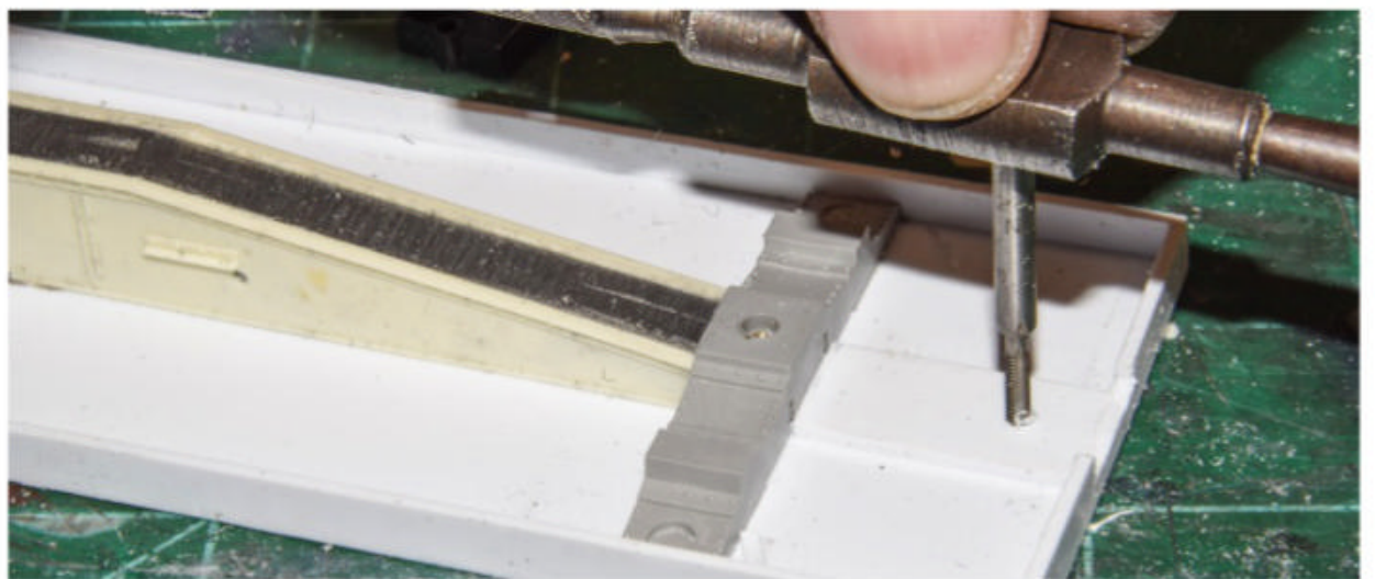
5 Underbody work. After marking the location of the center hole in the draft-gear box with a punch, Charles drilled and tapped the styrene for 2-56 screws. He held the tap at a right angle to the body so the screw would seat properly.
