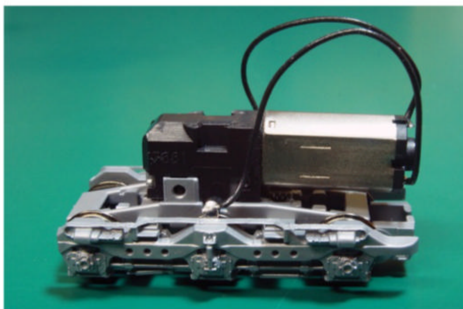
4 After mounting the motor and worm gear to the truck, Ron hooked up the motor leads to the truck's power pickups and tested it with a DC power pack. It ran.
