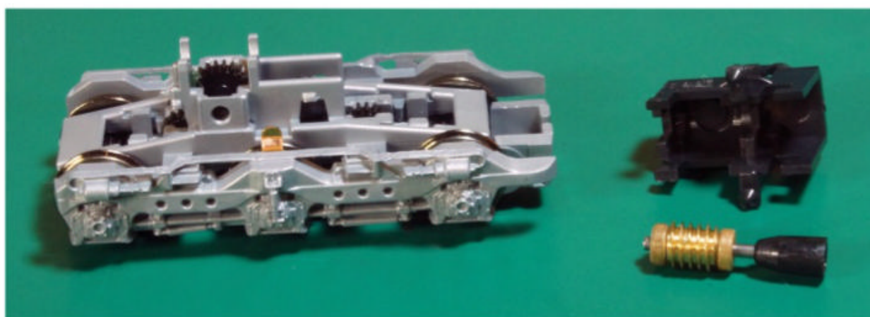
2 Ron removed the gear tower enclosure and the worm gear. He trimmed the plastic gear housing to make room for the motor and DCC decoder.
