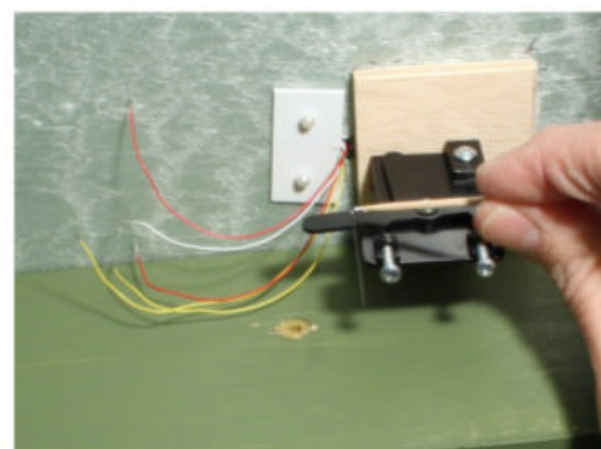
⑨ The next step was to bend the gate actuating wire. Tom marked that location using white paint applied with a toothpick.
