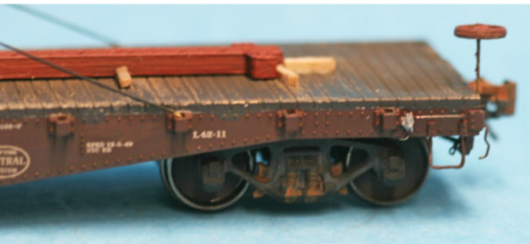
5 Small but important. On the left side of the car, between the stake pocket and grab iron, is the retainer valve. Mont used a Precision Scale Co. part to add this detail.
