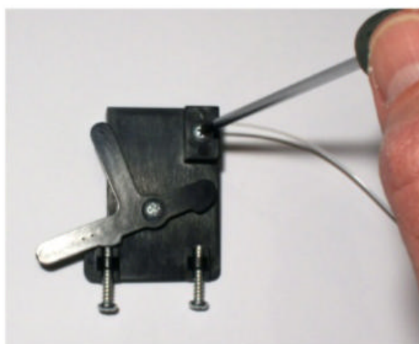
⑩ Tom used a Phillips-head screwdriver to clamp the tubing in the bracket on the actuator. He then ran the actuating wire through the tubing.
