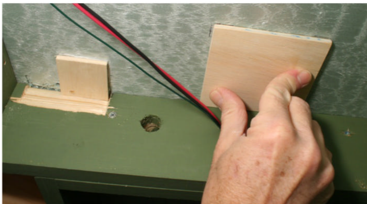
⑦ Tom used foam-safe adhesive to attach wood mounting plates to the bottom of his layout. The plates allowed him to secure the drive mechanism and actuators with screws.
