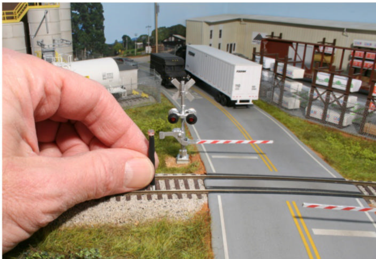
14 Tom inserted the photocells for the grade crossing flashers from the top of the layout. He used a small amount of white glue to hold them in place.
