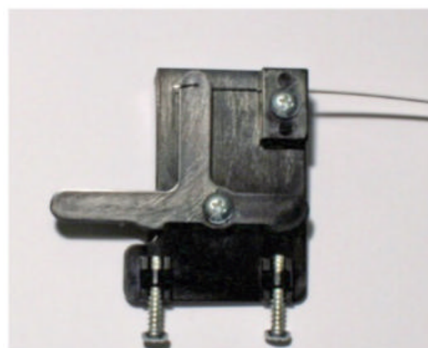
⑪ After bending one end of the stainless steel actuating wire into a Z shape, Tom inserted it into the bell crank arm.
