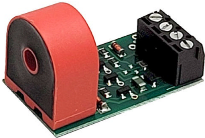
1 NCE BD-20 block detector. Note the hole in the tombstone-shaped current transformer for the wire to your detected track section.
