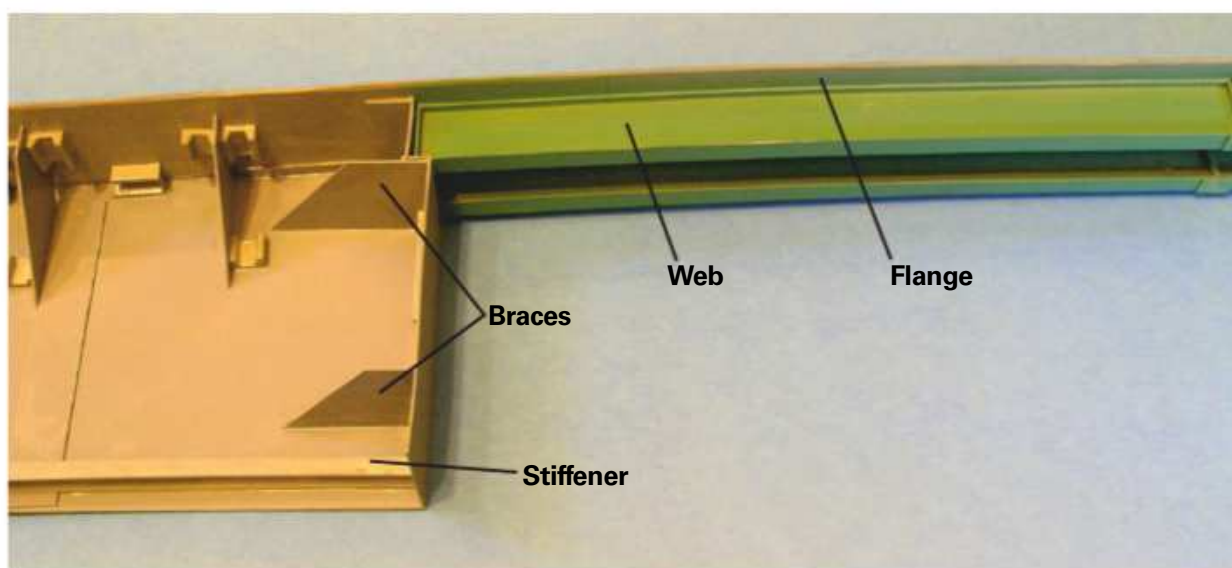
FIG. 2 USING STYRENE. Bruce used Plastruct .030" styrene to model the bridge abutments. He installed braces so the sides and ends of the abutments would be at right angles, and he added stiffeners so the thin styrene wouldn't bow.
