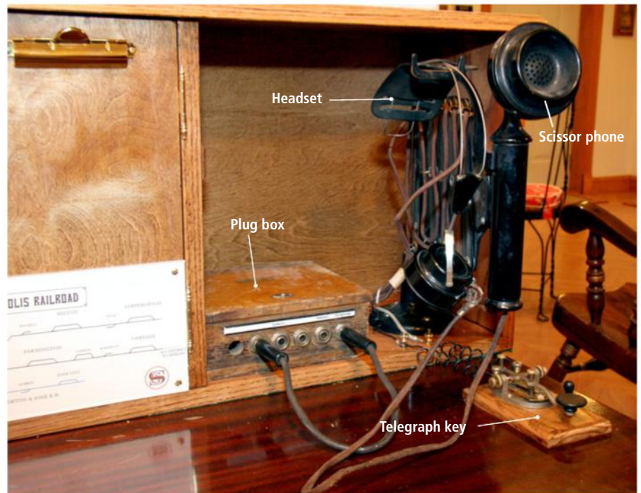
5 Lines of communication. The scissors phone mounts to the bottom of the console. Don attached felt to the bottom of the phone to prevent scratching the desk top. The small box to the left of the phone is a plug box to select whether the dispatcher will use the scissor phone and headset or a breastplate microphone with headset.
