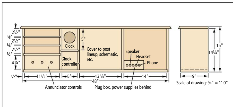
1 Drawing of the dispatcher's console. Don made the console using standard woodworking techniques.
