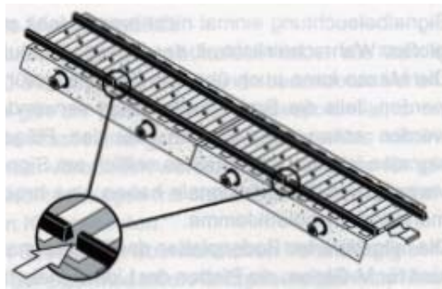
Contact track set 5145
