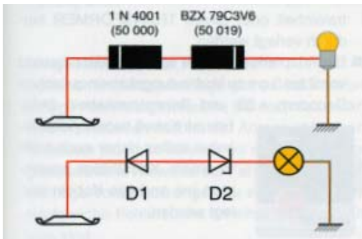
protective circuit from two diodes prevents a memory loss of the motive decoder
