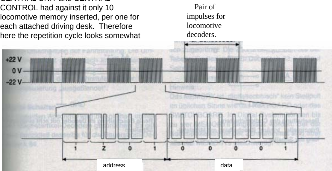
Timing diagram of the tension at the track (in the example represented: Locomotive address 34)
