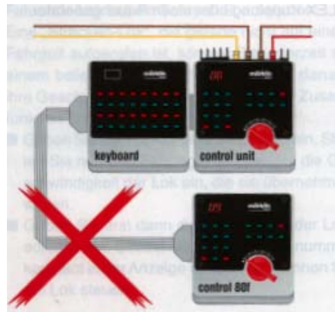
Correct connection of driving and placing desks with adaptor cables cables also the referring to page 64.
