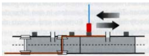
Picture: Operational principle of a contact track
