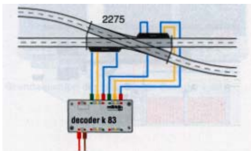
Connection of the crossing switch 2275
