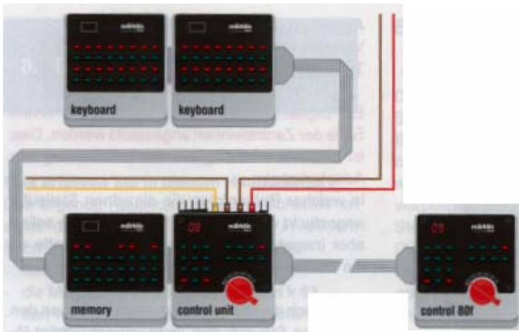
Correct connection of driving and placing desks with adaptor cables
