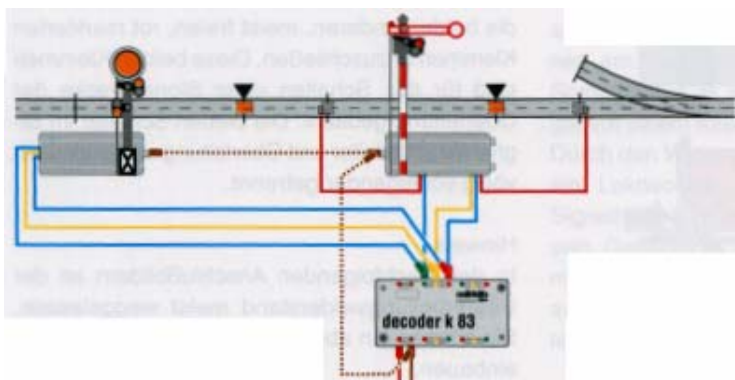
Connection of the form signals 7040 and 7038
