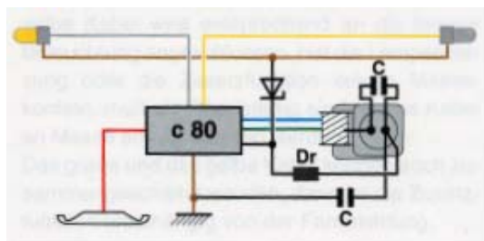
Connection lighting at engine return pipe
