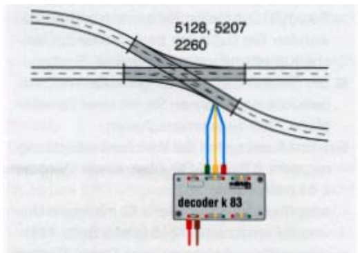
Connection of the crossing switches 5128 5207 and 2260
