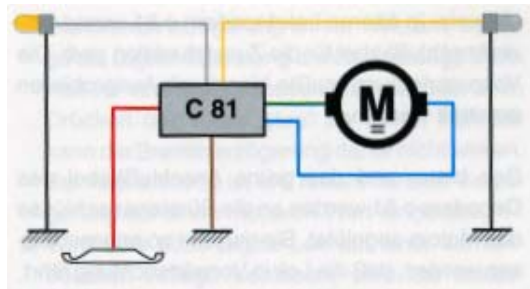
Standard connection of the locomotive decoder c 81
