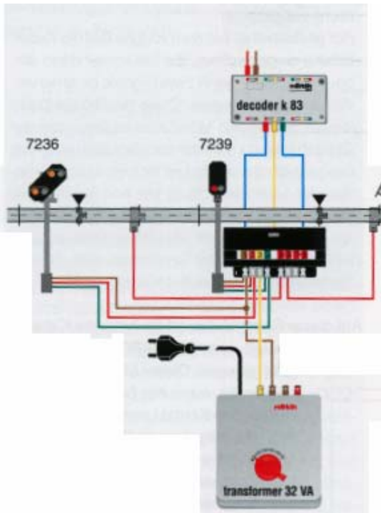
Connection of the light signals 7239 and 7236
