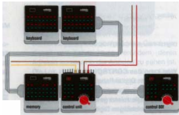
Correct connection of driving and placing desks with adaptor cables cables also the referring to page 64.
