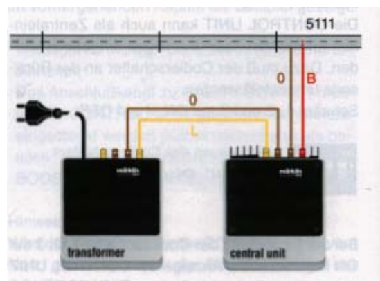
Connection of the cent RAL UNIT
