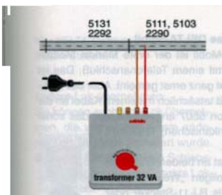
Conventional track connection with one TRANSFORMER 32 VA
