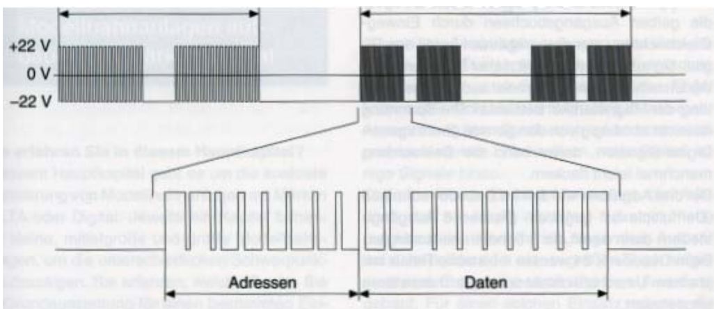
Timing diagram of the voltage at the track with a magnet article instruction
