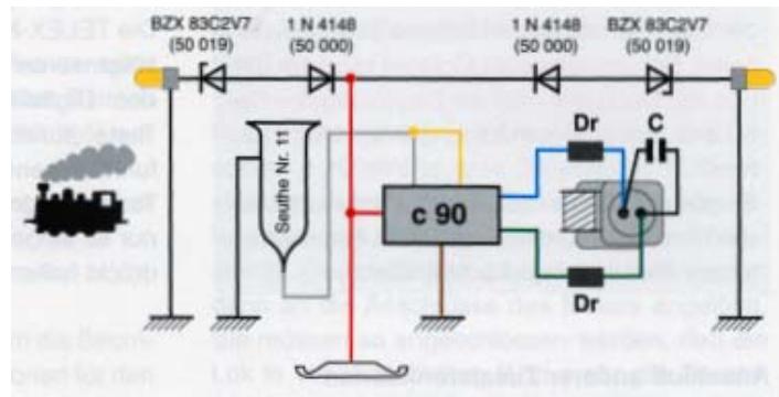
Auxiliary function smoke generator
