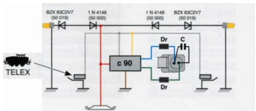
Auxiliary function TELEX clutch
