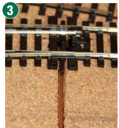
The copper tube was laid in the 3mm wide channel and when the adjacent line was relaid there was no misalignment.
