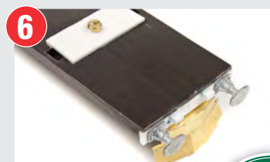
The completed headstock detail with frame ends showing. They will be detailed with an ETH socket and air brake hoses.
