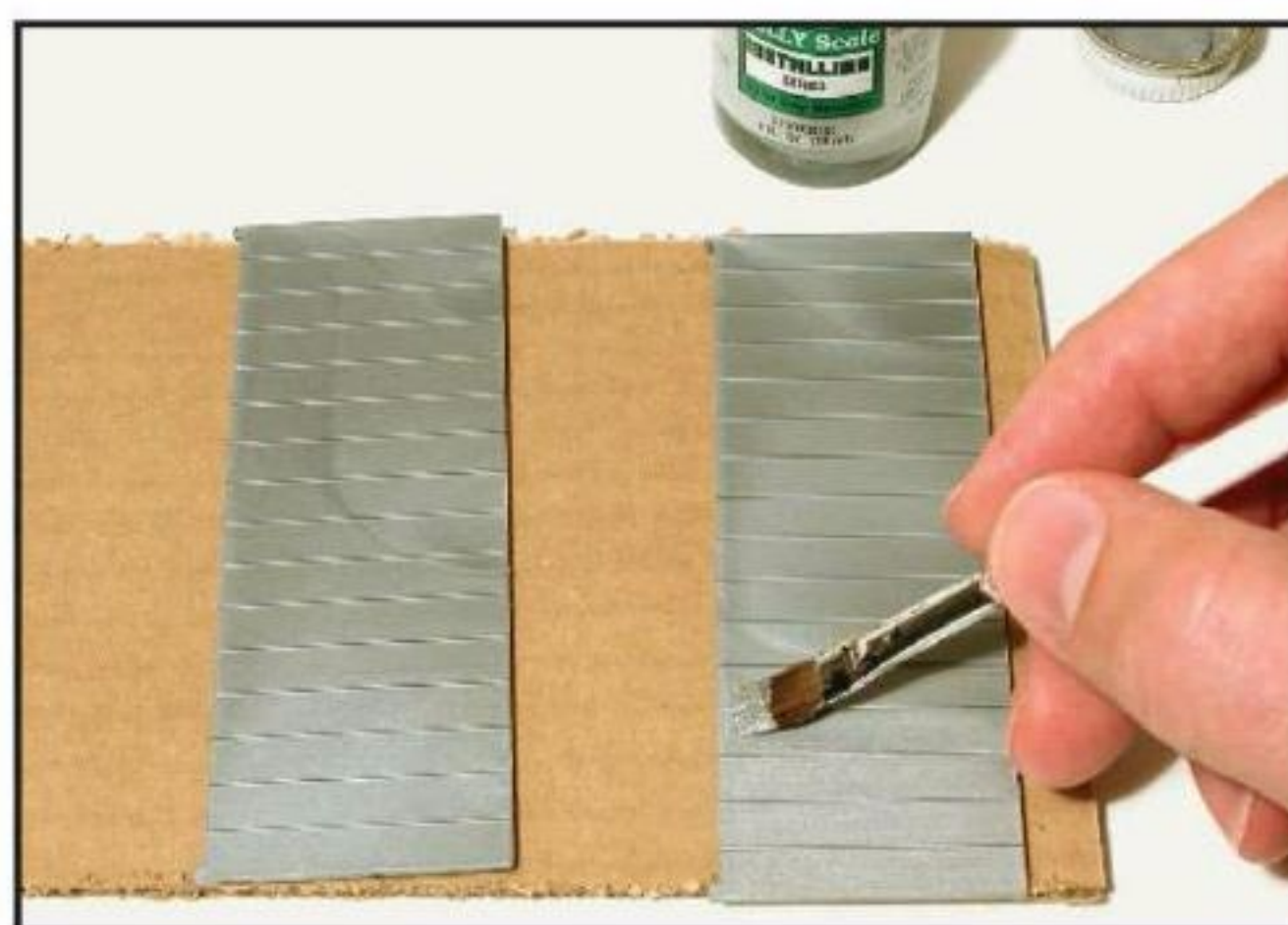
41 Polly Scale flat aluminum is a good base color for simulating galvanized metal. Brush it on parallel to the groove or ridges of the roof surface.
