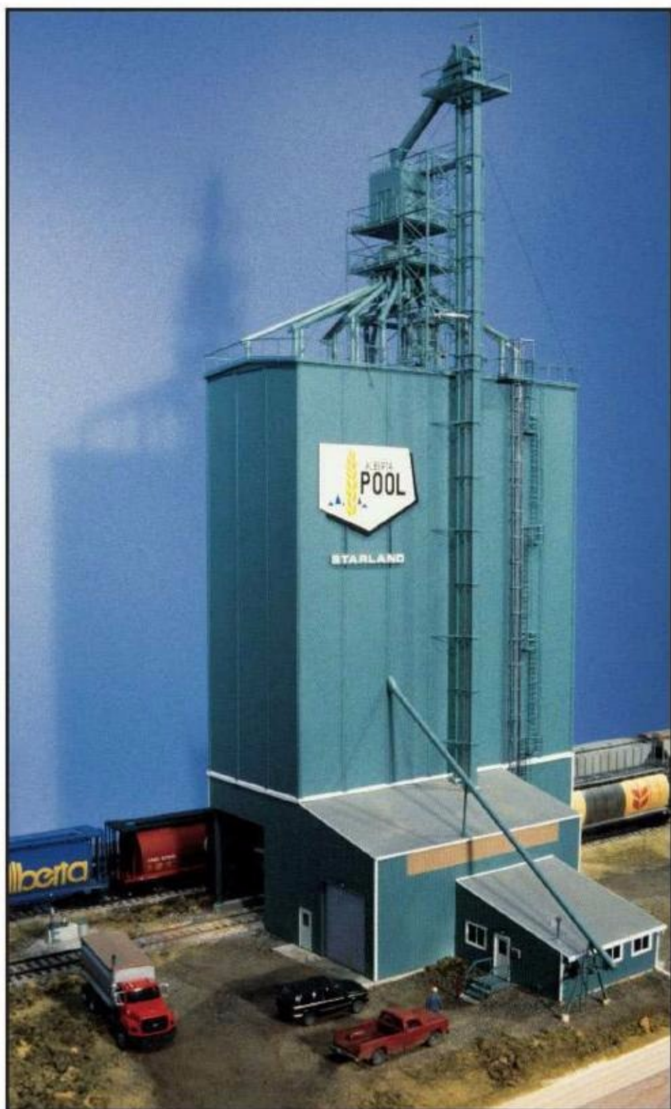
3 Jon Greggs built this impressive HO scale model of a steel grain elevator using sheet styrene and structural shapes, with details from a variety of sources. It was built to match a real grain elevator in Starland, Alberta, Canada. Jon Greggs photo
