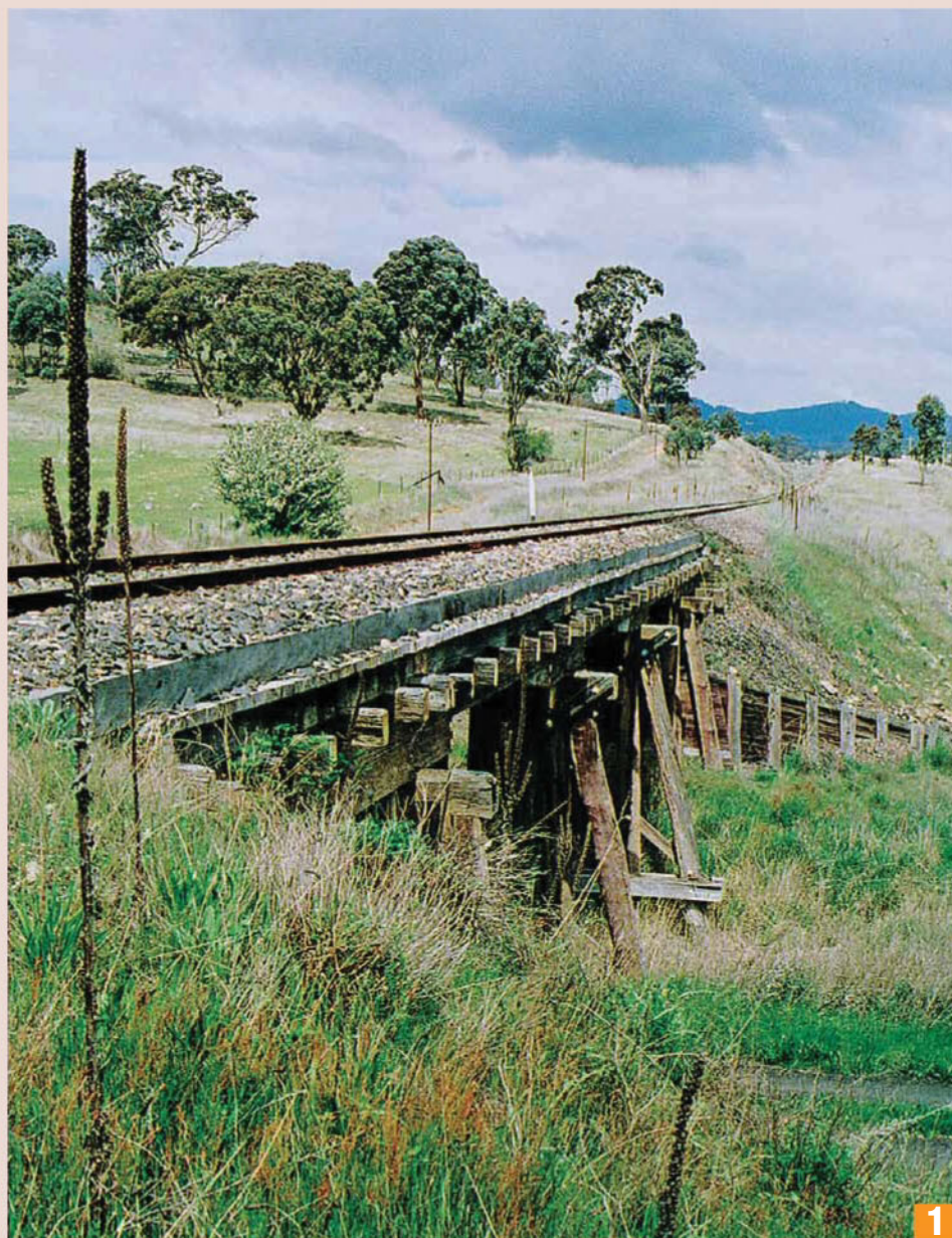
A Whitton-era ballasted deck timber trestle bridge on the Queanbeyan to Michelago section of the Cooma line, photographed by the author on 15 October 1999.
