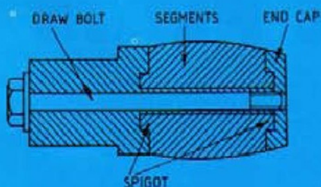
Fig. 9: Collapsible Former
