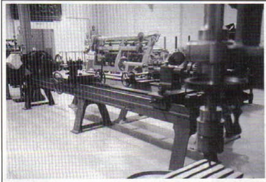
Fig. 15: This is a James Fox lathe of 1817, photographed at the Birmingham Museum of Industry.
