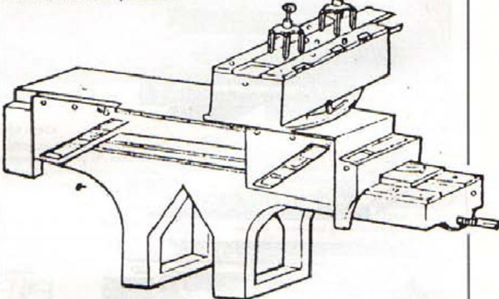
Fig. 12: This is Maudslay's slide rest, nick-named "Maudslay's Go-cart".
