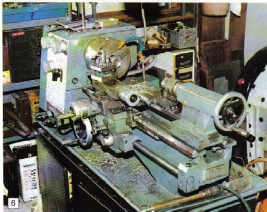
6: The Excel lathe.
