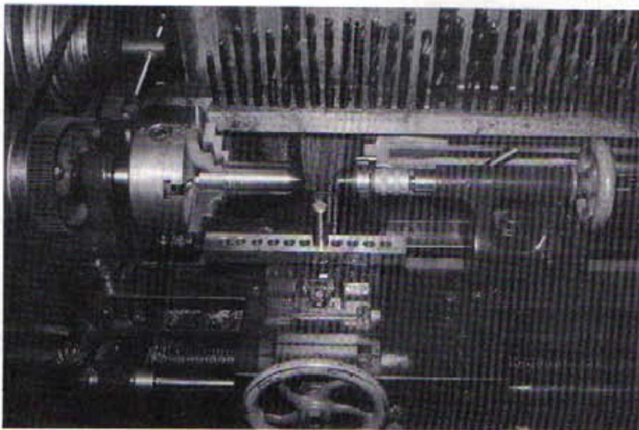
The lathe, seen here set up for metal spinning.
