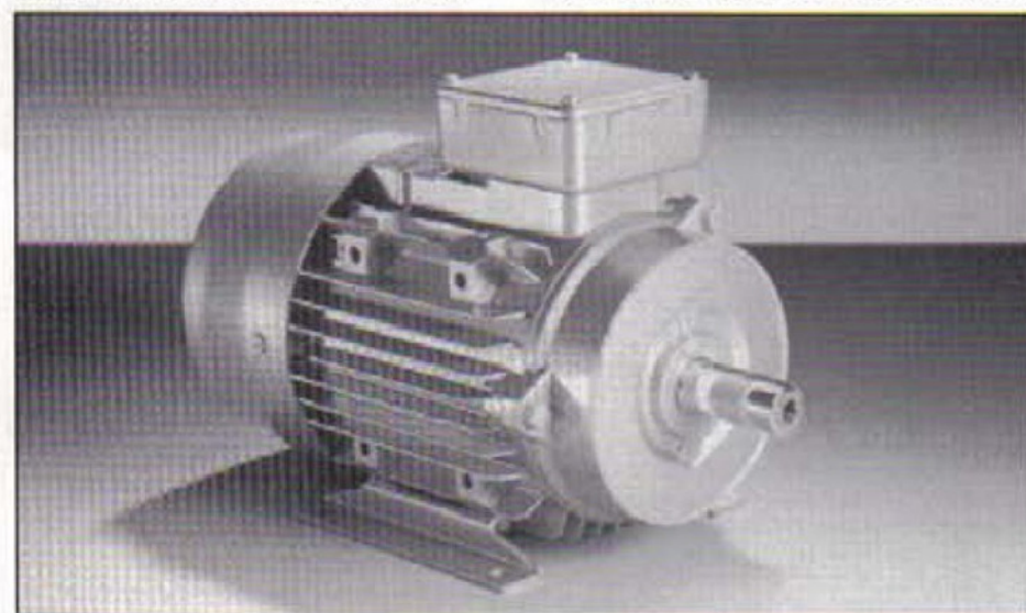
Photo 3: A modern Brook Crompton aluminium frame motor having multi mount facilities. These are available from 0.07KW up to 37KW three phase. Similar single phase motors are available but covering only the lower end of the power range.
