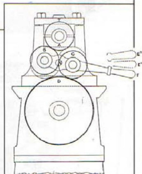
Fig. 13: James Nasmyth's tumbler reverse for the lathe traverse, 1837. (James Nasmyth, Autobiography, 1883).
