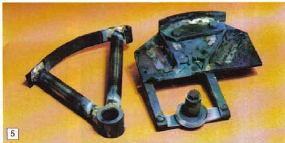
5: A replacement roll over stand in the course of construction together with its welding/brazing jig.
