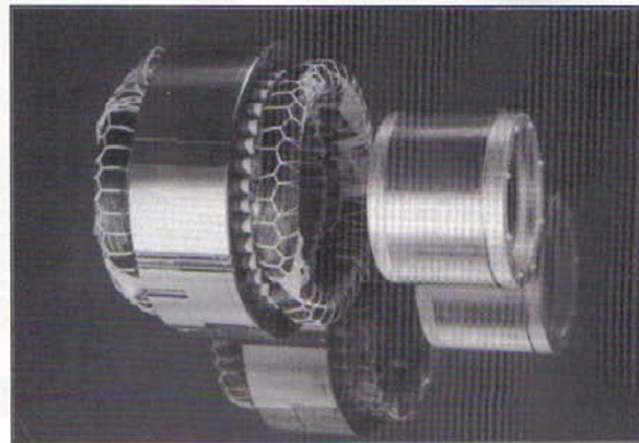
Photo 2: The two main parts of a three phase motor, showing the simple construction of the rotor.
