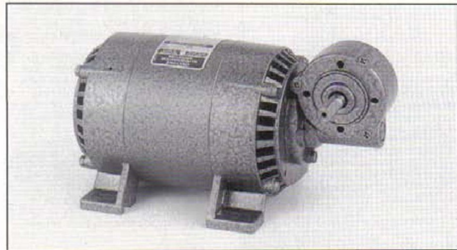
Photo 4: A small Parvalux motor with output gearbox, available for single or three phase supply. Output power is up to 120W, speed is either 1400 or 2800 rpm without a gearbox. Speeds from 35 up to 680 rpm are available with differing gearboxes. This is typical of the very wide range of small AC and DC motors supplied by this company.
