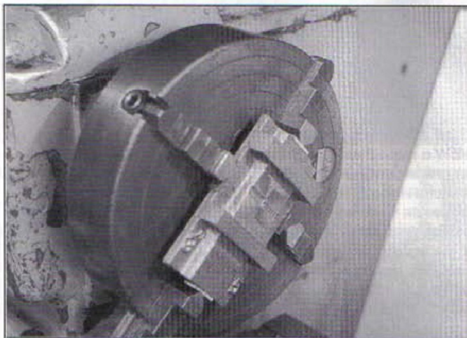
4: The slide faced for the 5 in. square plate.
