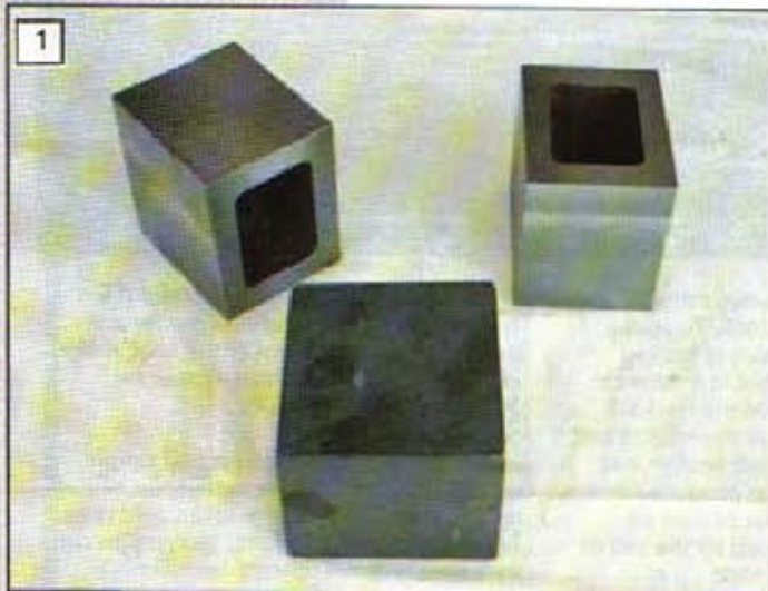
1: Shows two box angle plates partly machined with the wooden pattern in the foreground.
