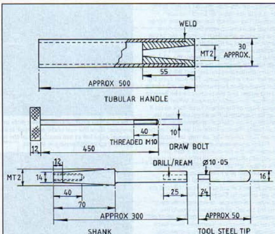
FIG. 5 COMPONENT PARTS FOR SPINNING TOOLS
