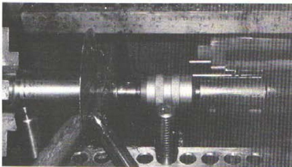
The next four photographs show a little of the sequence of operations in the spinning process. Note the use of the backstick in the first; the partly spun dome in the second; the ragged edge left at the conclusion of the forming operation in the third, and the end result prettied up and gleaming in the last.
