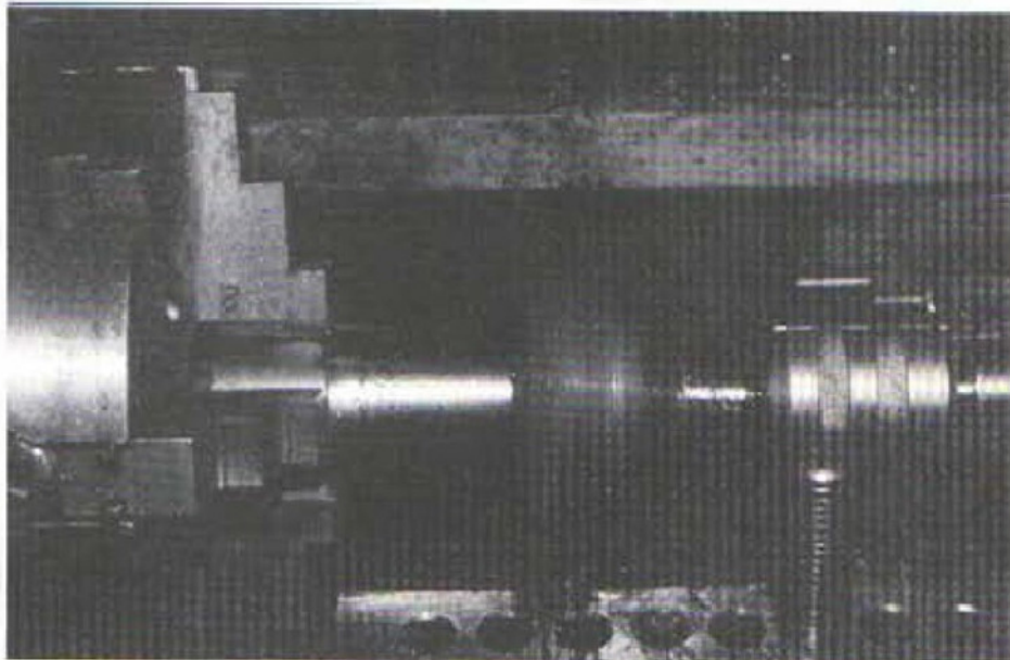
The next four photographs show a little of the sequence of operations in the spinning process. Note the use of the backstick in the first; the partly spun dome in the second; the ragged edge left at the conclusion of the forming operation in the third, and the end result prettied up and gleaming in the last.
