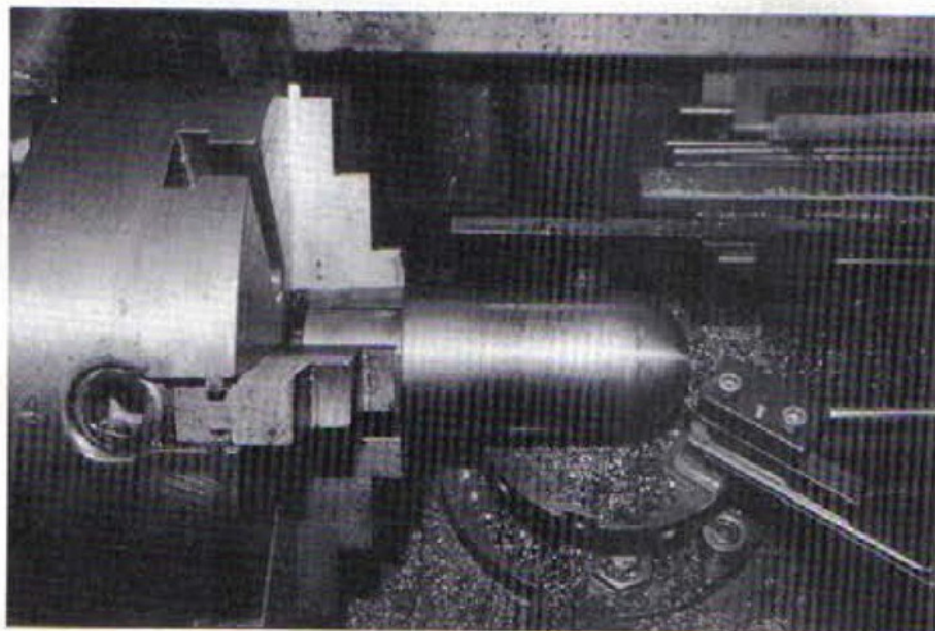
As can be seen in this photograph a ball turning attachment cones in very handy when making the formers.
