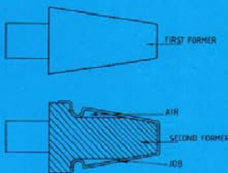
FIG. 10: SPINNING IN AIR
