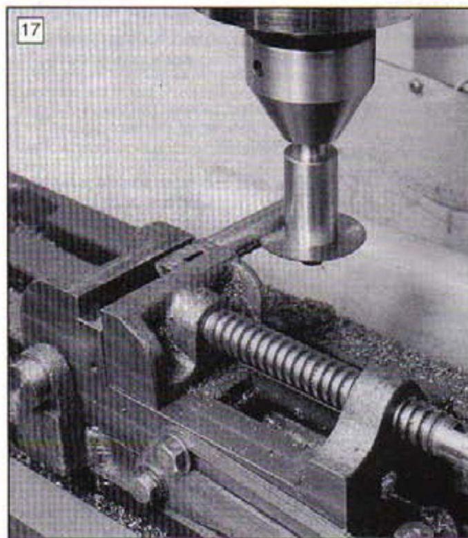
17: Slotting the toolmakers clamps. Note the use of the small Vee block to assist with holding the part securely.
