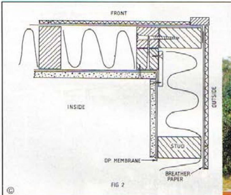
Frame detail.
