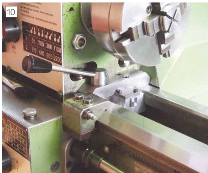
Clutch control lever.
