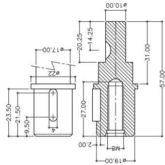
Output Shaft Mat'l: 01 tool steel
