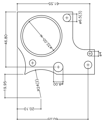
Output Bearing Cover Mat'l: Aluminium
