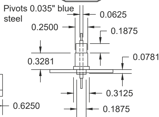
Minute wheels 39t, 0.75 module, O.D. 1.233, 1/16" thick Pinion 6t, 0.75 module, O.D. 0.228
