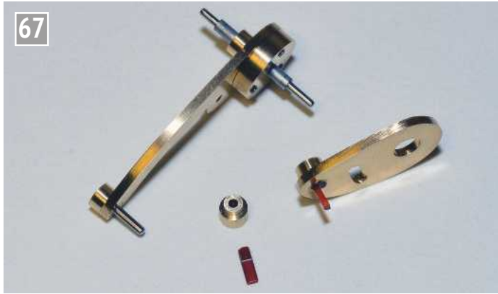
The remontoire release arms.
