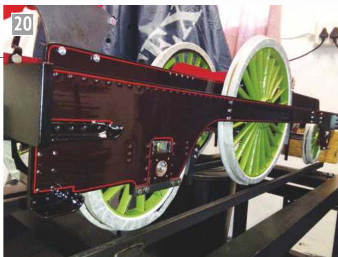
Stirling frame lining (the masking tape on the wheels is for assembly).
