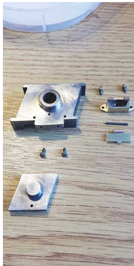
19. Here is a view of the various parts that make up the springplate assembly for the Cartazzi axle. The lower item is the wedge - you can clearly see the oilway hole, which is off centre - above is the two 10BA bolts that would hold on the dust shield if fitted - this seems to be a later item and I haven't seen the shield itself on pictures from the era I'm modelling, although the bolts are seen. Next up was to bolt the tank to the spring plate and then drill the oilway hole, this being drilled at an angle through from the oil tank, through the spring plate and then also through the sideways control wedge.
