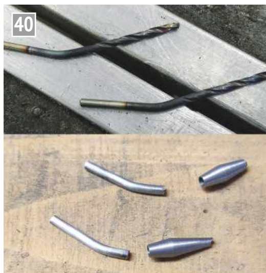
A novel way of making the handles.
