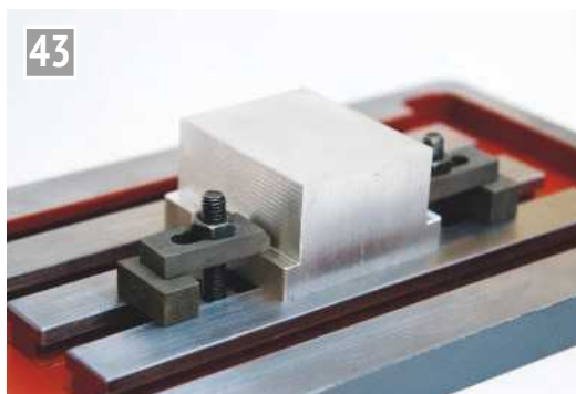
Test piece held down with home-made clamps.
