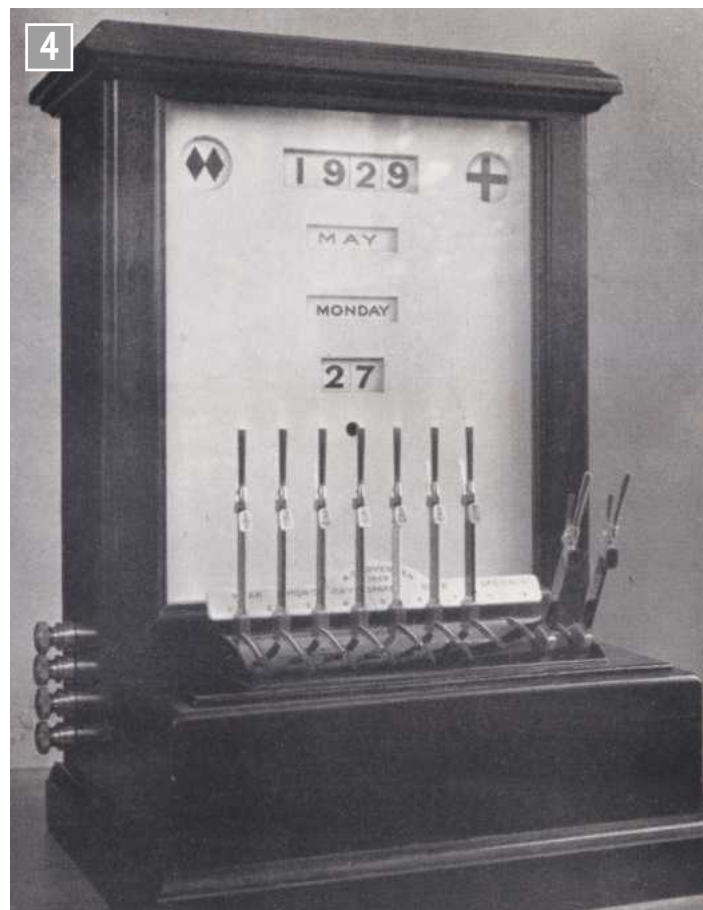
Interlocking calendar from Brighton & Hove SMLE (photos thought to be by Dr John Bradbury Winter).
