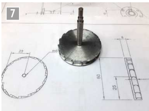
Rotor with all buckets machined.
