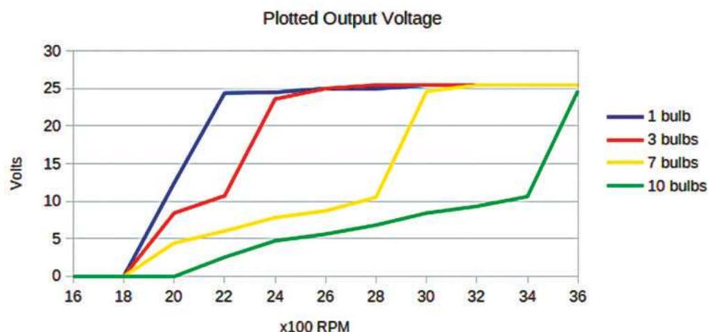
Fig 18 Engine Alternator Rig - AutoTest Results
