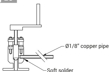
Part 77: Regulator Assembly
