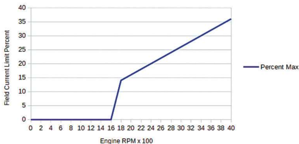
Fig 17 Lookup Table used in AutoTest
