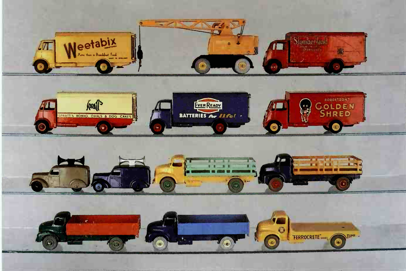
Row 1. 514 Weetabix Van, 571/971 Coles Mobile Crane, 514 Slumberland Van. Row 2. 514/917 Spratts Van, 918 Ever Ready Van, 919 Golden Shred Van. Row 3. 34c/492 Loudspeaker Van (x2), 531/417 Leyland Comet (x2). Row 4. 532/418 Leyland Comet (x2), 533/419 Leyland Cement Truck.
