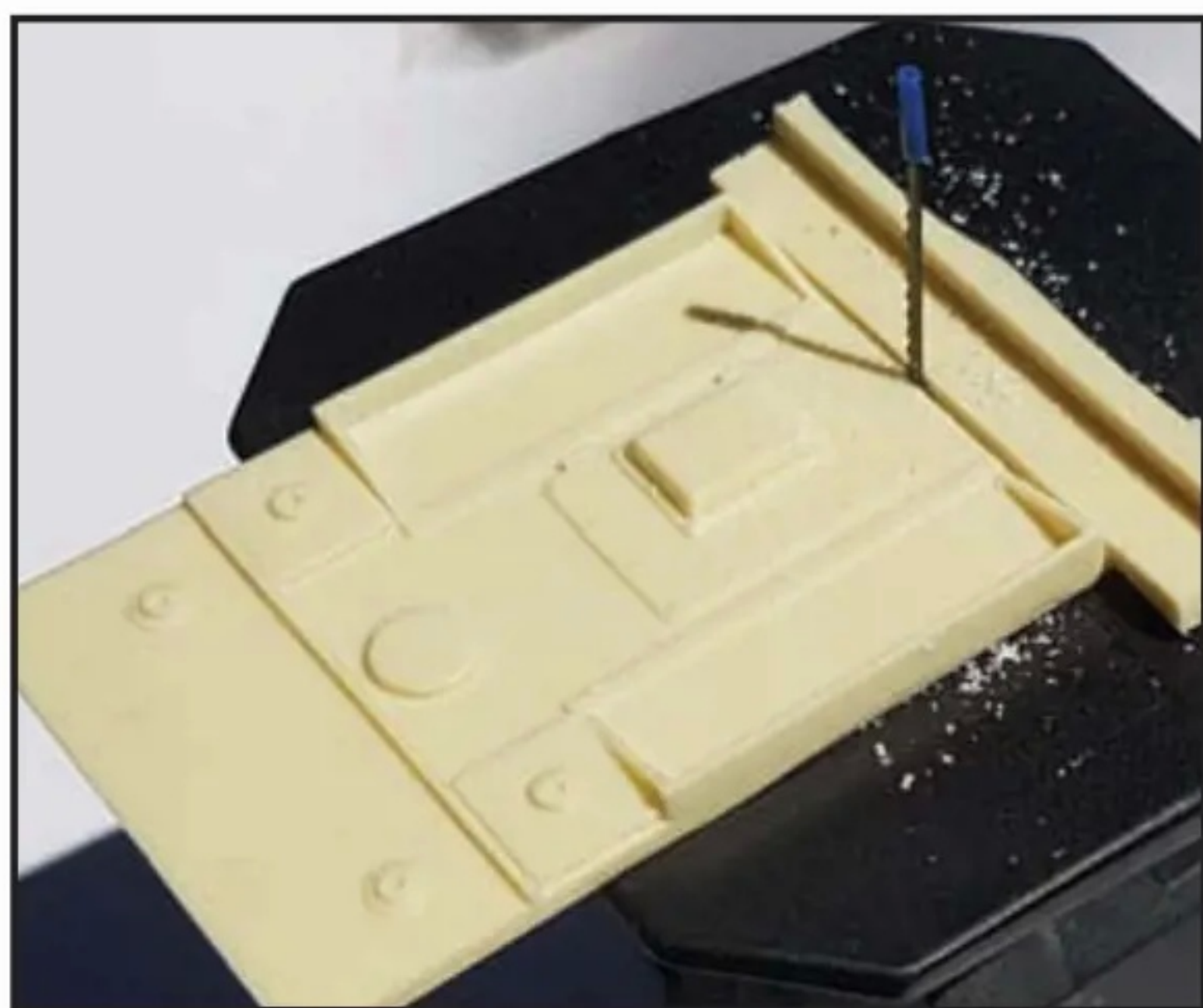
For separating less fragile resin parts from the huge casting block I used a mini-scroll saw.
