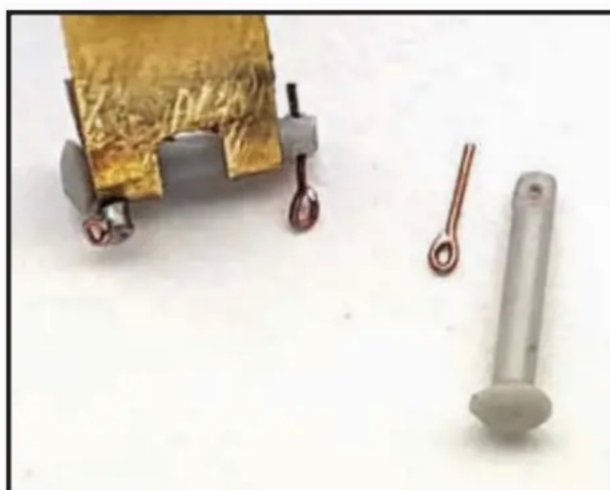
The travel lock fixing device consists of a tightening metal strap secured with 2 bolts. A heated screwdriver held close at one of the plastic rod ends created half-round bolt head. Then I modified thin wire as the cotter pins and glued a little eye for securing chain.
