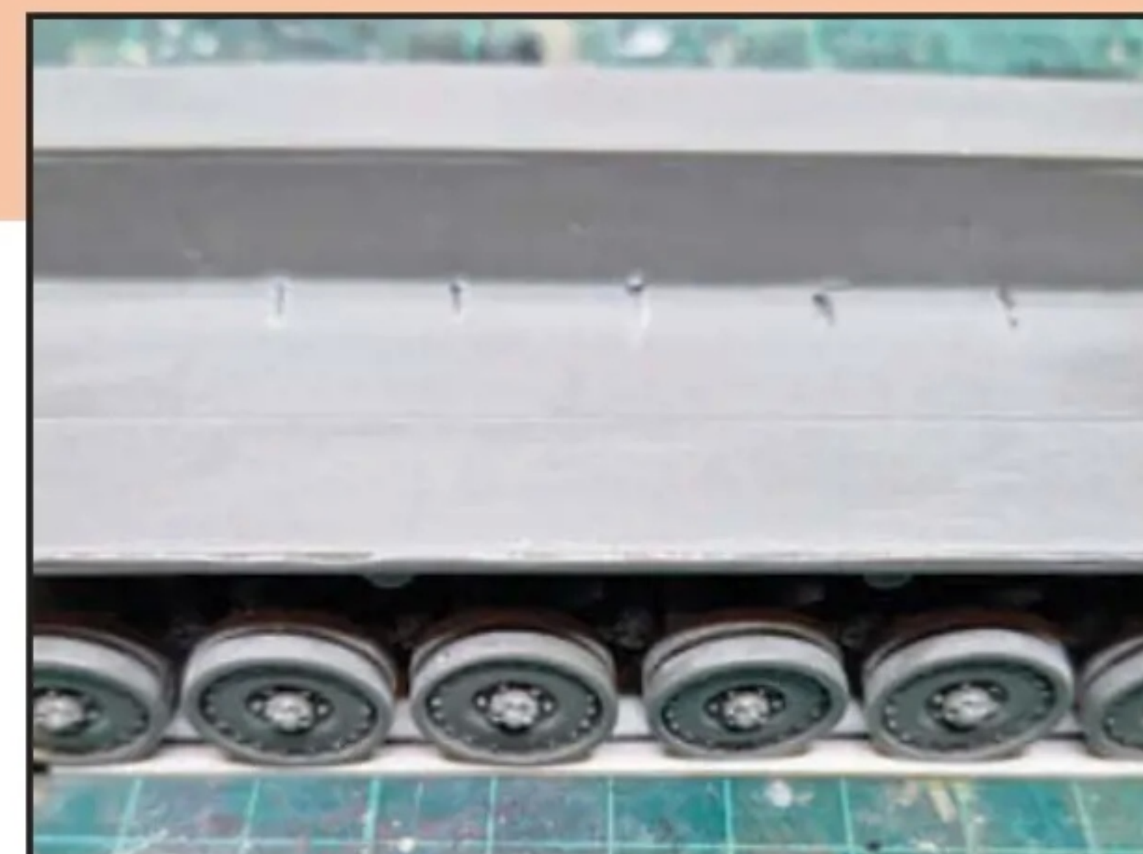
The jig was fitted with a metal rod to ensure the correct alignment of the wheels
