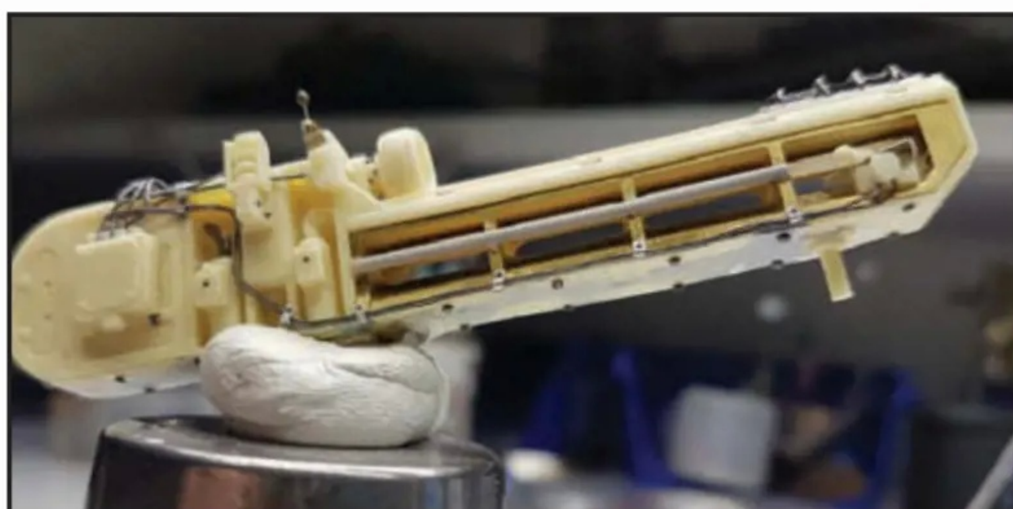
Very simplified loading mechanism was improved by adding a lot of new elements for which the lead wire proved to be quite appropriate.
