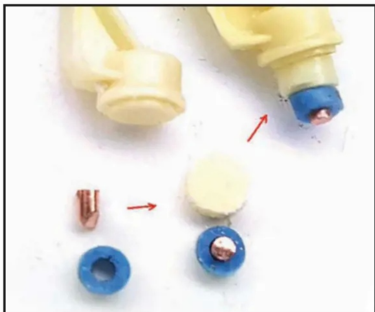
Buffer parts of the shock absorbers were improved adding a little resin cylinder with electrical wire and its jacket.
