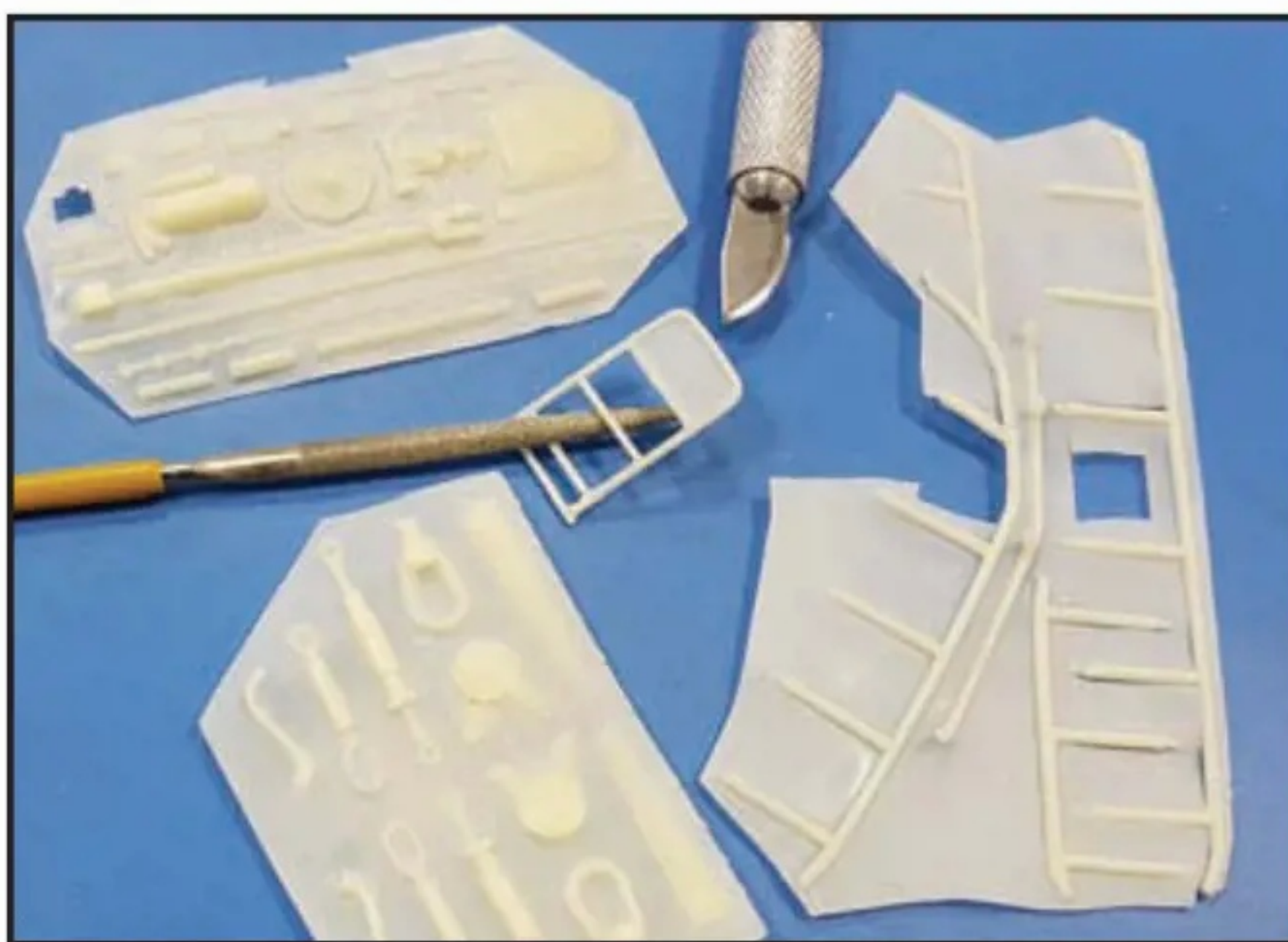
The most fragile resin parts were released with a brand new half-round scalpel, of course immediately after they had been heated gently to make the resin less brittle. Tricky job demanding a great deal of patience
