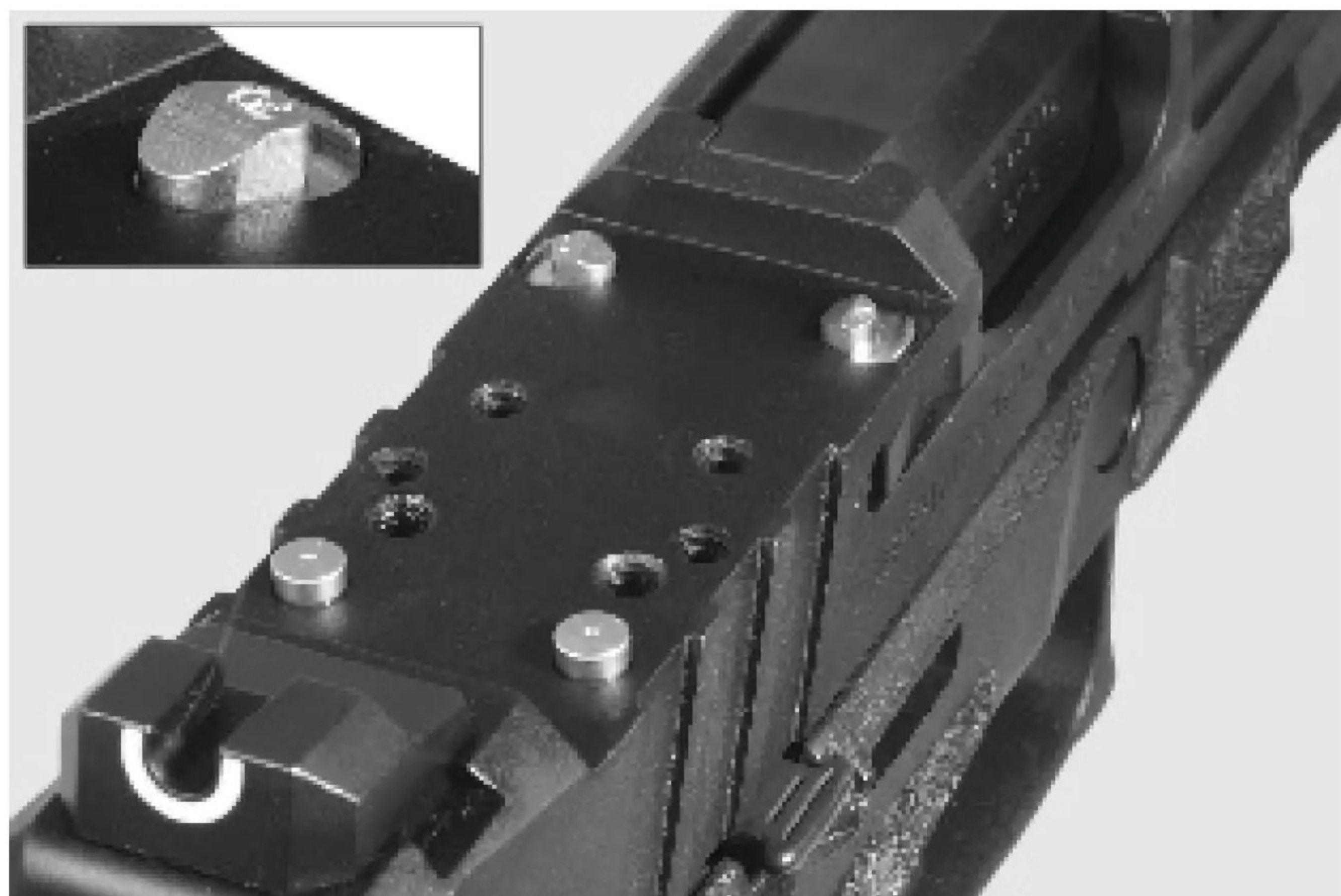
▲ The VIS's pin system allows a direct mount of more than 30 red dots. The angled front pin design (inset) dramatically reduces potential zero shifts.
