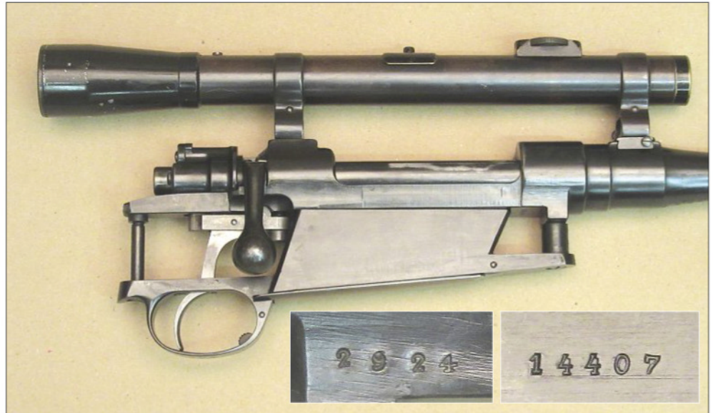
Rifle no. 2 action with slanted magazine box and step-down receiver ring. Rigby number 2924 and Mauser number 14407. Original Rigby telescope in factory quick-release mounts with front locking lever.
