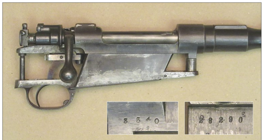
Rifle no. 3 action with slanted magazine box and step-down receiver ring. Rigby number 3540 and Mauser number 28290.
