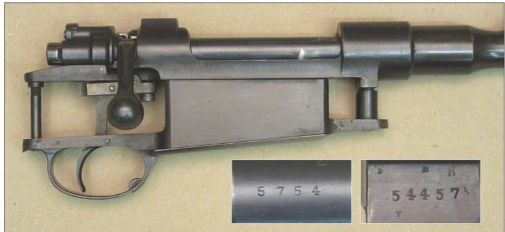
Rifle No. 4 Magnum action with normal magazine box and receiver ring. Rigby number 5754 and Mauser number 54457.
