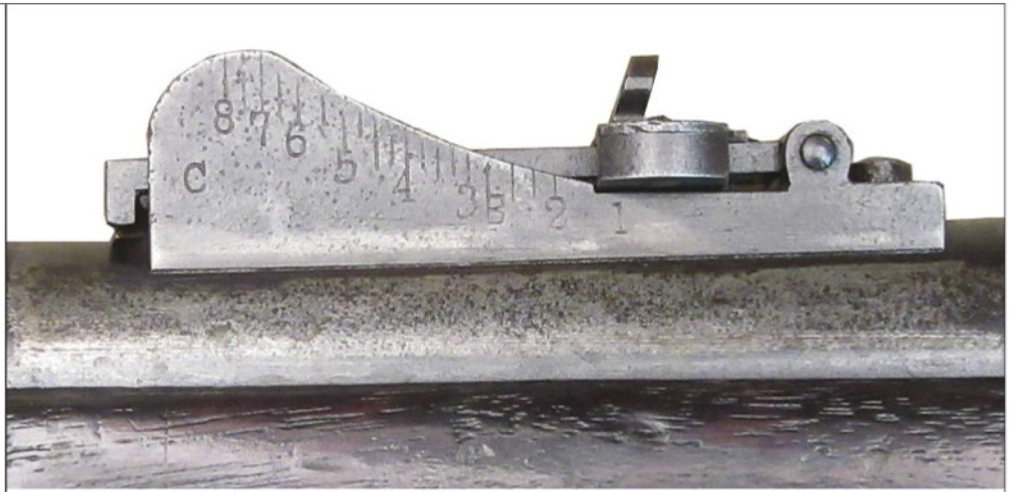
LEFT AND ABOVE: The early rear sight found on the carbine. Note the “C” stamped into the top left of the ladder and on the left side.
