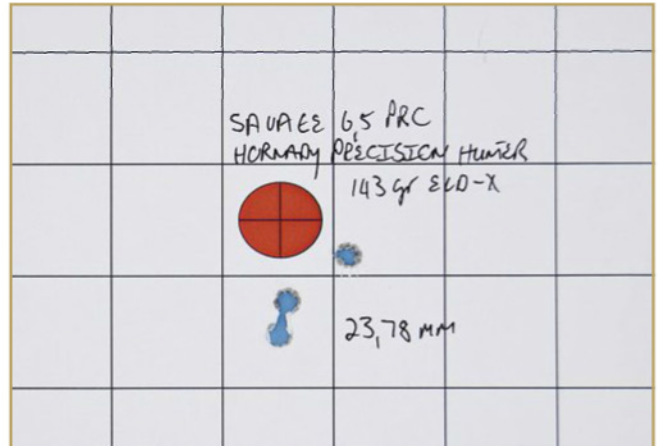
The group achieved with the Precision Hunter ammunition – 23,78 mm or 0.817 of a MOA – very good by anyone's standard and far better than most out-of-the-box factory rifle/ammo combinations are capable of.
