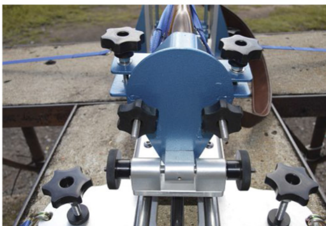
A view from the rear of the RCBB showing the different adjustment controls and clamps.
