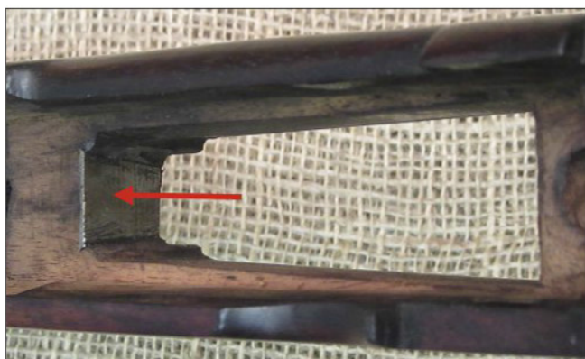
Steel plate inlet into stock to provide front wall for extended magazine box.
