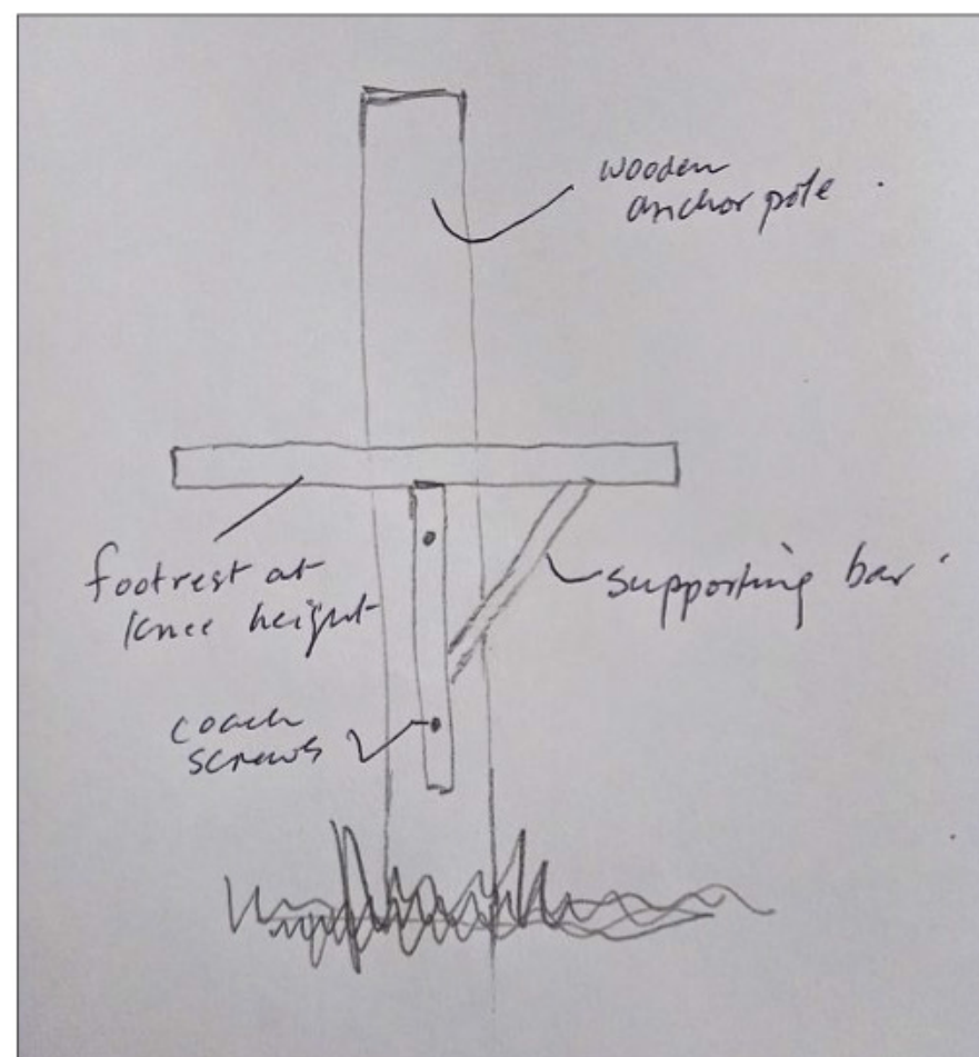
A technical drawing of the "T-step".
