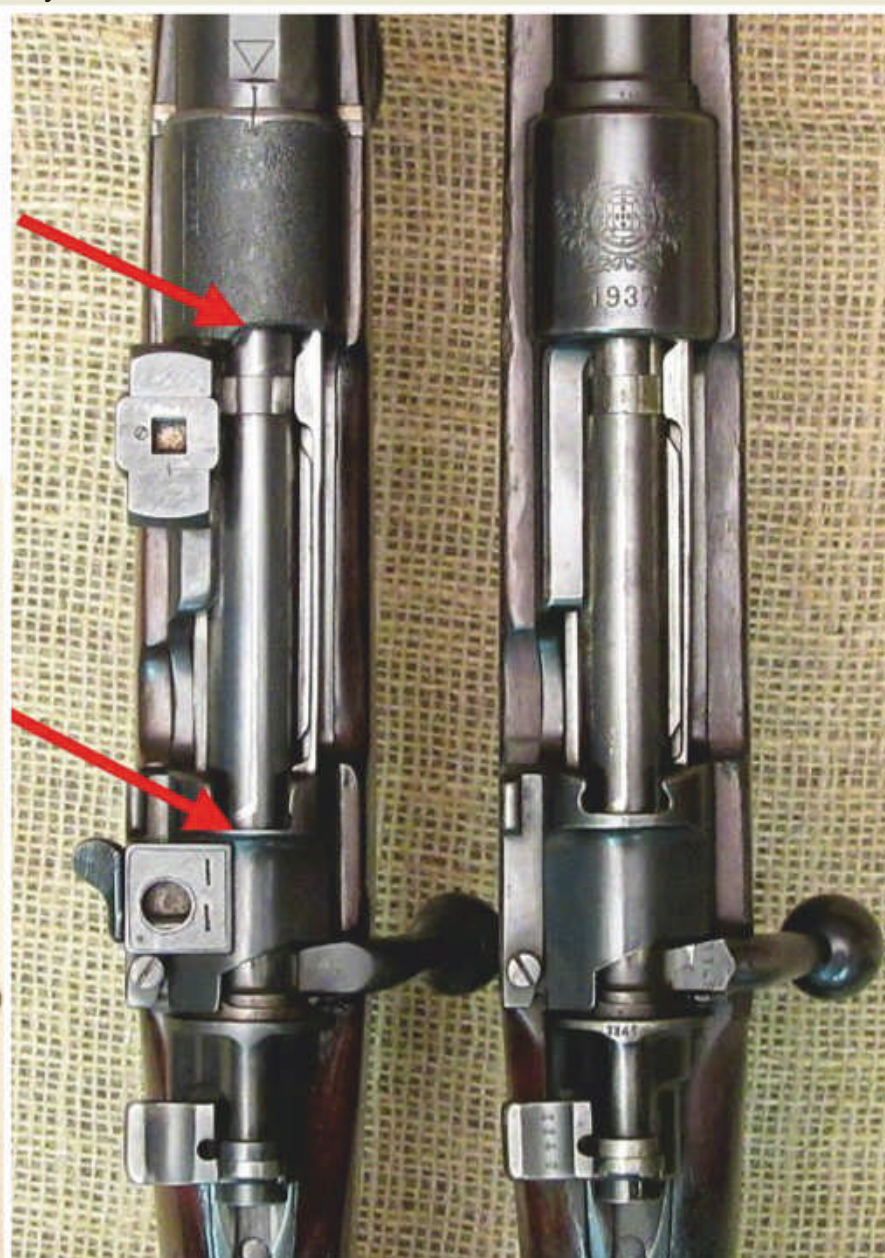
.318 Westley Richards on the left and military M98 8x57 mm on the right. Notice how the receiver ring has been moved forward and the stripper clip notch moved backwards.
