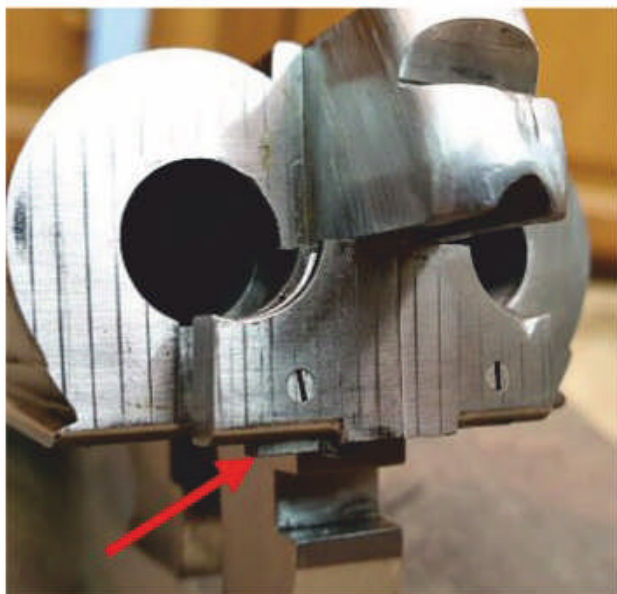
Rimless extractor plate in the down position with small tab protruding at the bottom as indicated.
