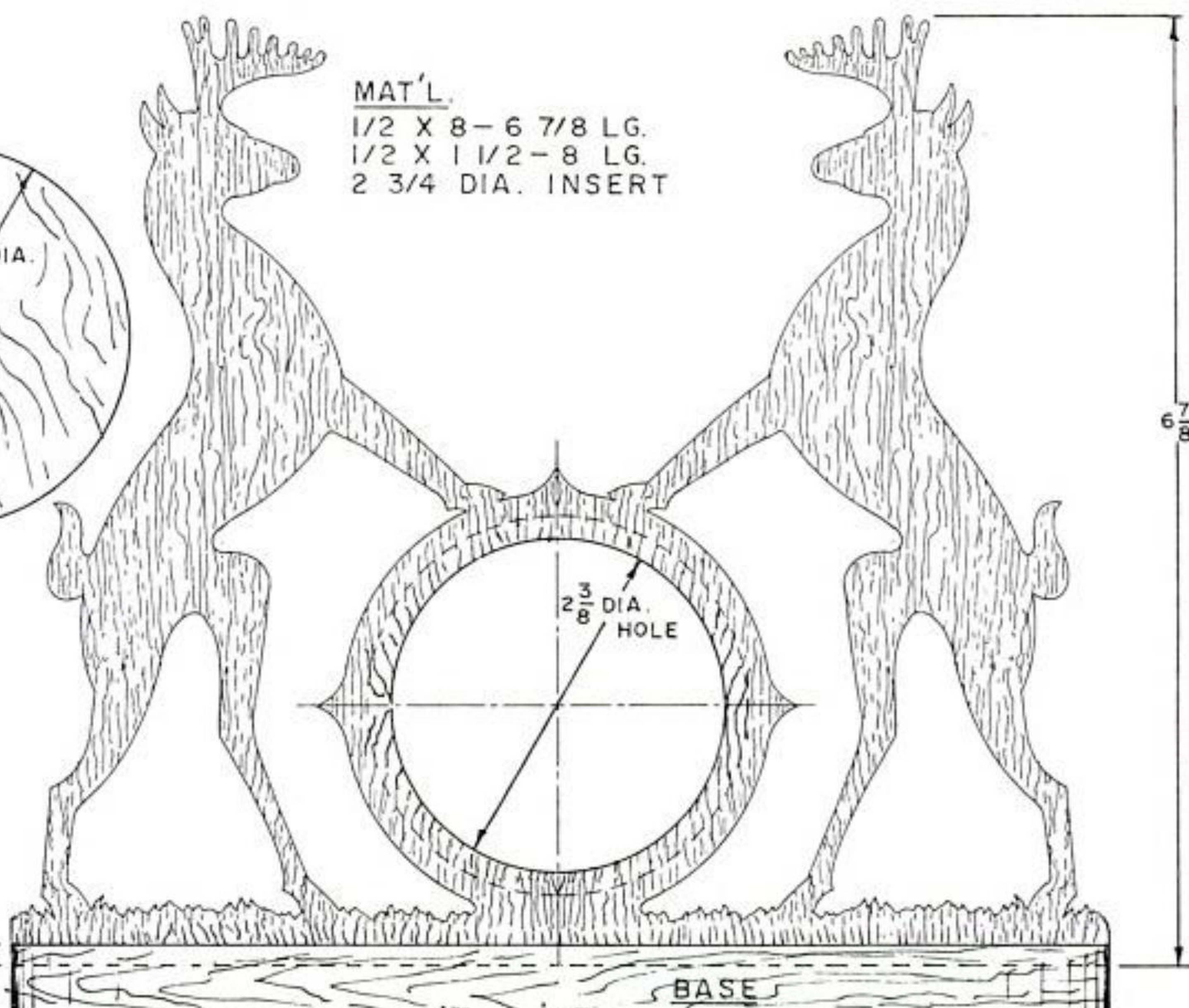
FRONT VIEW
