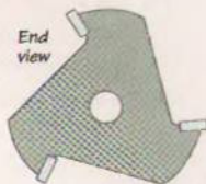
Slot-and-arbor cutter; also known as three-wing slotting cutter
