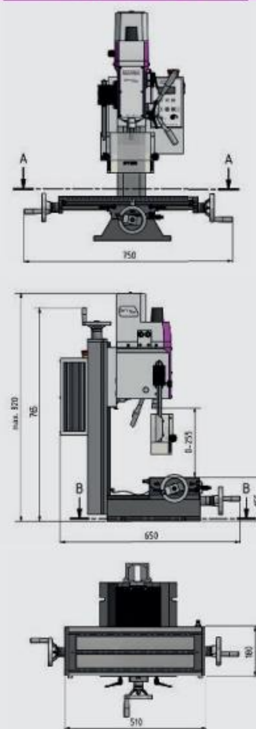
Dimensions MH 20V
