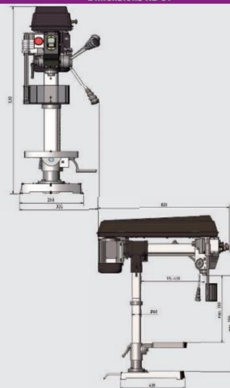
Dimensions RB 6T
