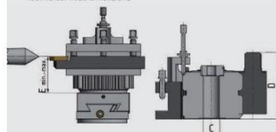
Tool holder head dimensions
