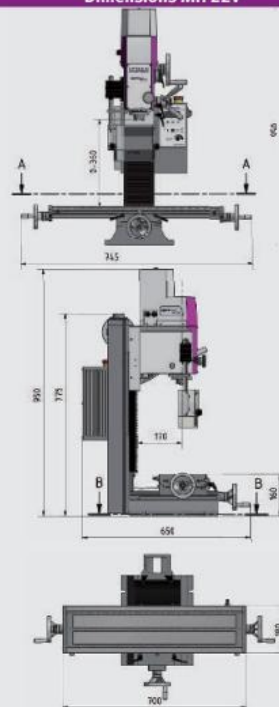
Dimensions MH 22V
