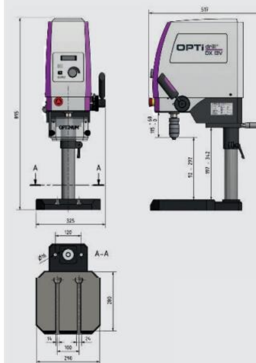
Dimensions DX 13V
