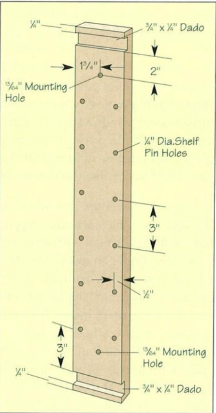
Side Panel Layout
