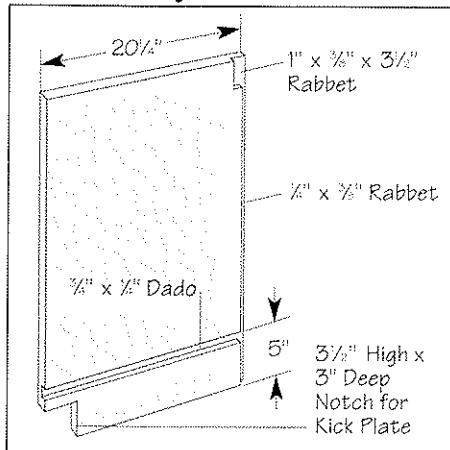
Partition Layout
