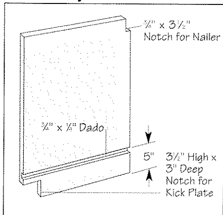
Partition Layout
