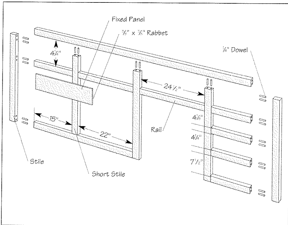
Face Frame Construction
