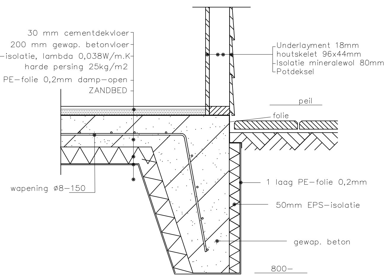
DETAIL FUNDERING
