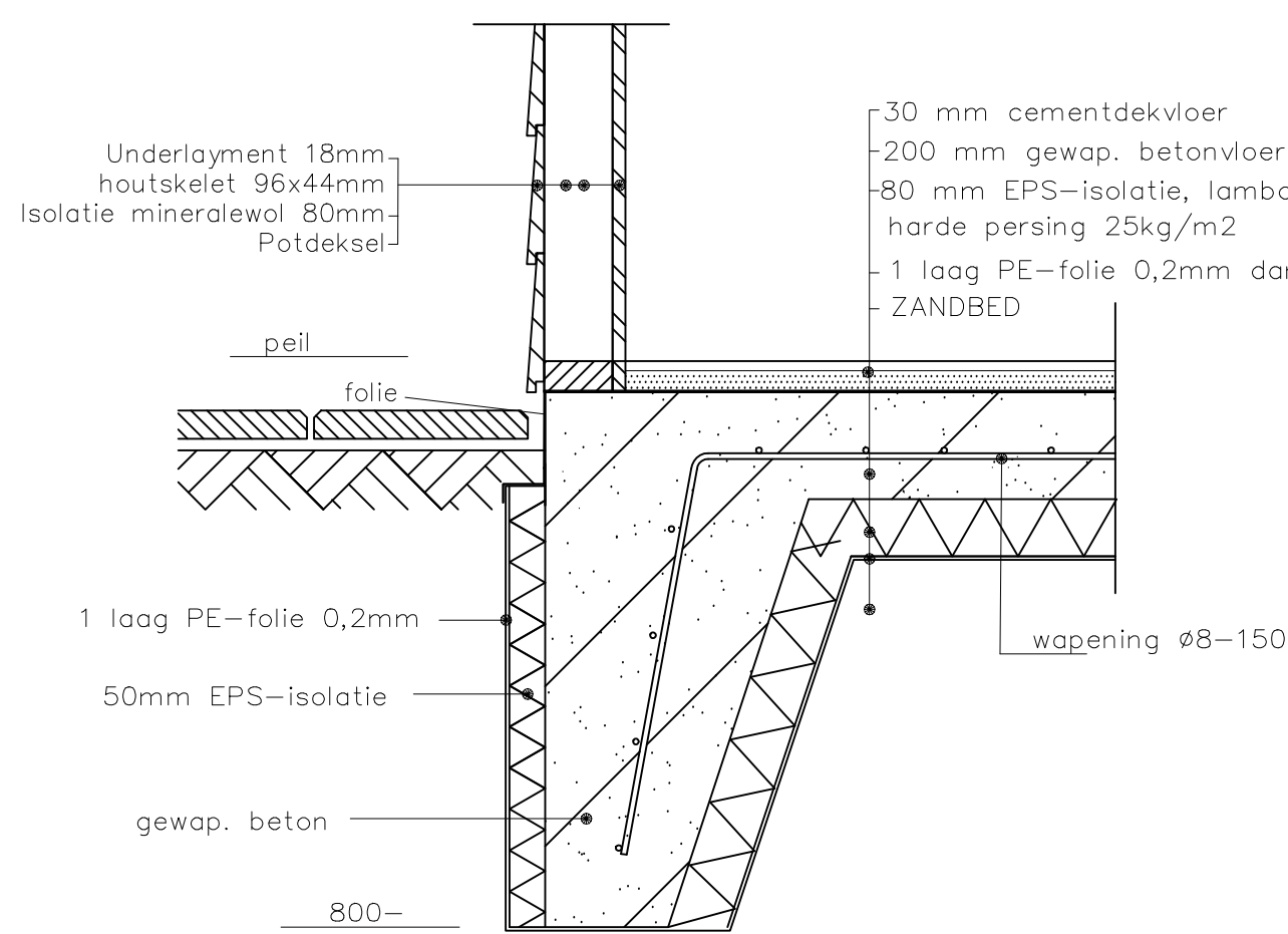
DETAIL FUNDERING
