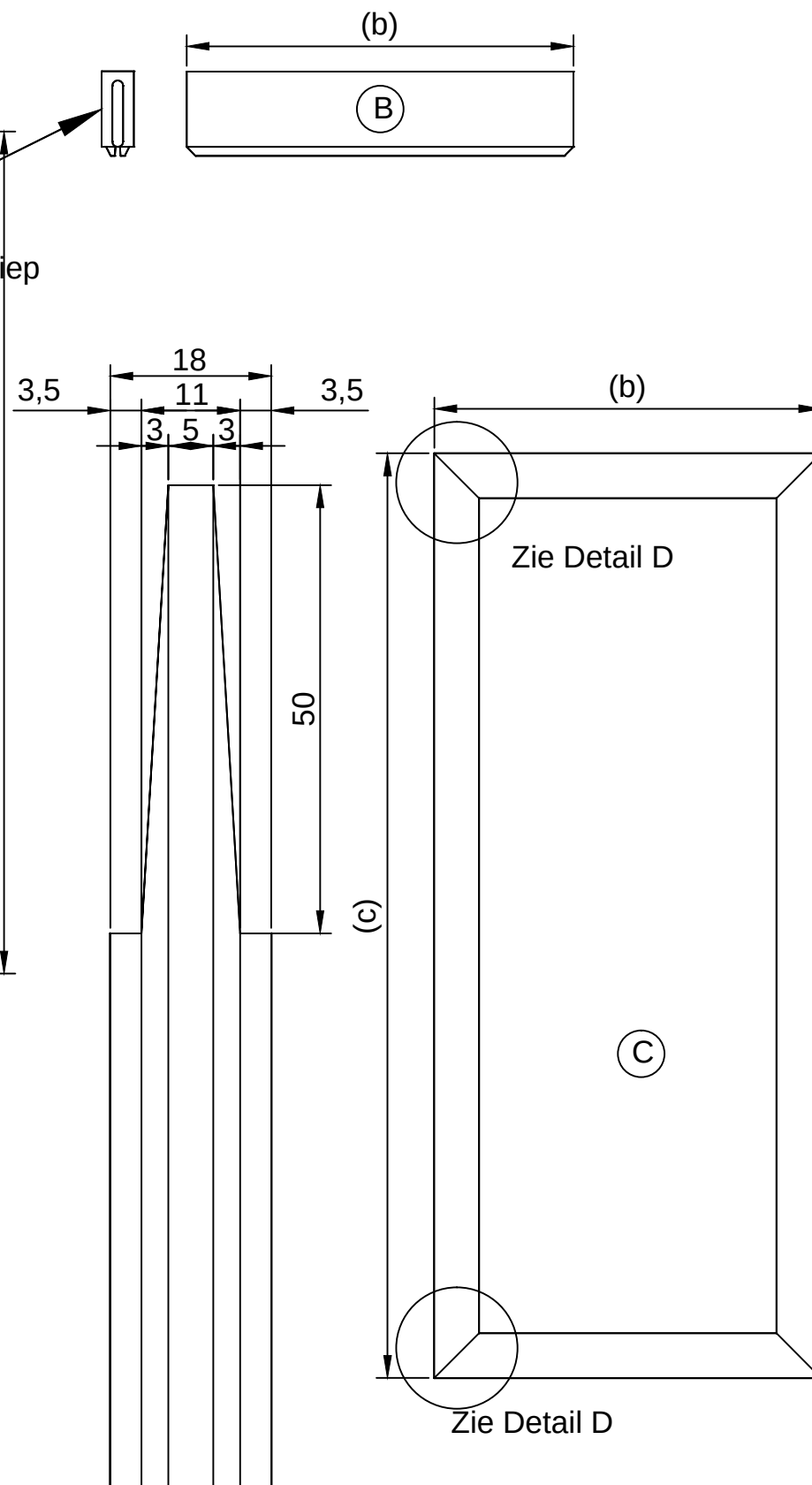
Detail D
