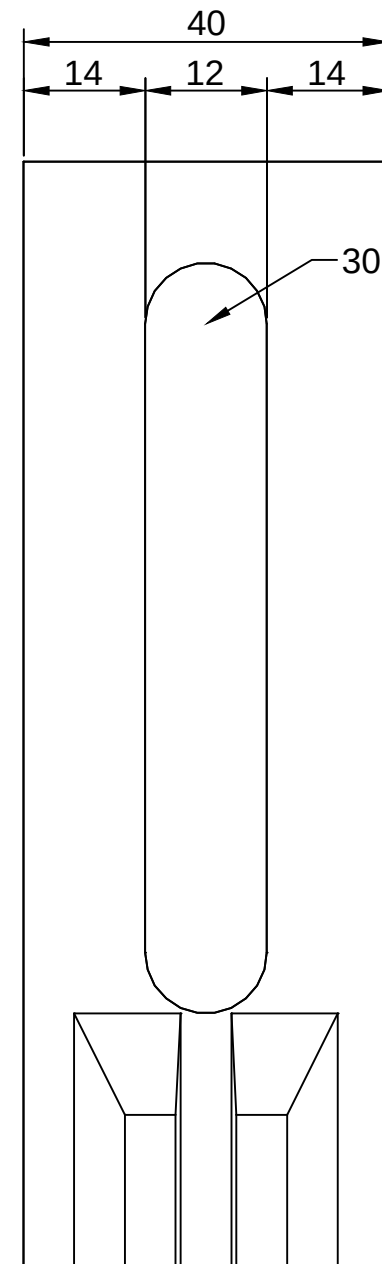
Detail B
