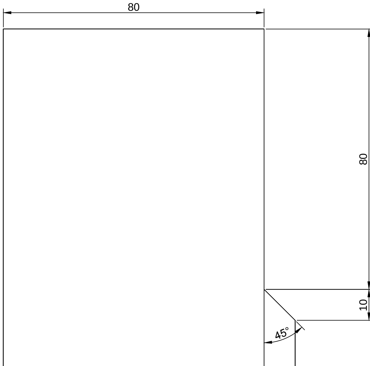
Detail A
