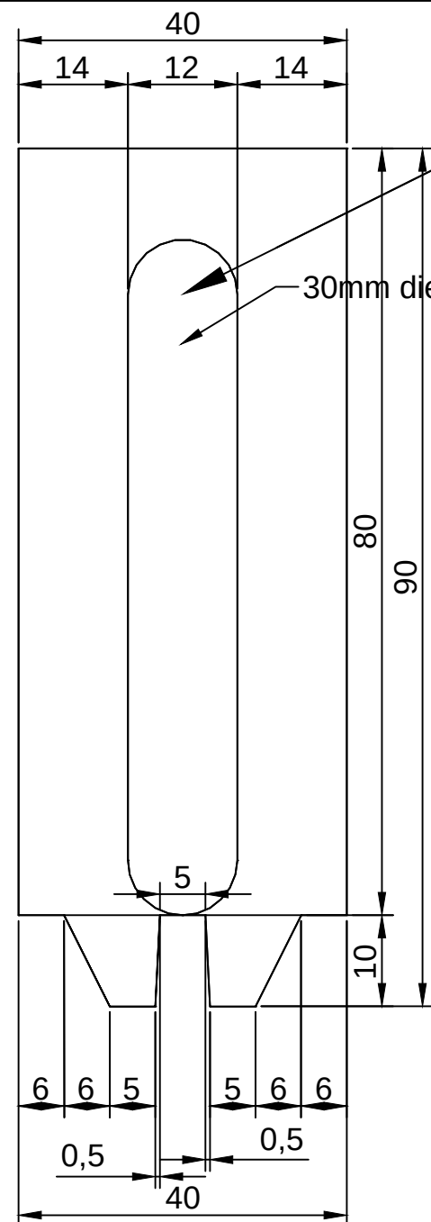
Detail C
