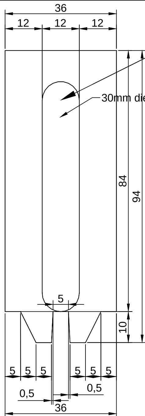
Detail C
