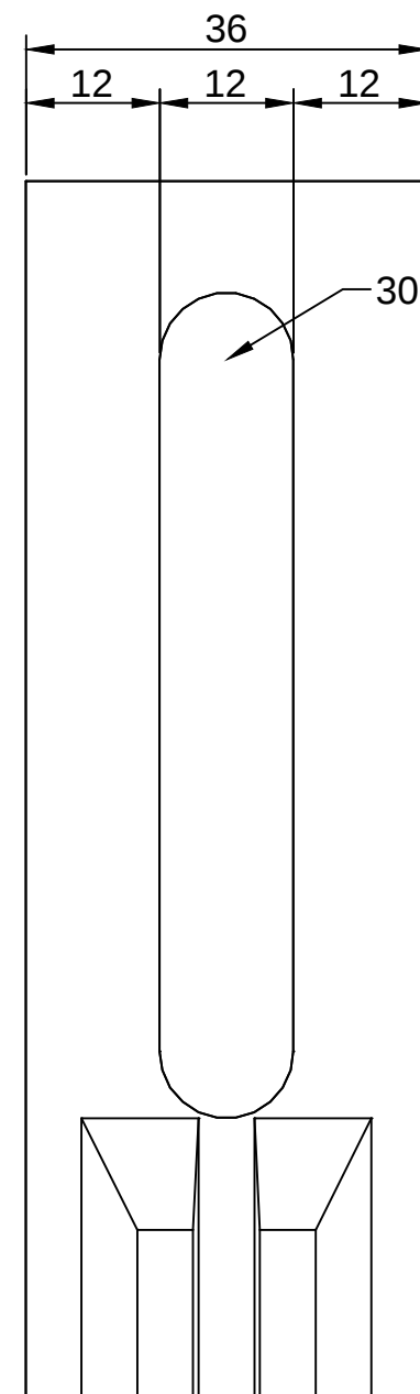
Detail B
