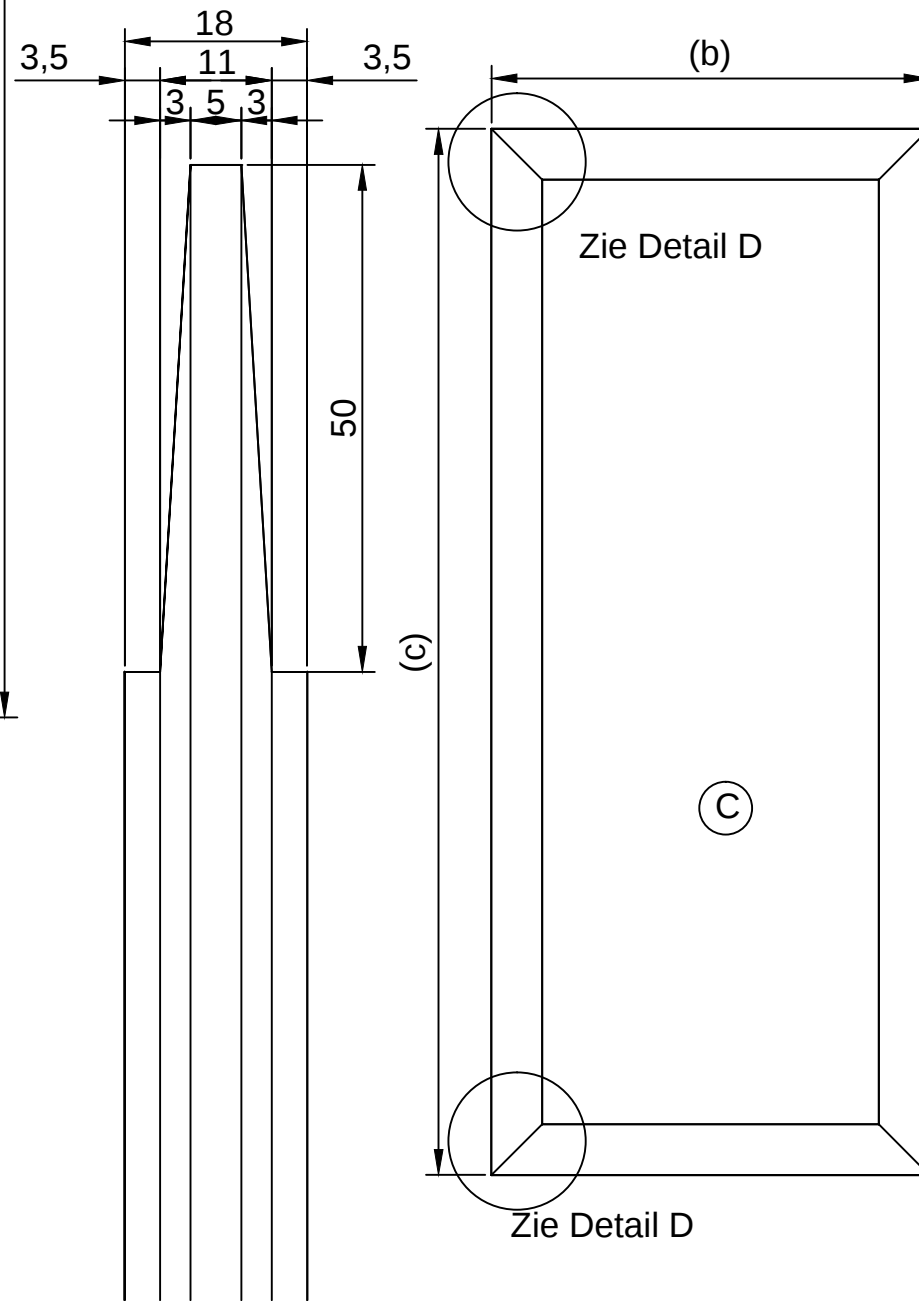
Detail D
