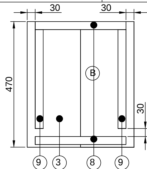
B = TUSSENWAND
